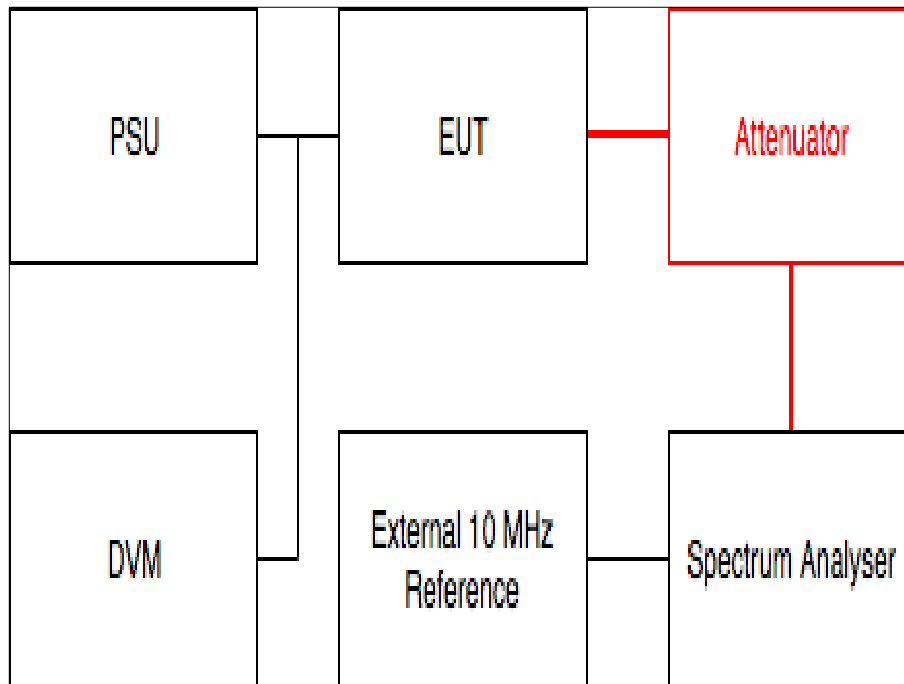
Figure 1 - Conducted Tests
