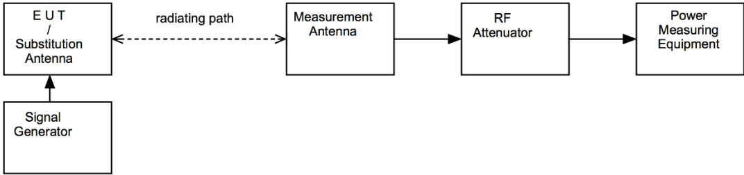
Figure vii Test Setup
