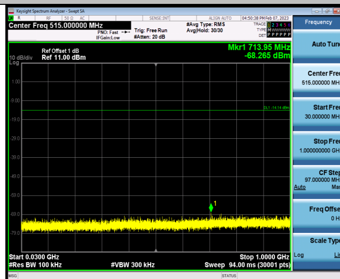
Mode1_2437_30~1000
