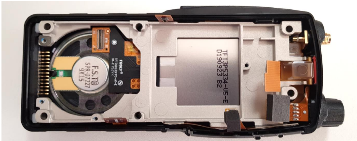
Figure 9. XX6SC2028 LCD Side
