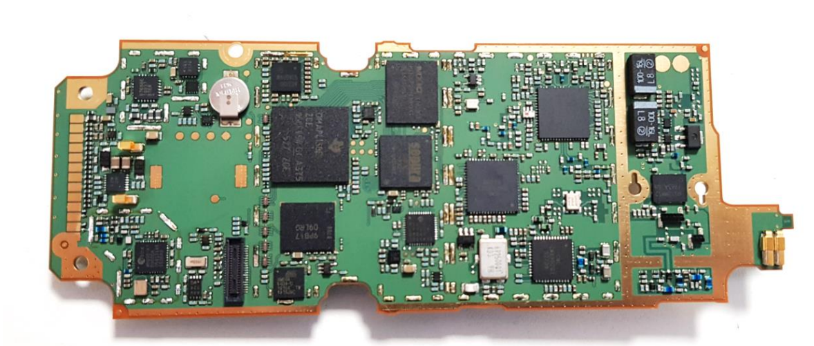
Figure 8. XX6SC2028 Main PCB Bottom View with Cans Removed
