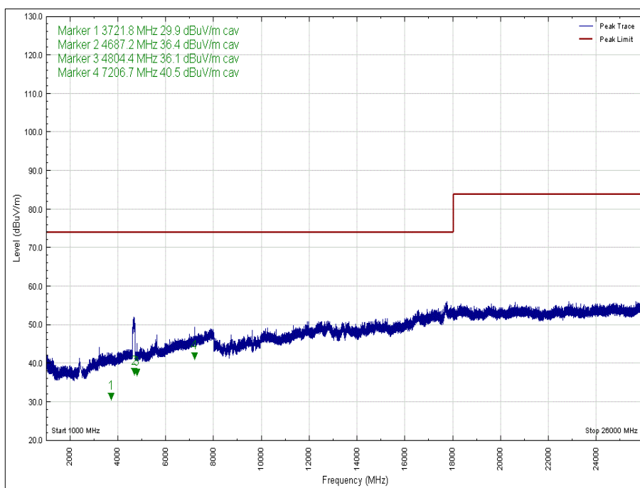
Figure 14 - 2402 MHz - 1 GHz to 26 GHz, Polarity: Horizontal, EUT Orientation: X, Peak
