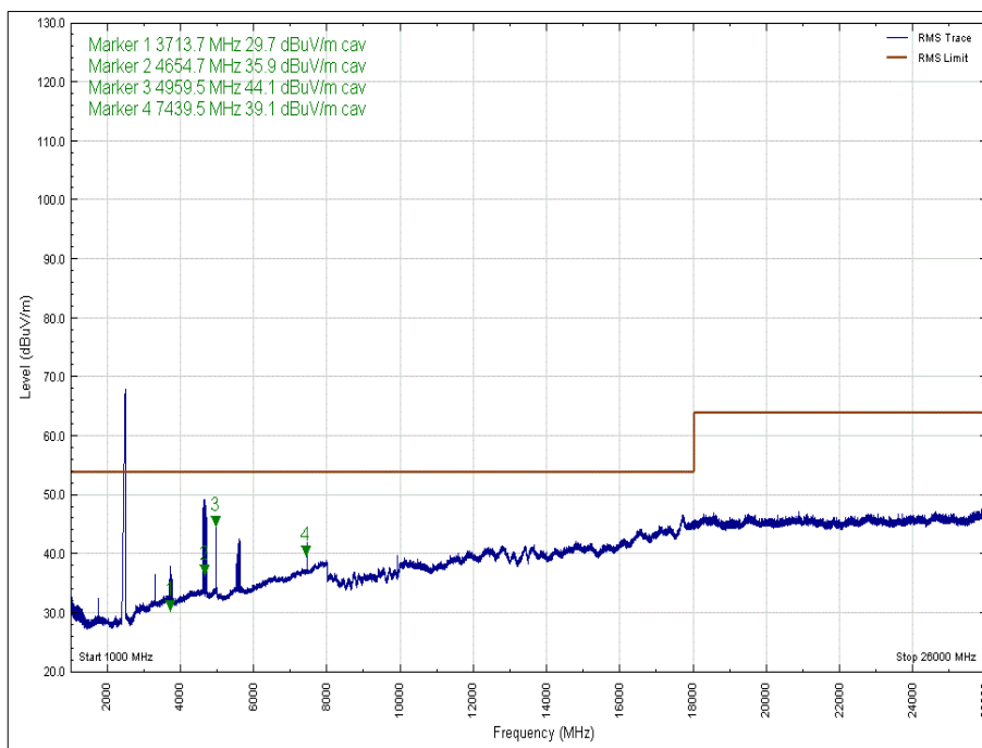
Figure 52 - 2480 MHz - 1 GHz to 26 GHz, Polarity: Horizontal, EUT Orientation: X, Average
