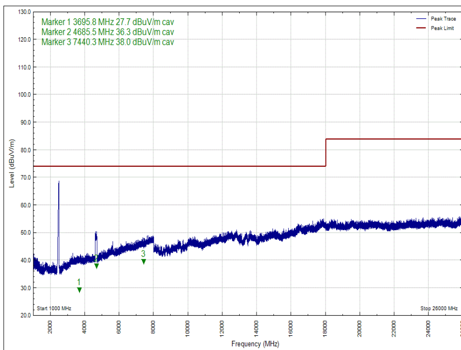
Figure 53 - 2480 MHz - 1 GHz to 26 GHz, Polarity: Vertical, EUT Orientation: Y, Peak
