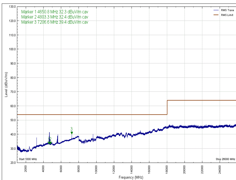
Figure 15 - 2402 MHz - 1 GHz to 26 GHz, Polarity: Vertical, EUT Orientation: X, Average
