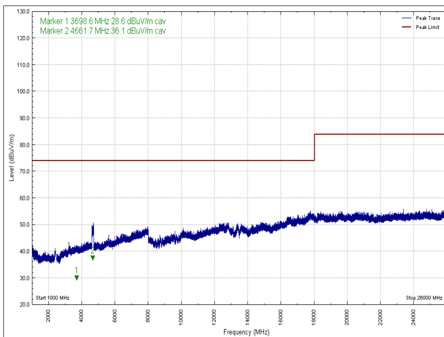
Figure 17 - 2402 MHz - 1 GHz to 26 GHz, Polarity: Vertical, EUT Orientation: Y, Peak
