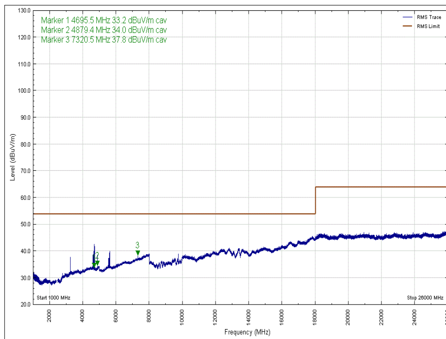
Figure 33 - 2441 MHz - 1 GHz to 26 GHz, Polarity: Vertical, EUT Orientation: X, Average
