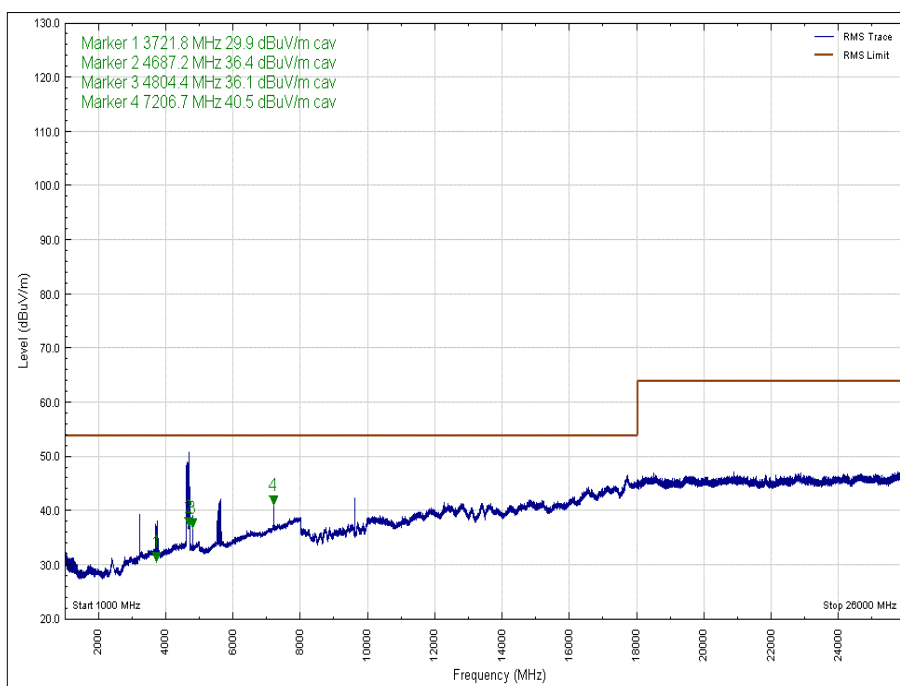
Figure 16 - 2402 MHz - 1 GHz to 26 GHz, Polarity: Horizontal, EUT Orientation: X, Average
