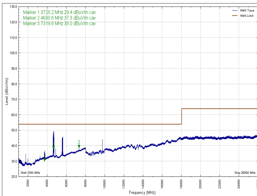
Figure 54 - 2441 MHz - 1 GHz to 26 GHz, Polarity: Vertical, EUT Orientation: Z, Average
