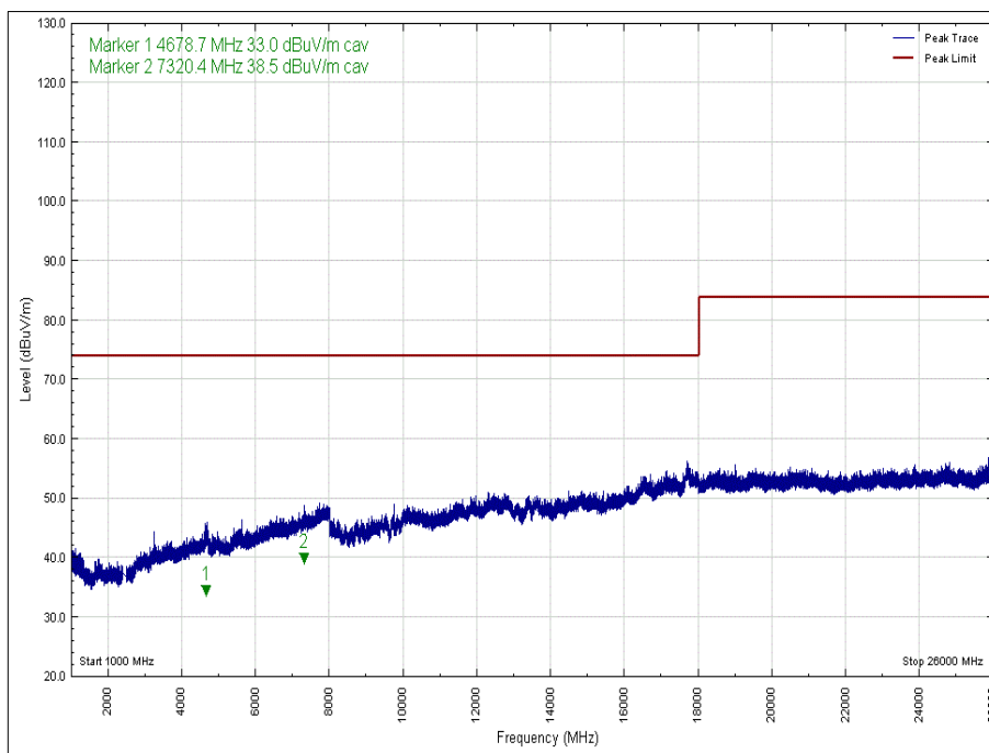
Figure 53 - 2441 MHz - 1 GHz to 26 GHz, Polarity: Horizontal, EUT Orientation: Z, Peak
