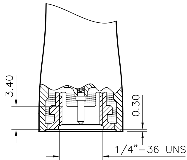
ENLARGED DETAIL OF TERMINAL END
