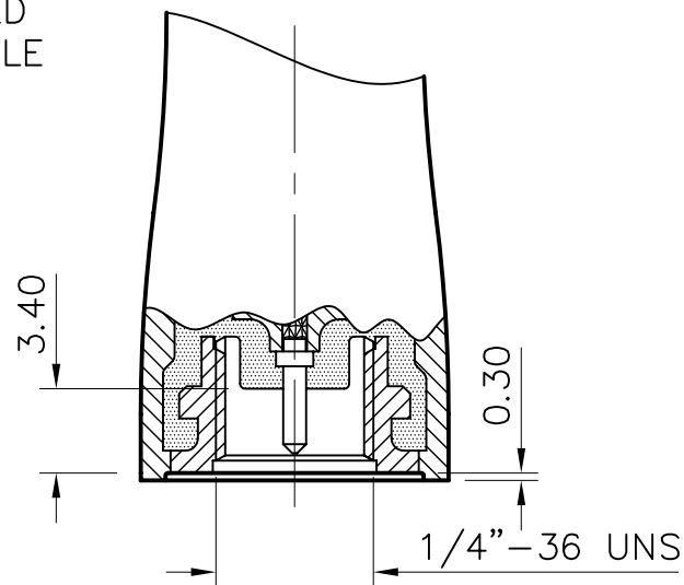
ENLARGED DETAIL OF TERMINAL END
