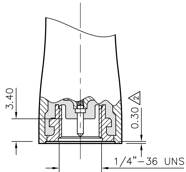
ENLARGED DETAIL OF TERMINAL END
