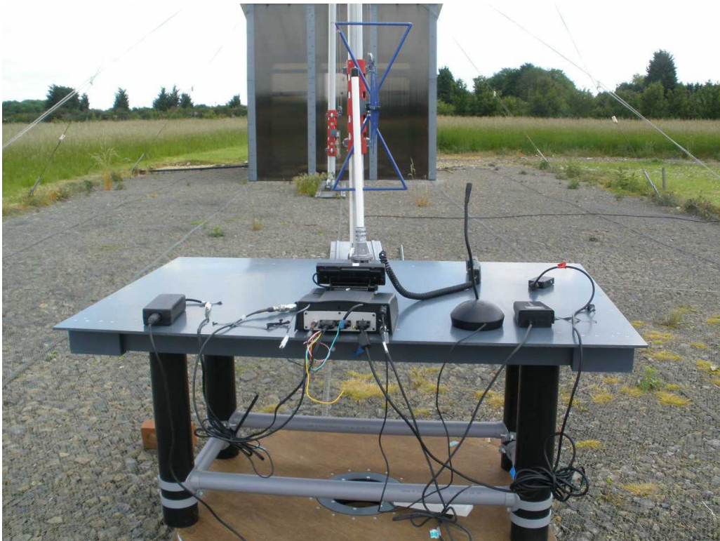
Photograph 5 DMU: Radiated Emissions - Back
