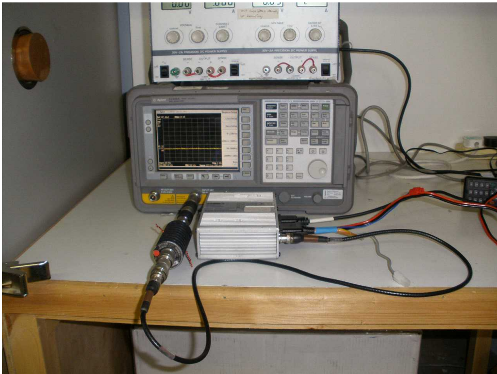
Photograph 1 SRG3500: Connected to Agilent Analyser
