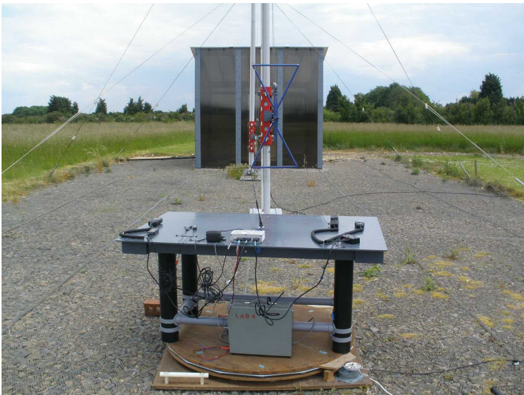
Photograph 3 Configuration 1: Radiated Emissions - Back
