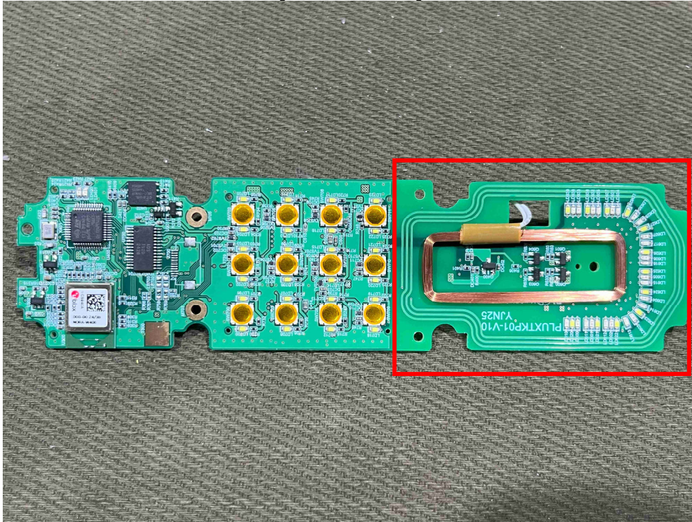
[125 kHz Antenna]
