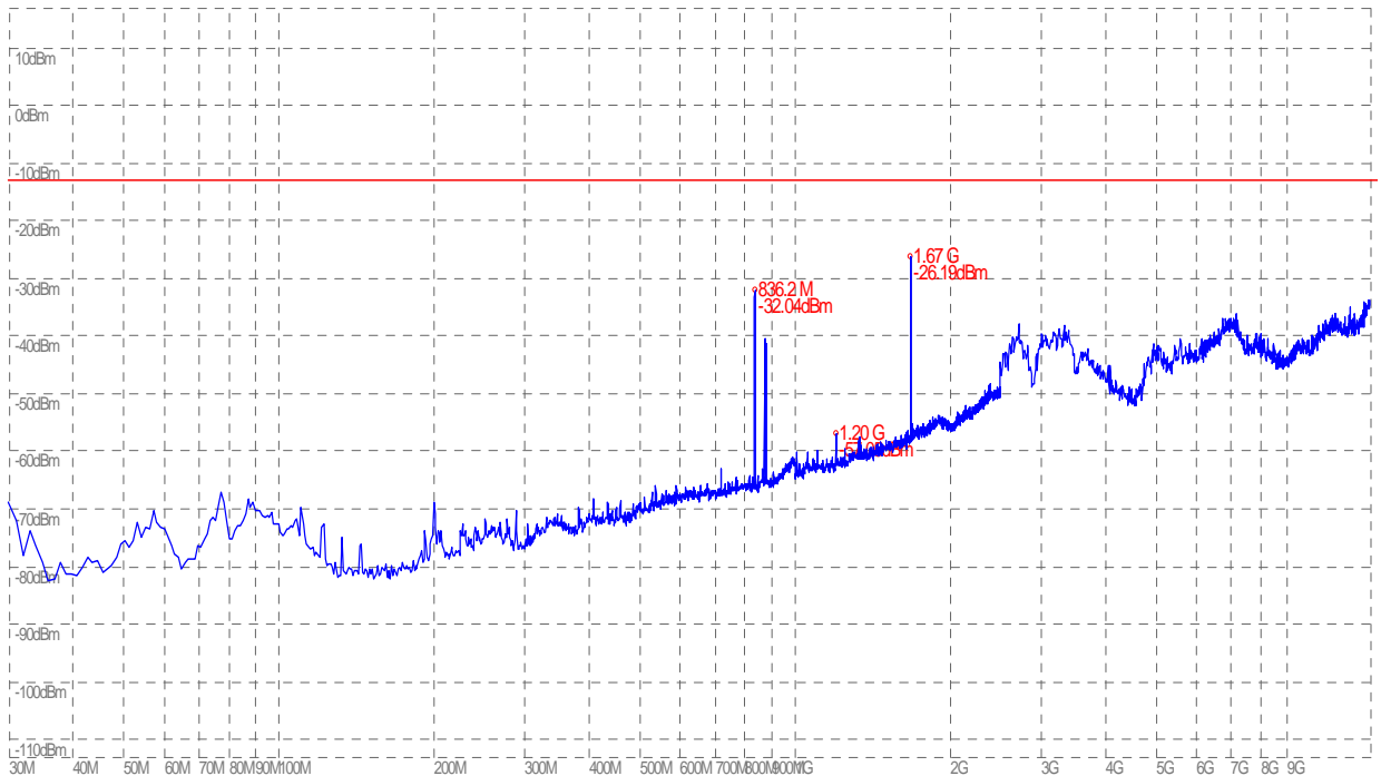
(Plot B.2: GSM 850MHz Channel = 190, Test Antenna Vertical)
