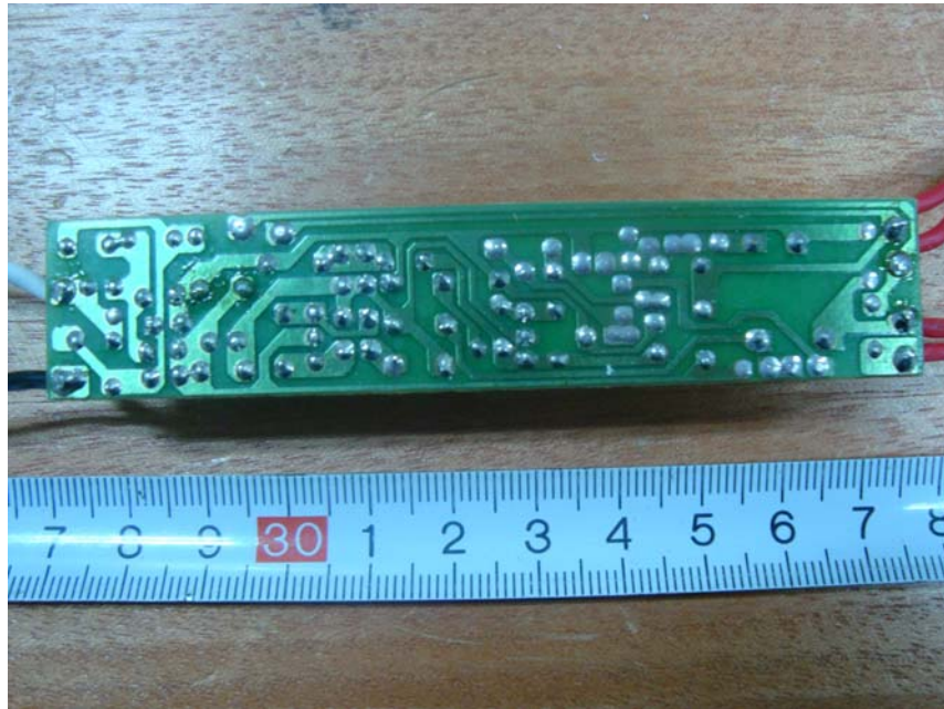
SSBT5-8W-L011: EUT – Main Board Circuit View
