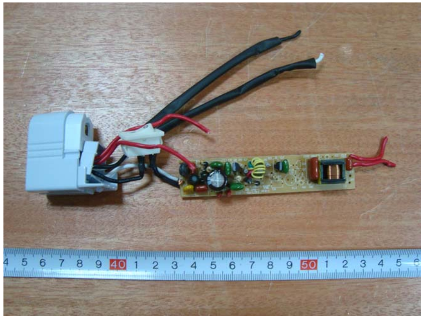
SSBT5-4W-L011: EUT – Internal Circuit View
