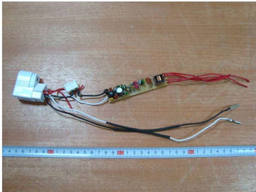
SSBT5-8W-L011: EUT – Internal Circuit View
