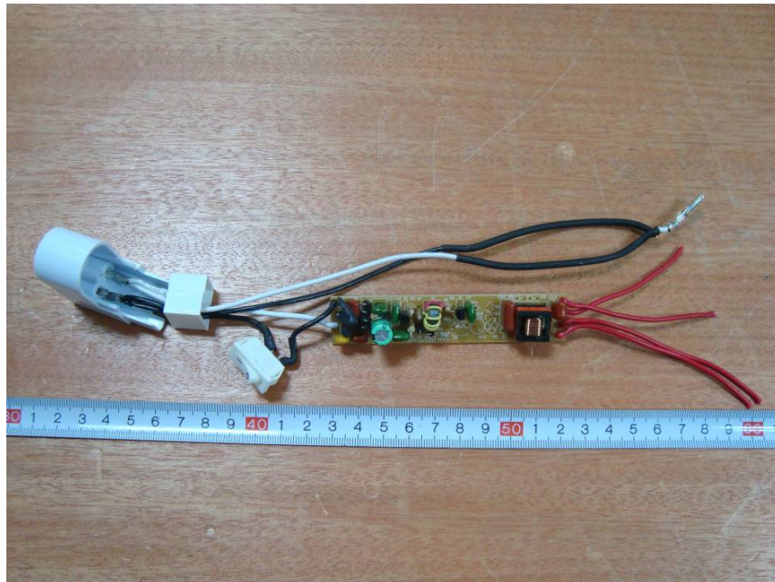
SSBT5-6W-L011: EUT – Internal Circuit View
