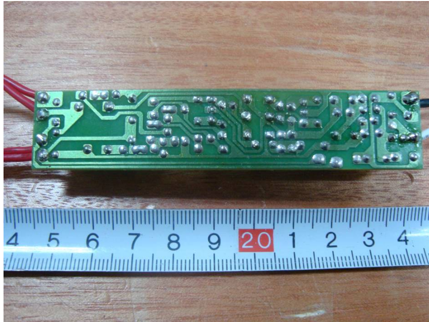
SSBT5-10W-L011: EUT – Main Board Circuit View
