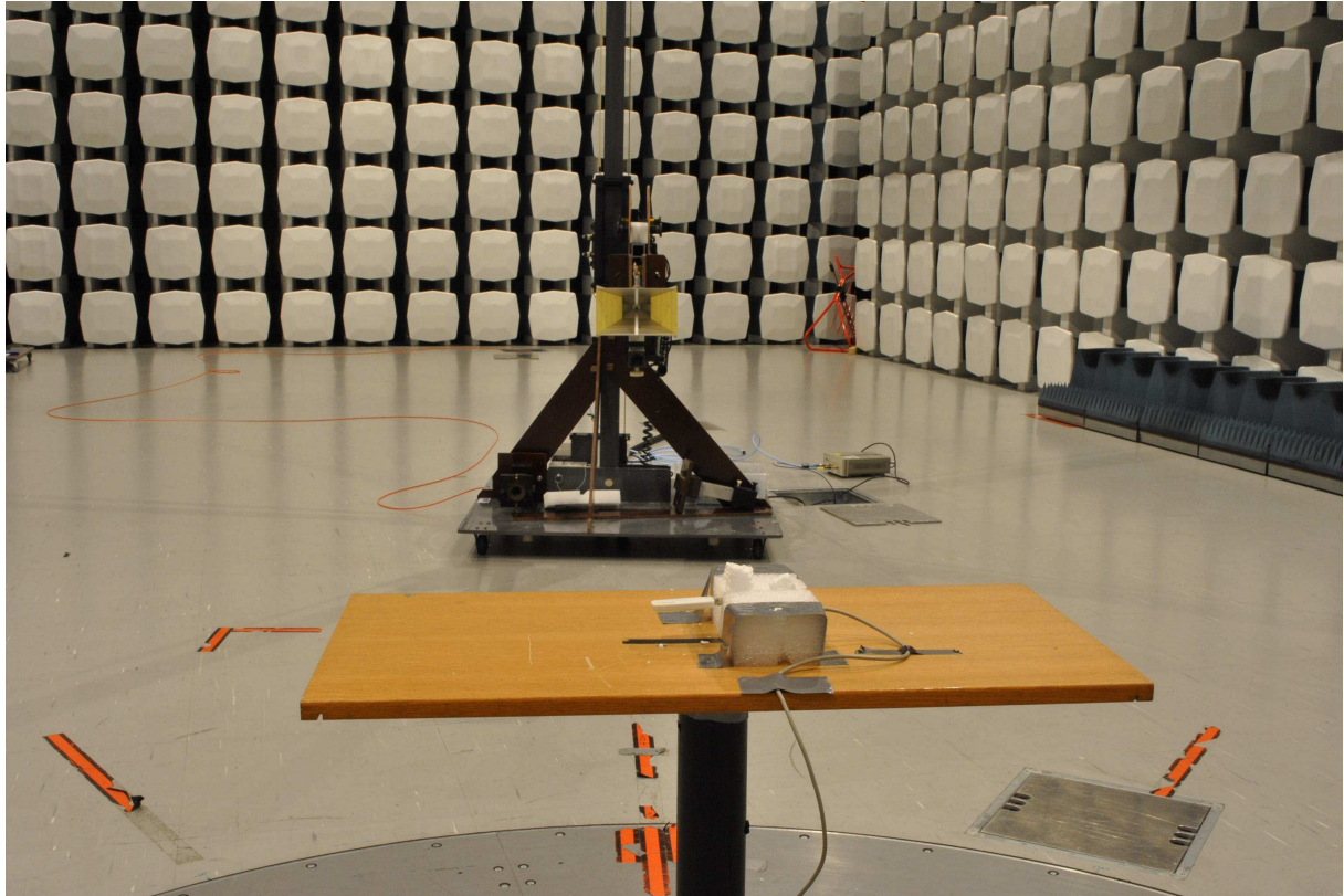
Radiated spurious emissions, 1 – 10 GHz
