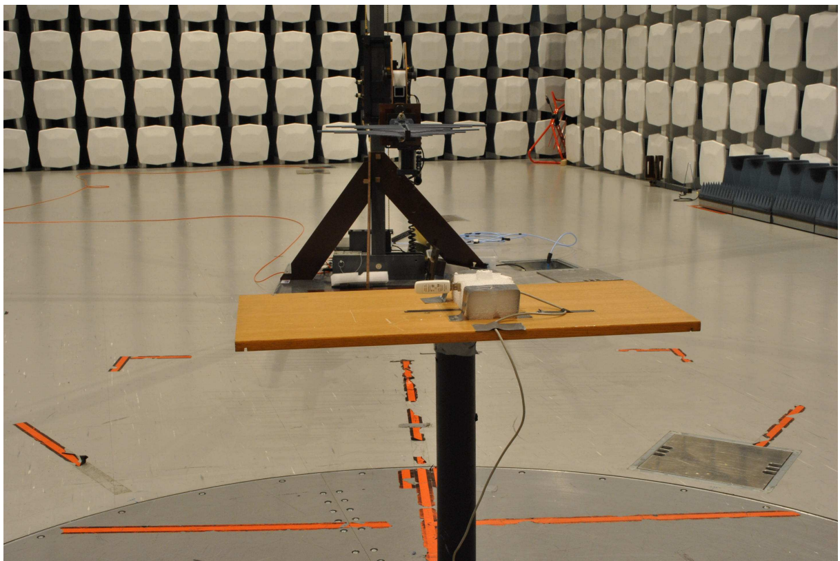
Radiated emissions – YZ plane
