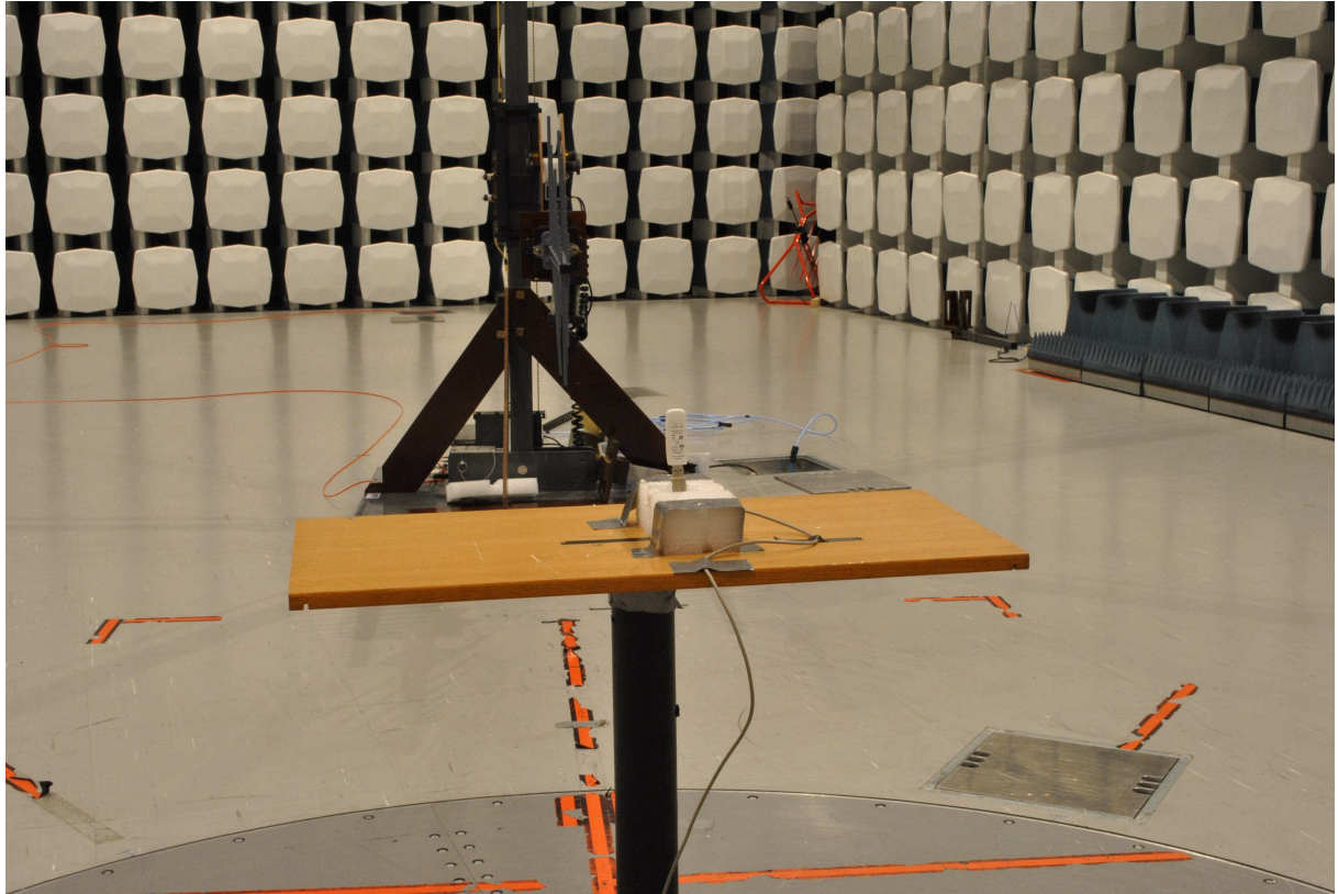
Radiated Emissions – XY plane
