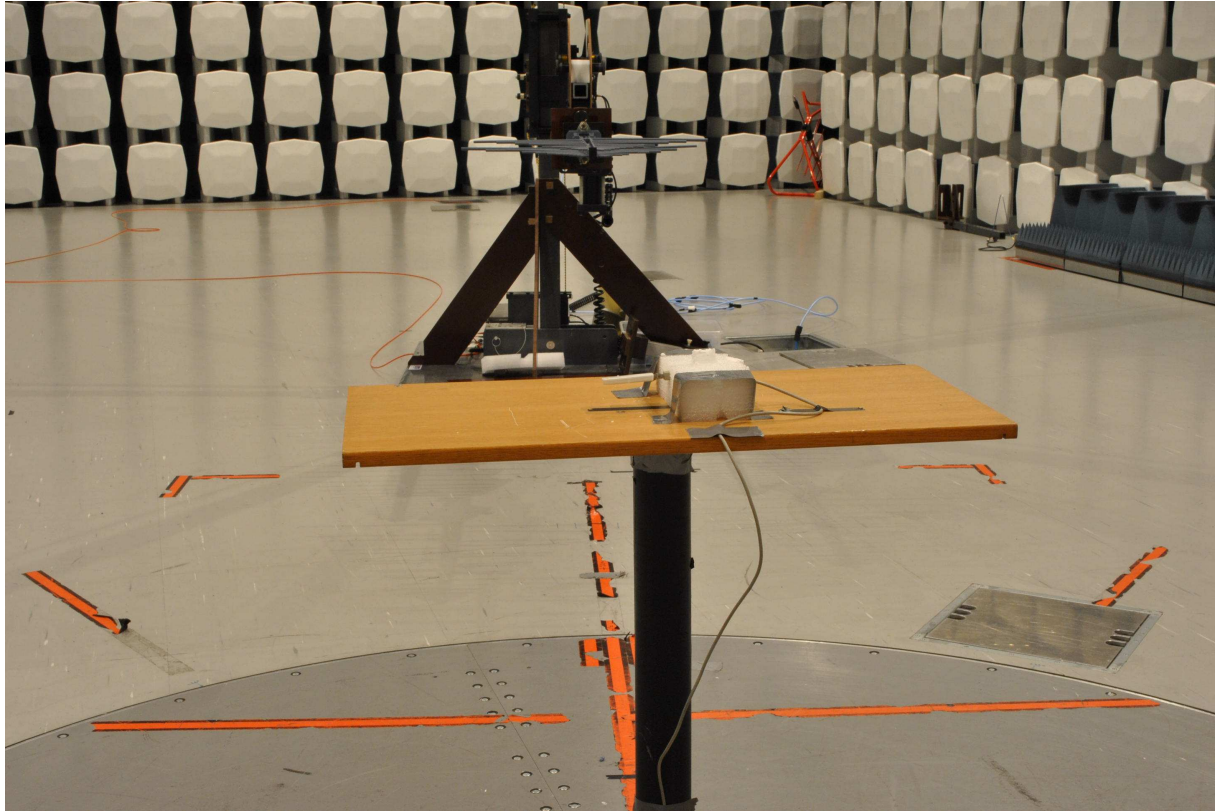
Radiated emissions – XZ plane
