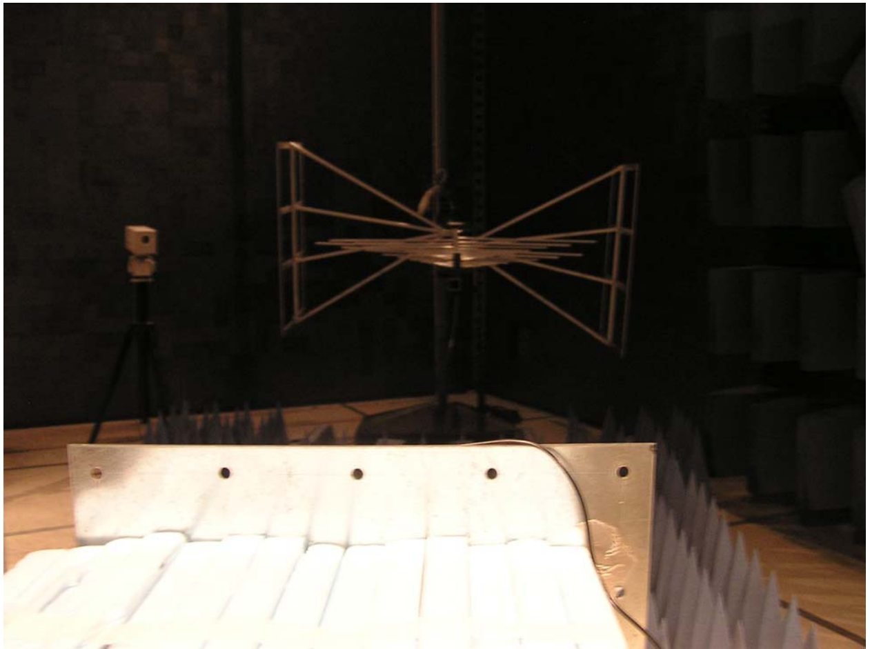
850 band ERP
