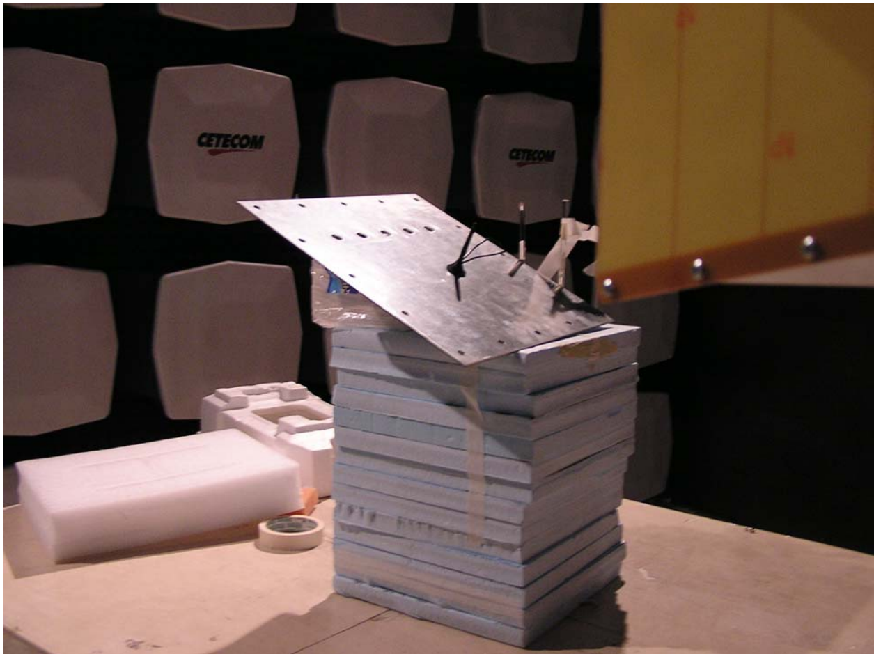
1900 band EIRP
