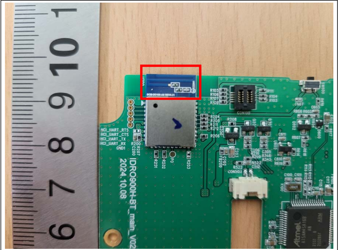
BT Antenna
