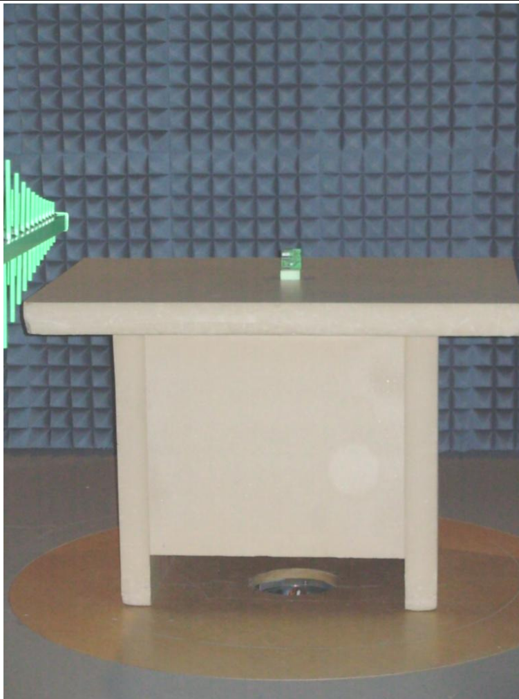
Figure 2: Measurement set-up for radiated measurement < 1 GHz acc. following sections of the report 1234-09-EE-10-PB006: 4.4.1 and 4.5.1
