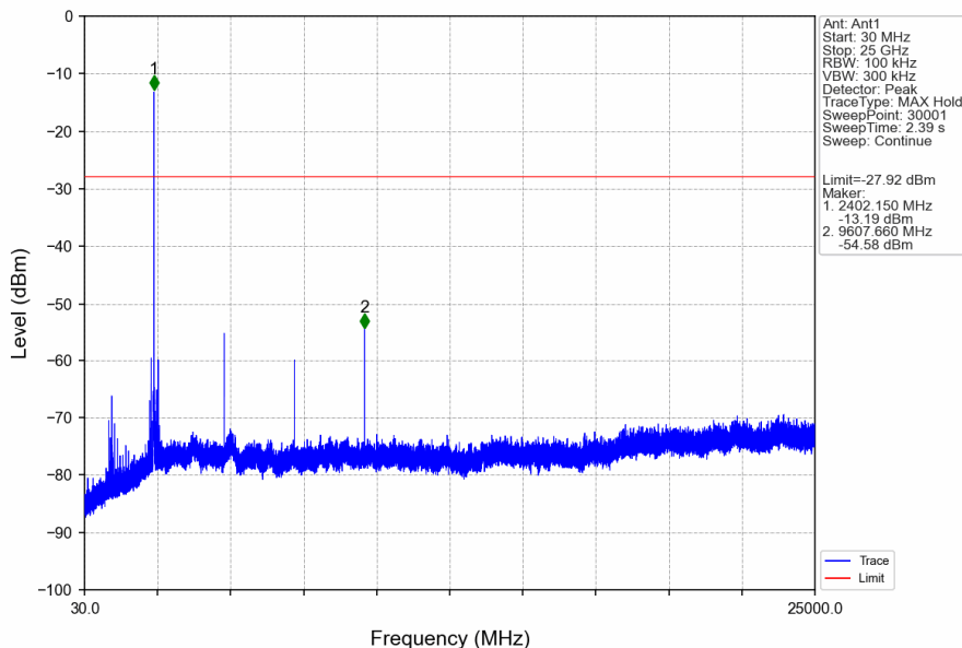
Pi/4DQPSK_2DH5_LCH_2402MHz_Ant1_NTNV
