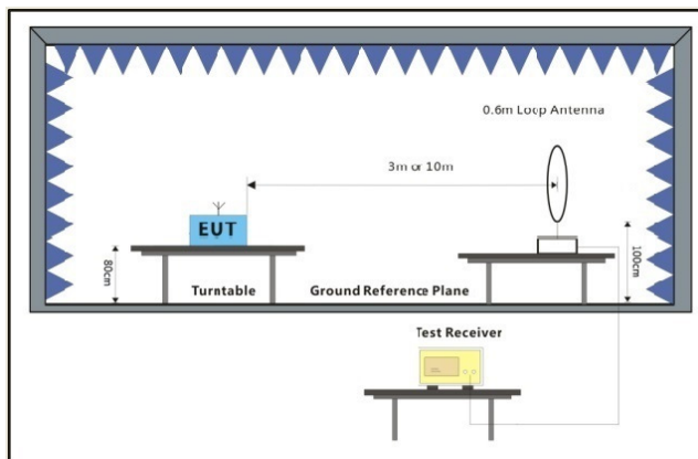
Below 30MHz
