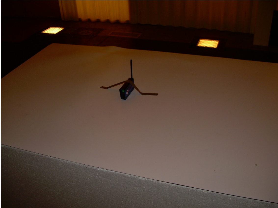
View of the Worst-Case Radiated Emission Test Setup (Vertical Alignment)
