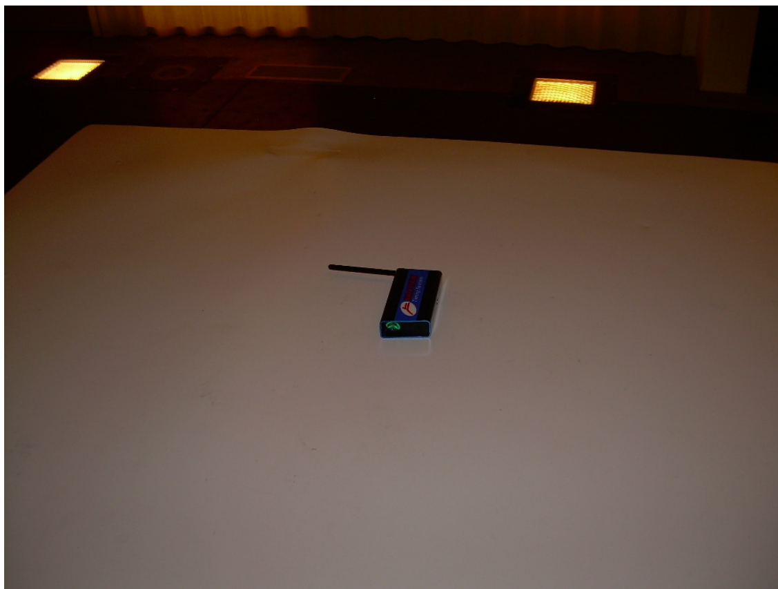
View of the Radiated Emission Test Setup (Horizontal Alignment)
