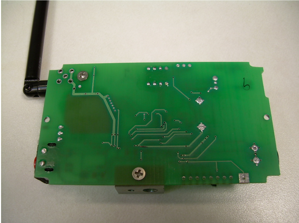
View of the Trace Side of the TC-PhotoGate A PCB
