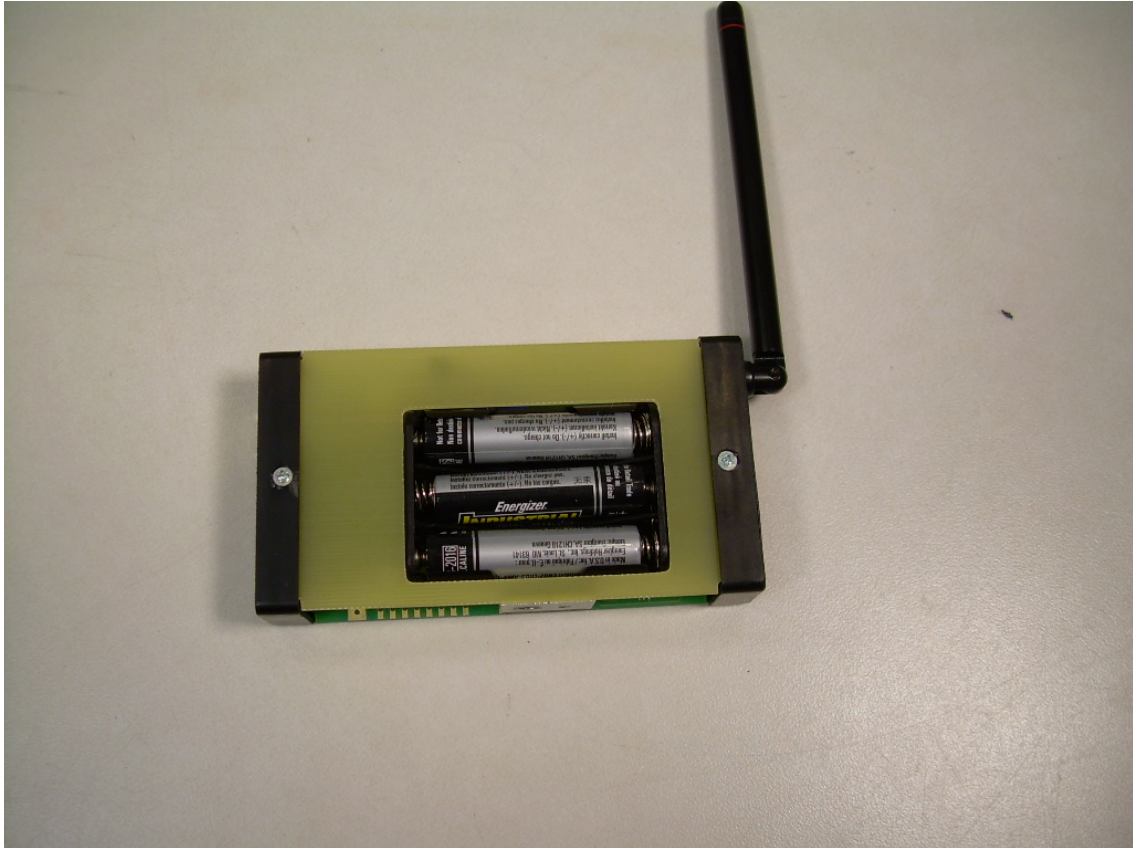
View of the TC-PhotoGate A with Housing Removed
