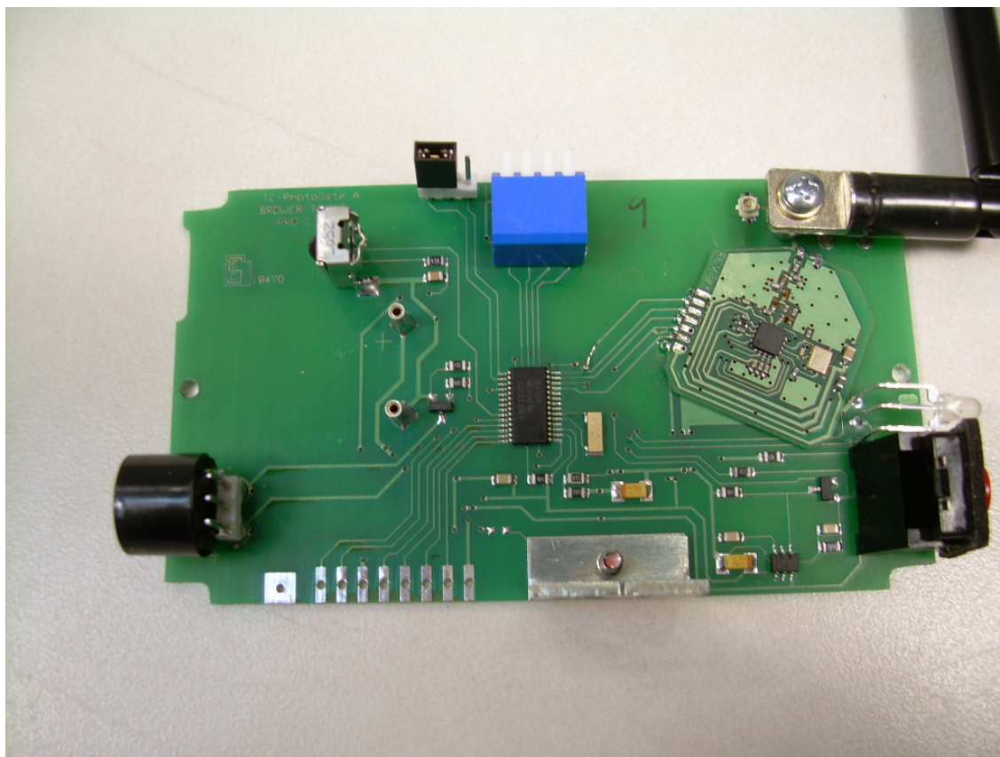
View of the Component Side of the TC-PhotoGate A PCB
