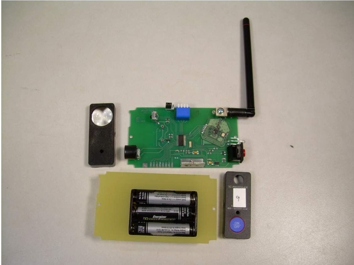
View of the Components of the TC-PhotoGate A
