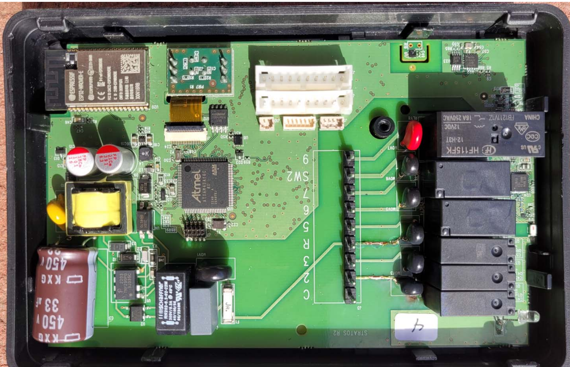
Top View of the PCB #2 - With Display
