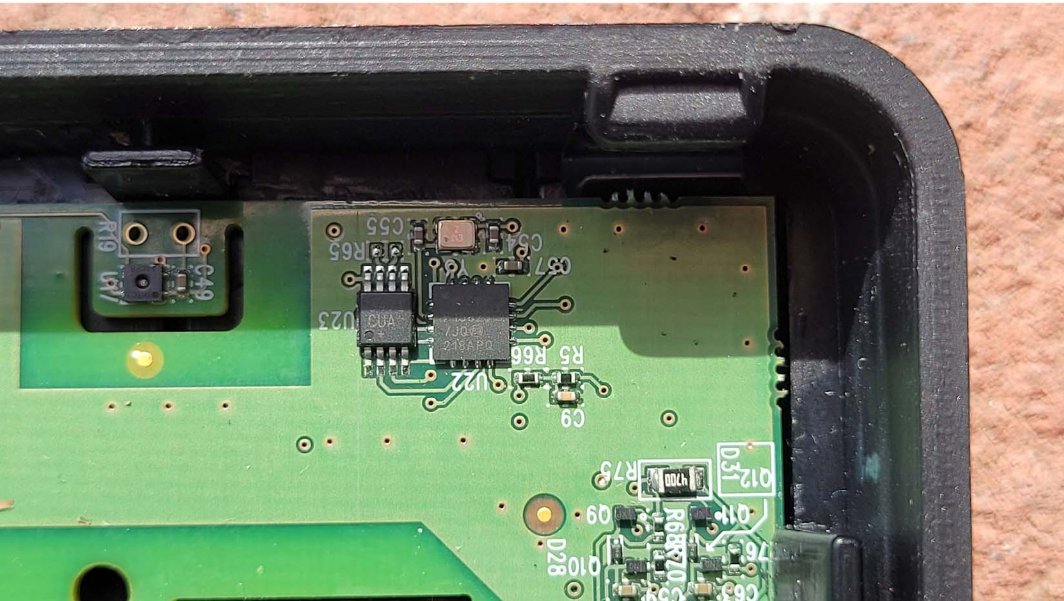
Top View of the PCB #7- With Display
