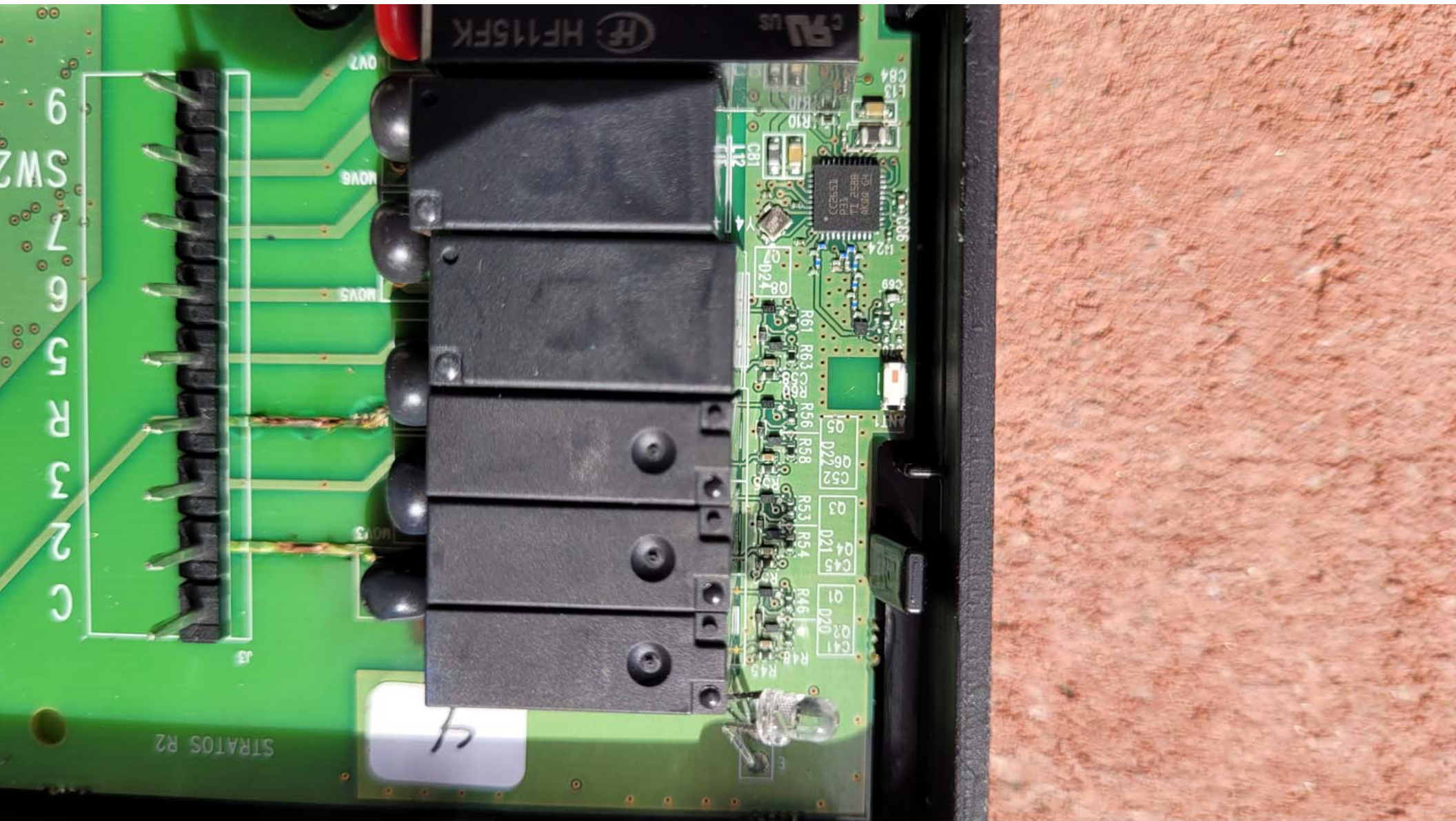
Top View of the PCB #11 - With Display
