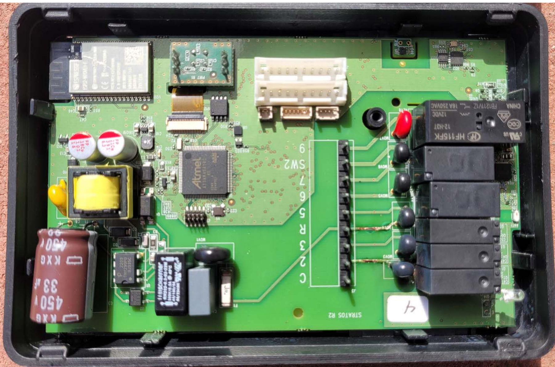
Top View of the PCB #1 - With Display
