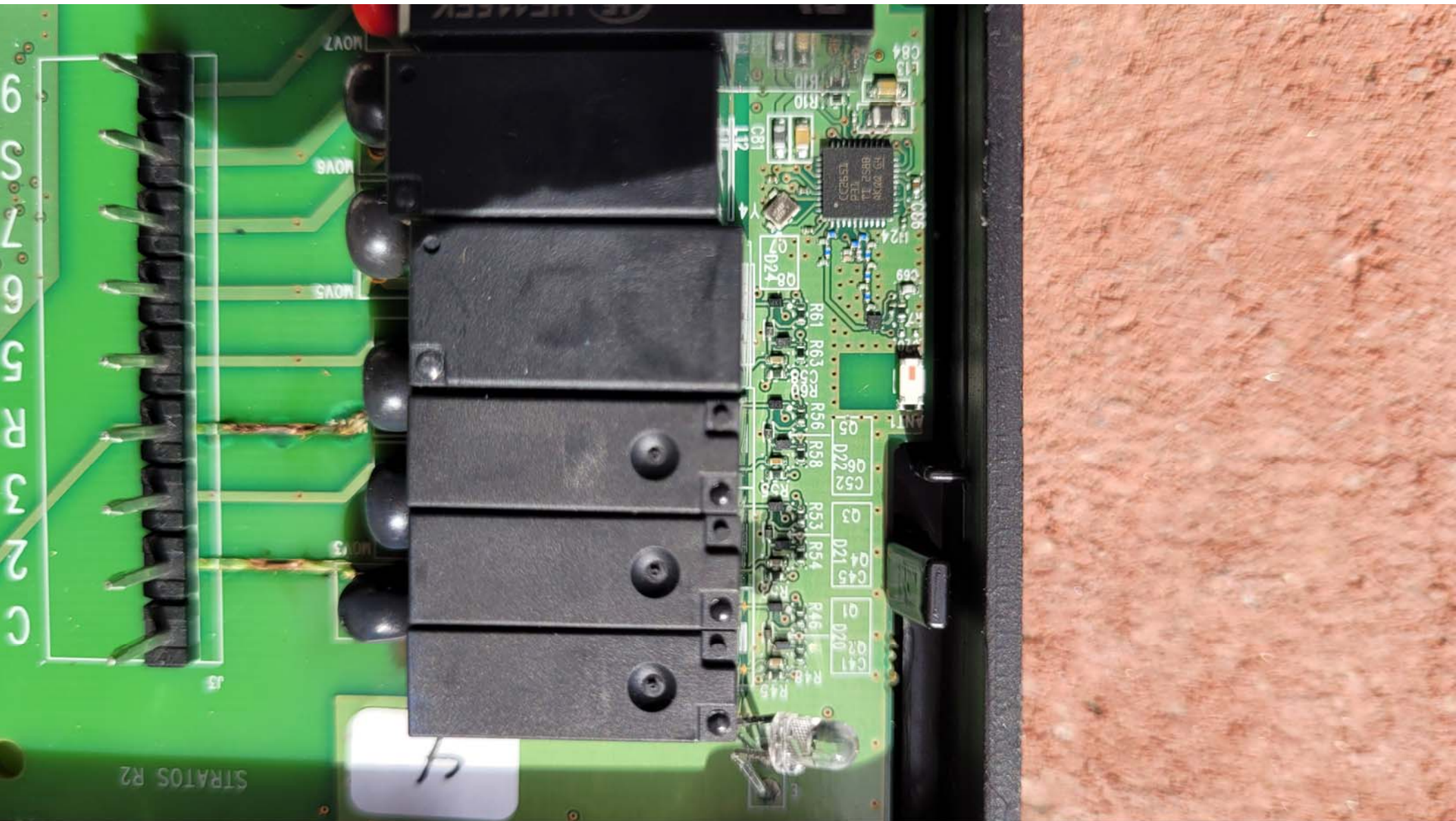
Top View of the PCB #10 - With Display
