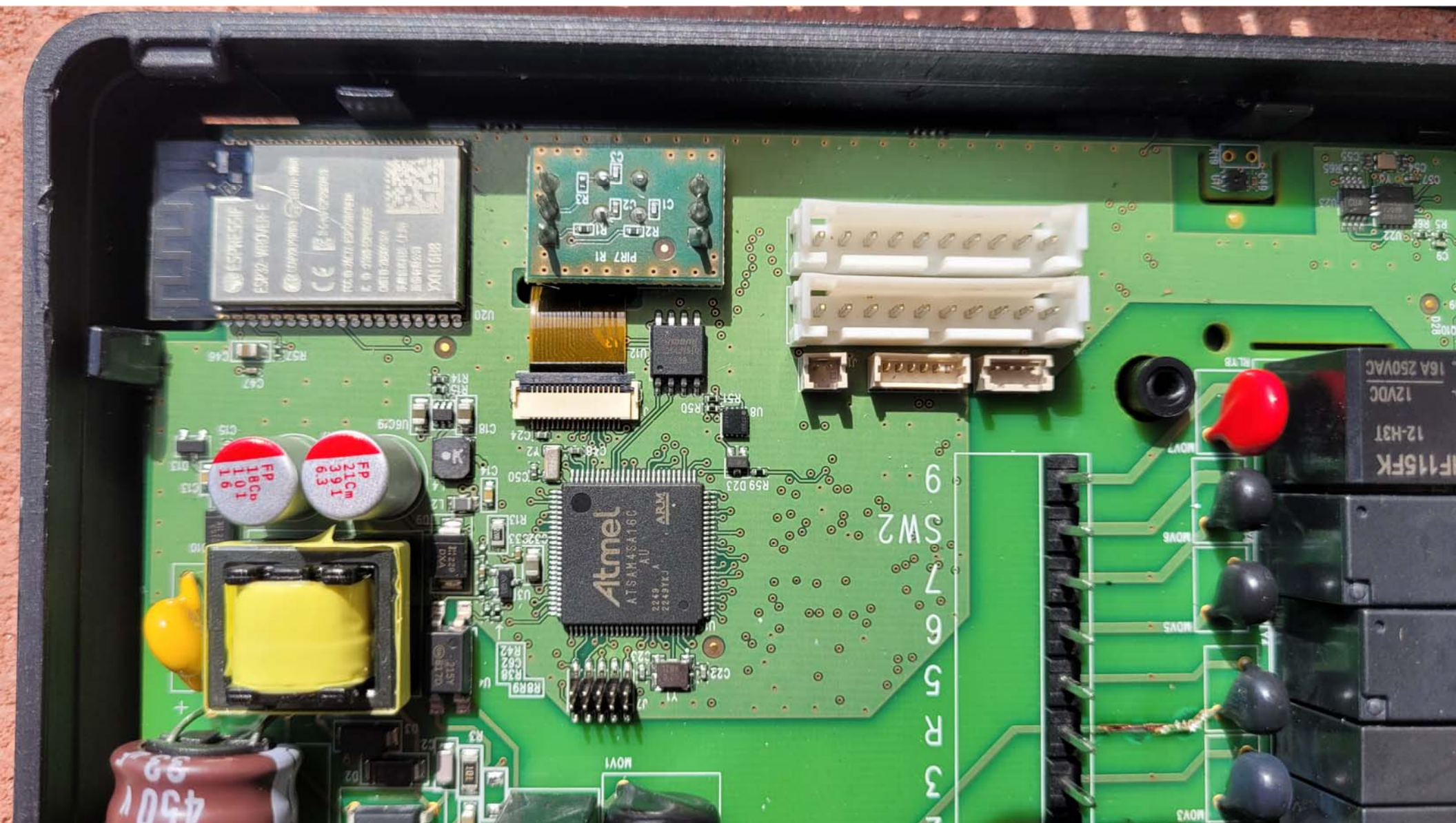
Top View of the PCB #4 - With Display
