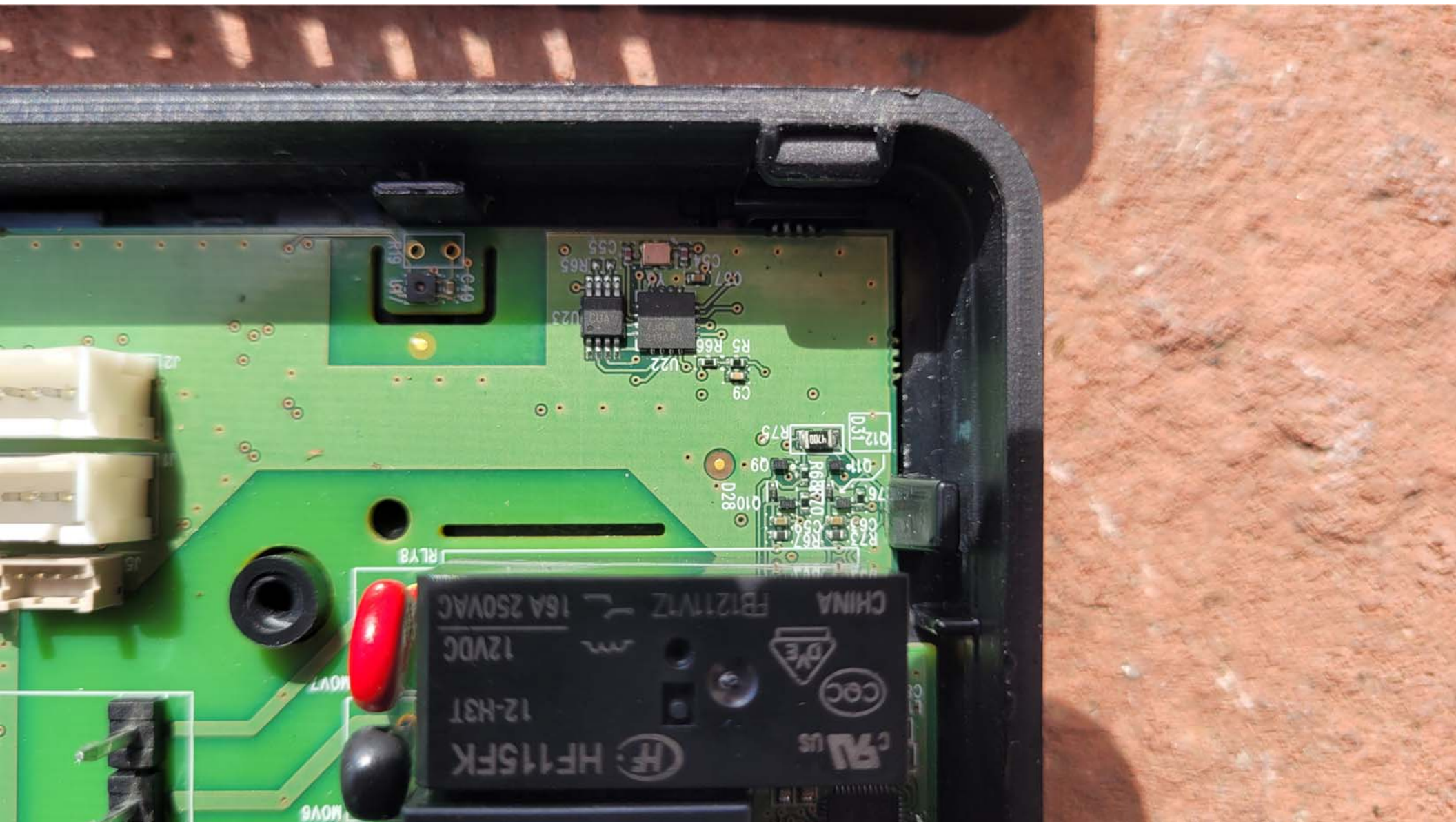
Top View of the PCB #5 - With Display
