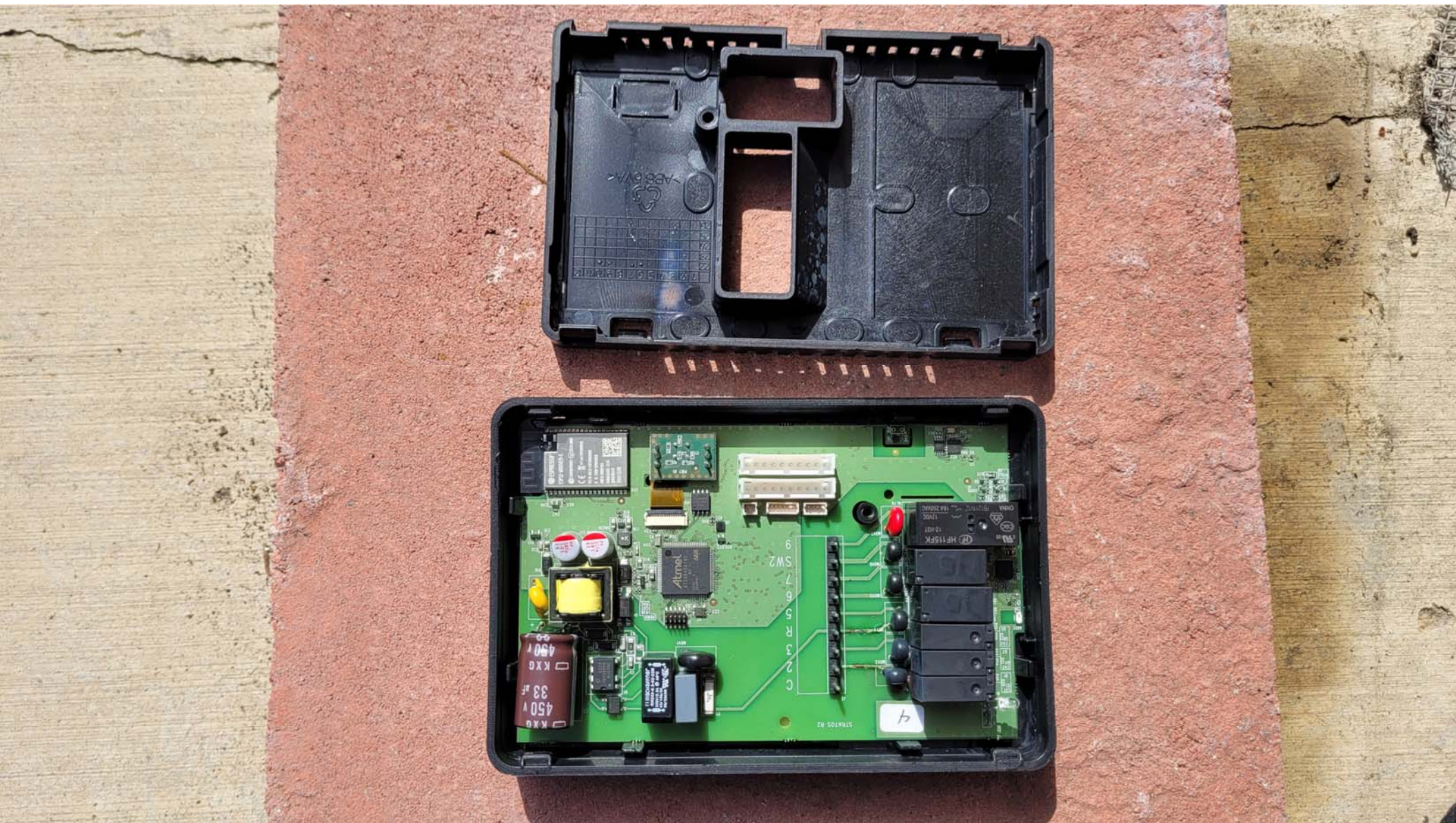
Inside View of the EUT #2 - With Display
