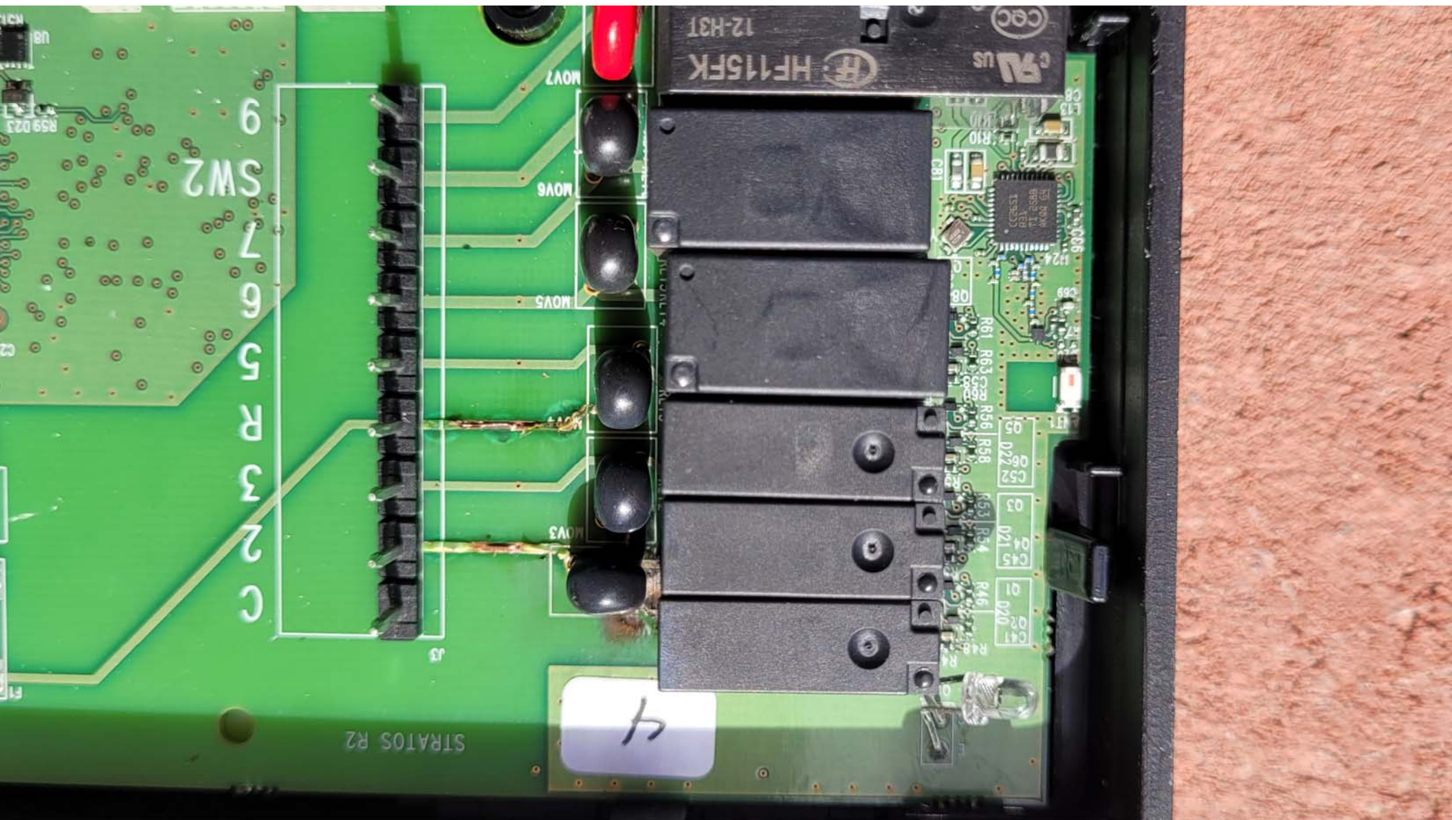
Top View of the PCB #9 - With Display
