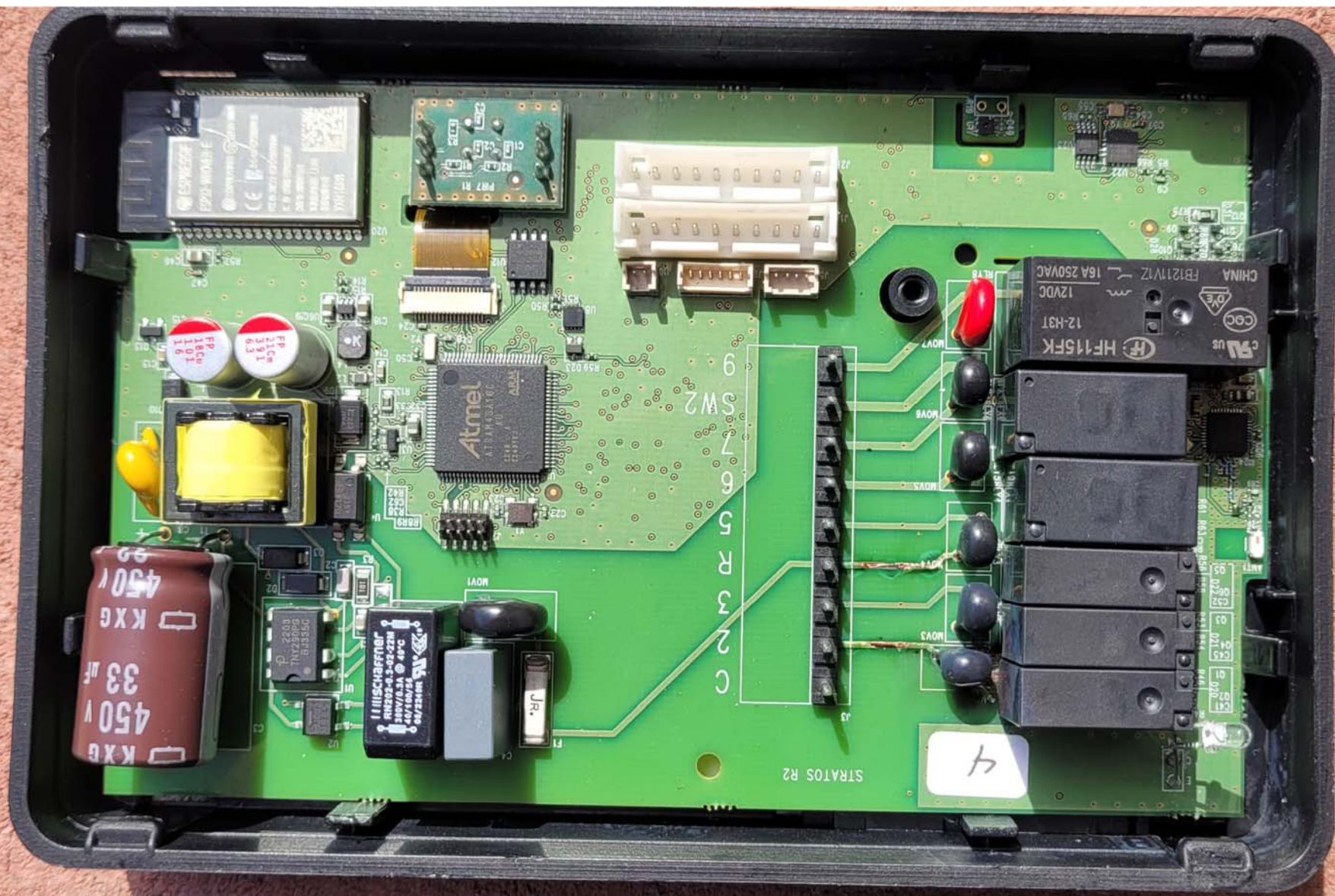
Top View of the PCB #5 - With Display
