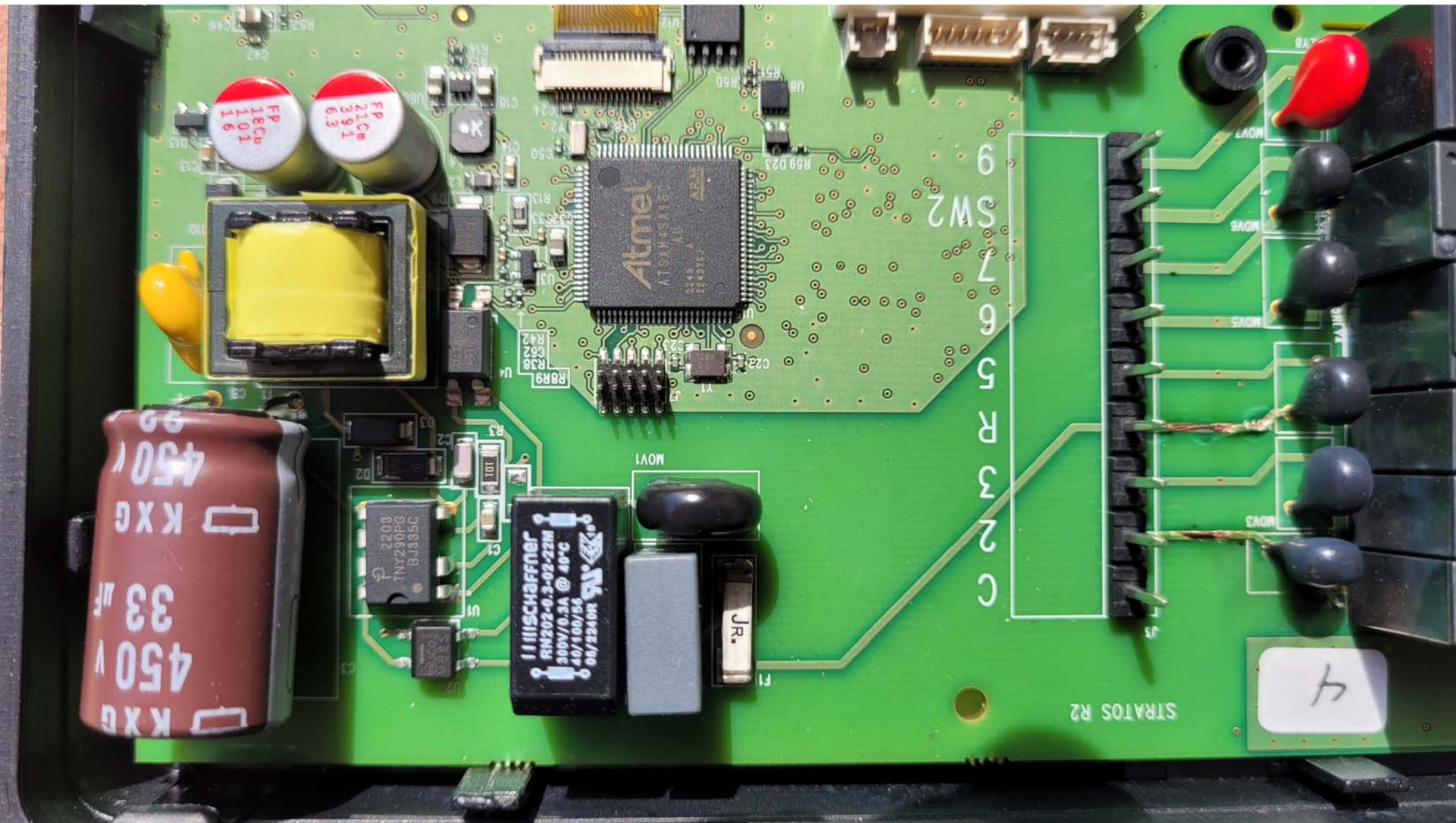
Top View of the PCB #3 - With Display
