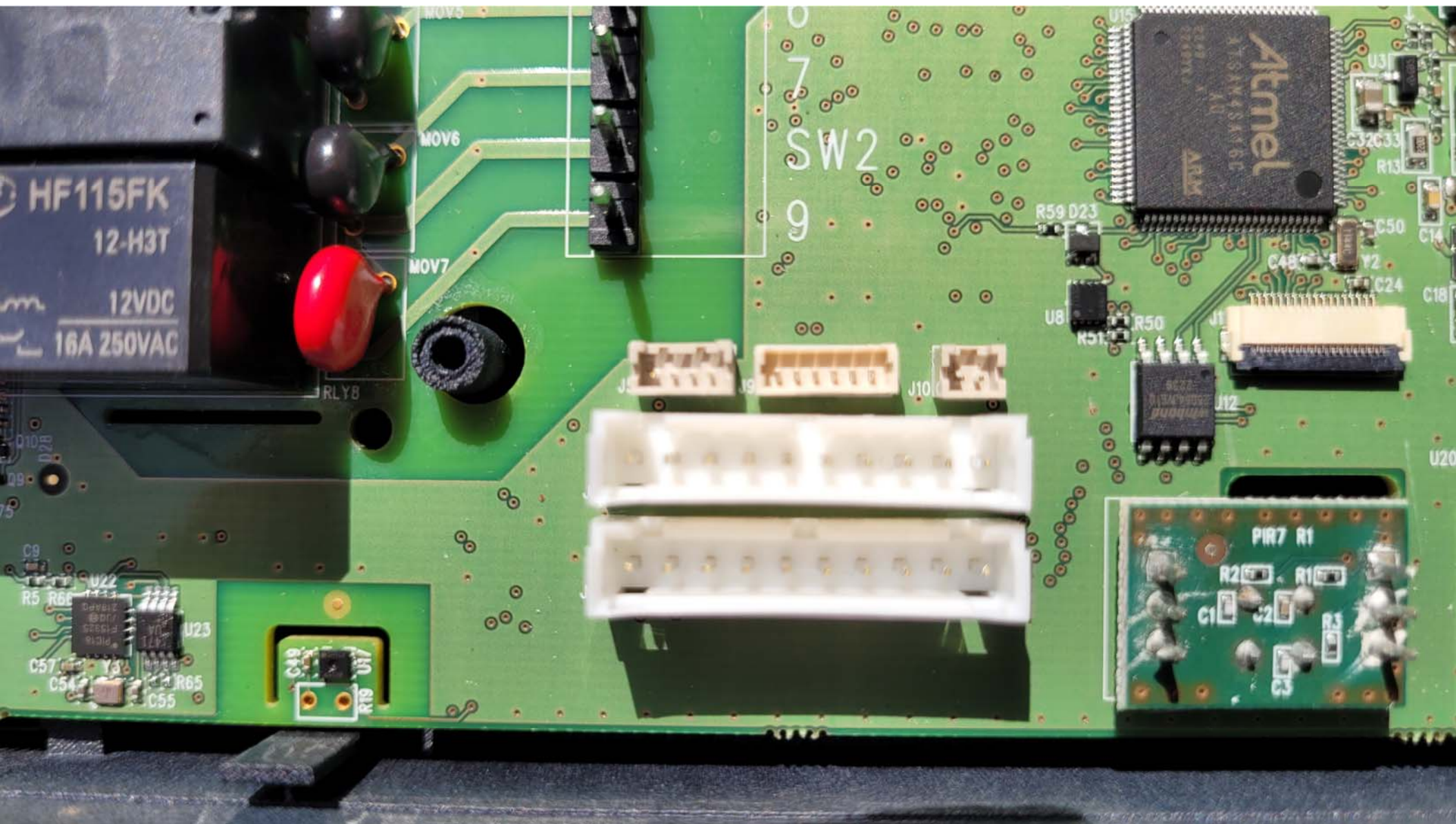
Top View of PCB - Closeup #4 - No Display
