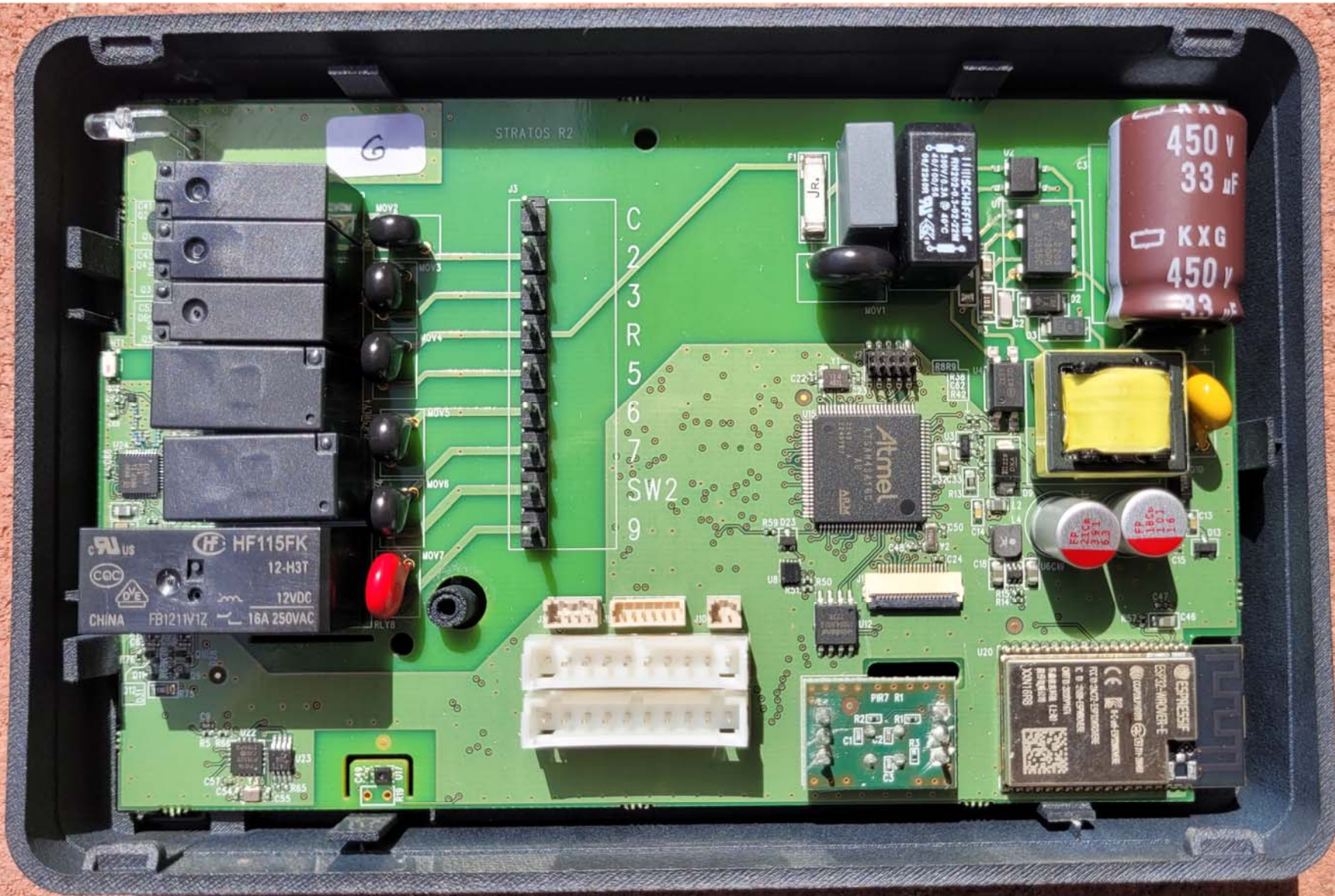
Top View of the PCB - No Display
