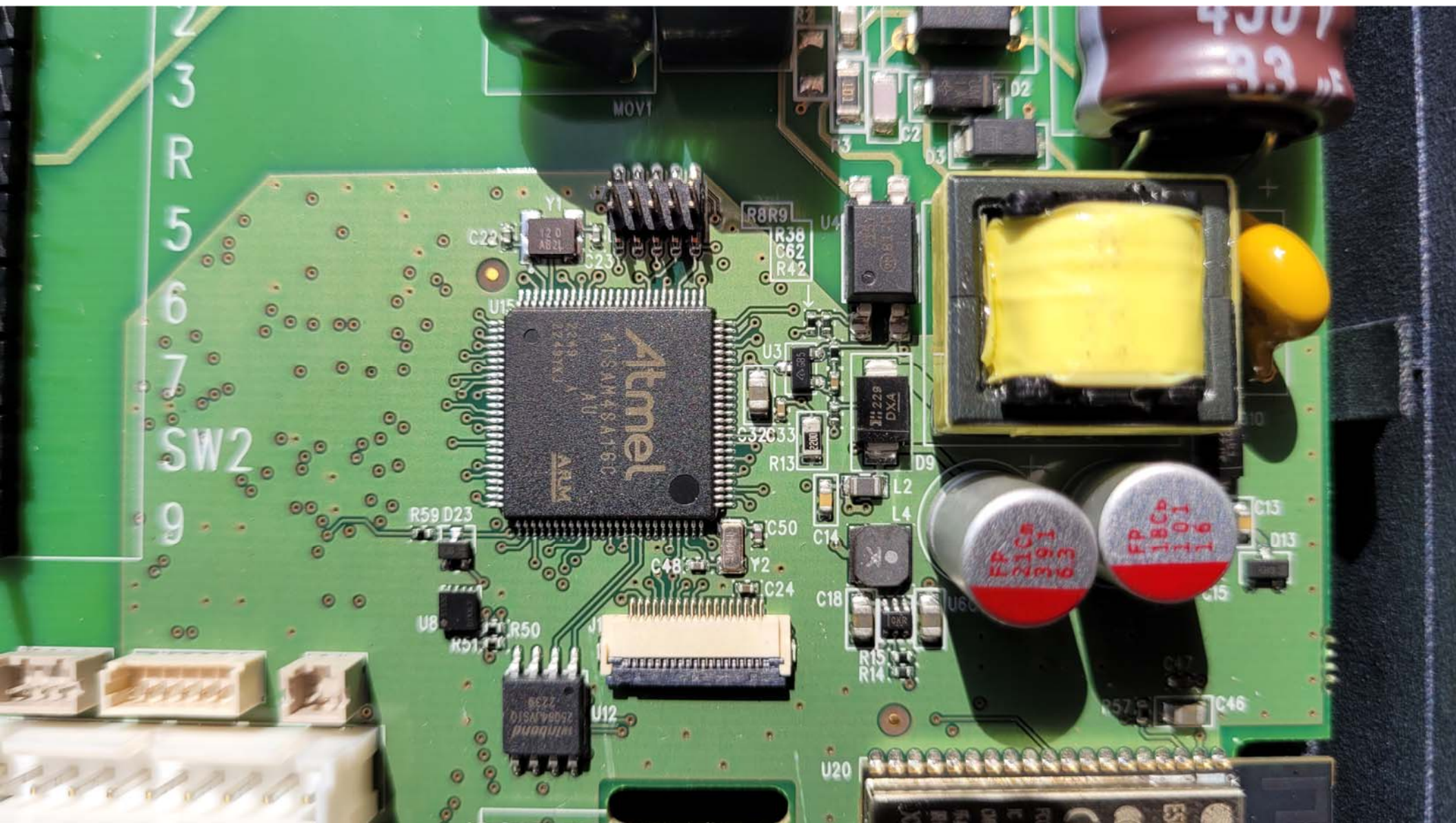
Top View of PCB - Closeup #2 - No Display
