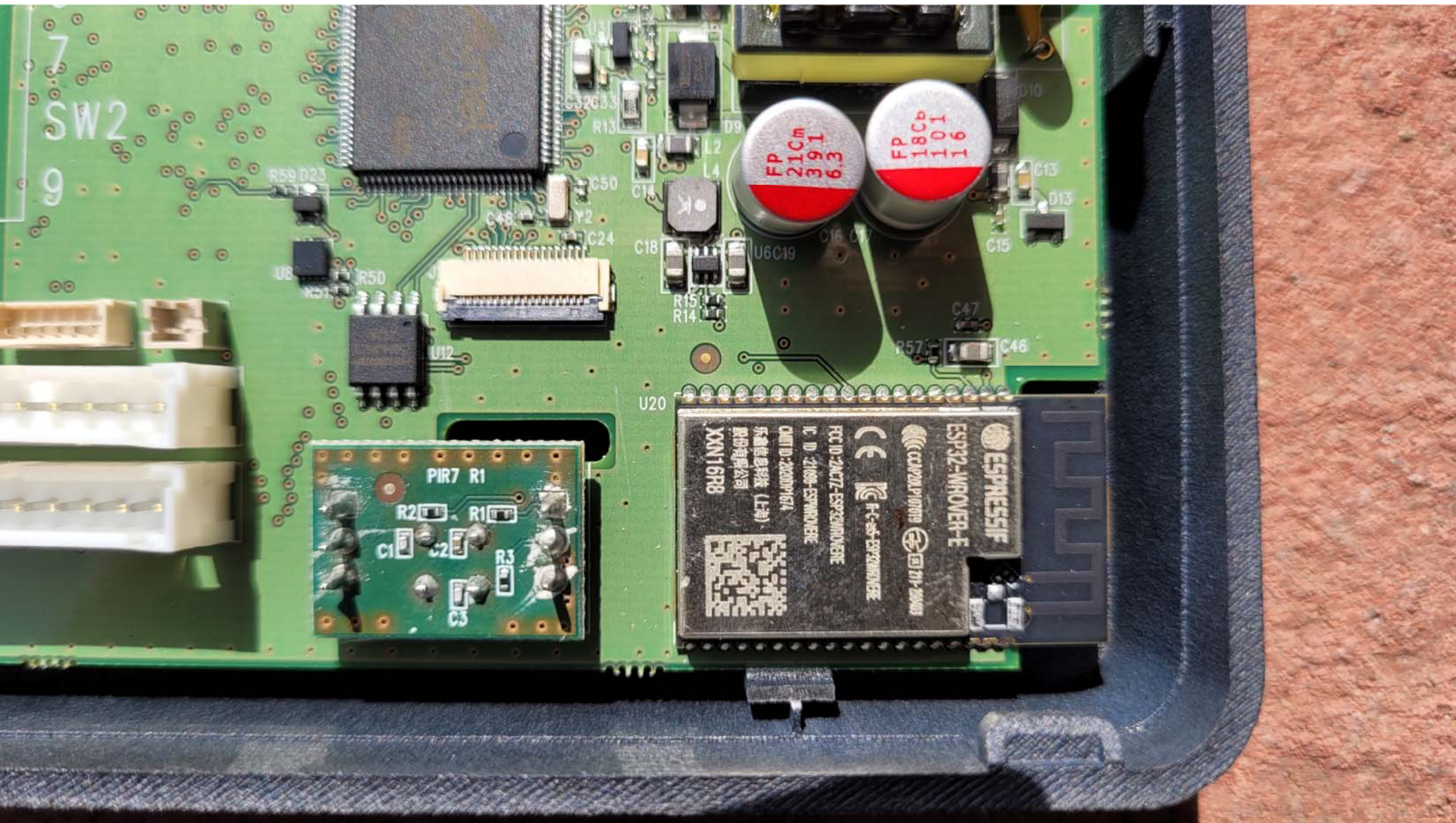
Top View of PCB - Closeup #5 - No Display
