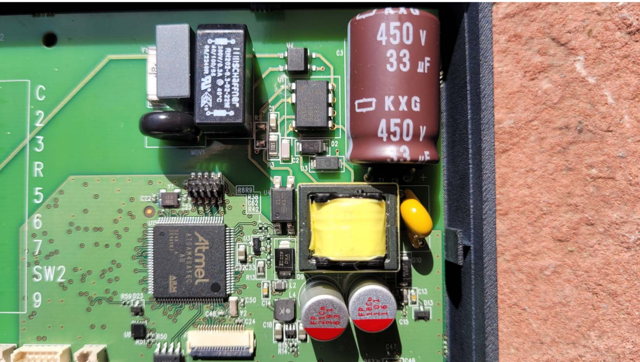
Top View of PCB - Closeup #1 - No Display
