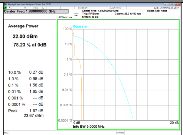
Band 2-15KHz-1#0-QPSK-Mid
