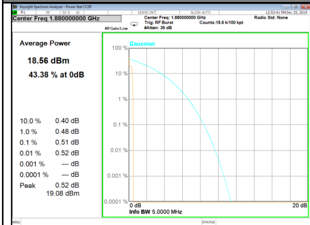
Band 2-3.75KHz-1#47-BPSK-Mid
