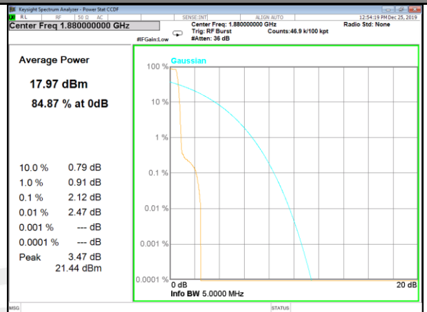
Band 2-3.75KHz-1#47-QPSK-Mid
