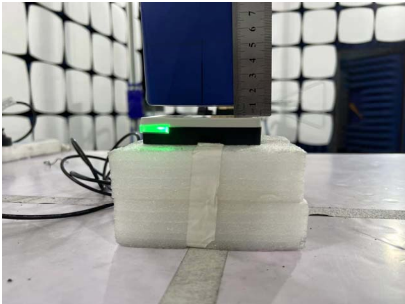
Back Side_10mm
