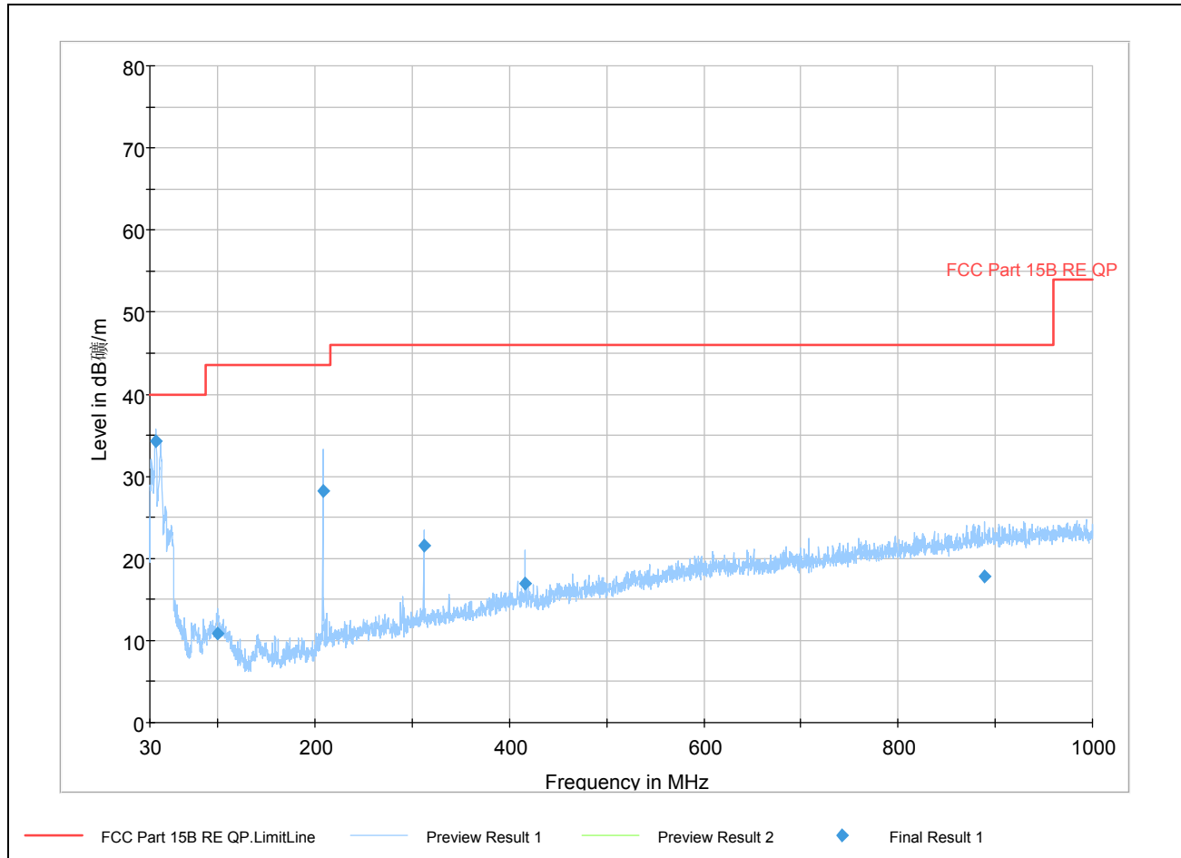
Radiates Emission from 30MHz to 1GHz
