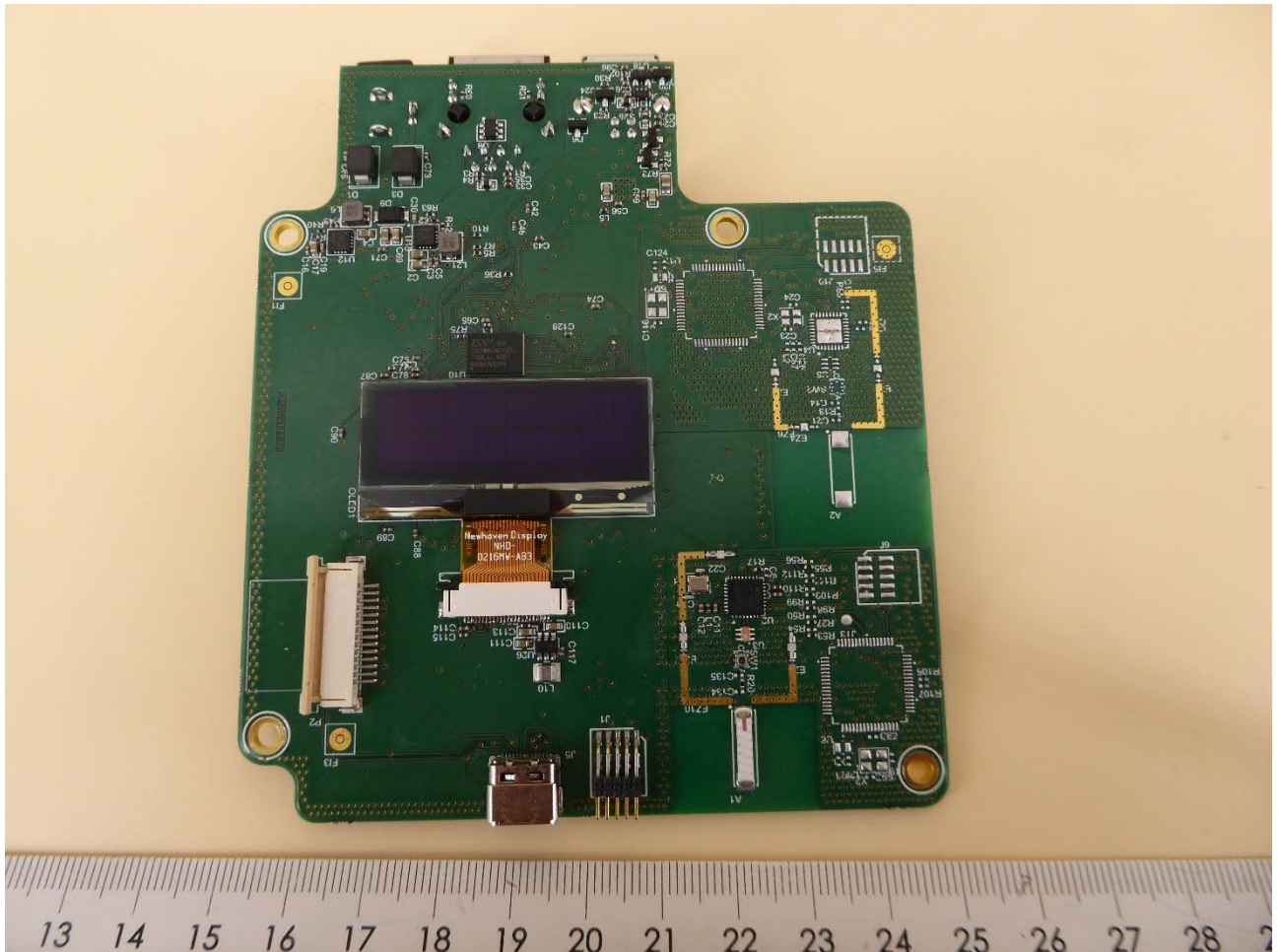
EUT – RS Main PCB (bottom view)
