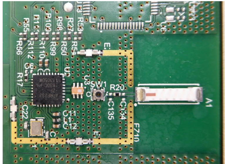
EUT radio part (detail view)
