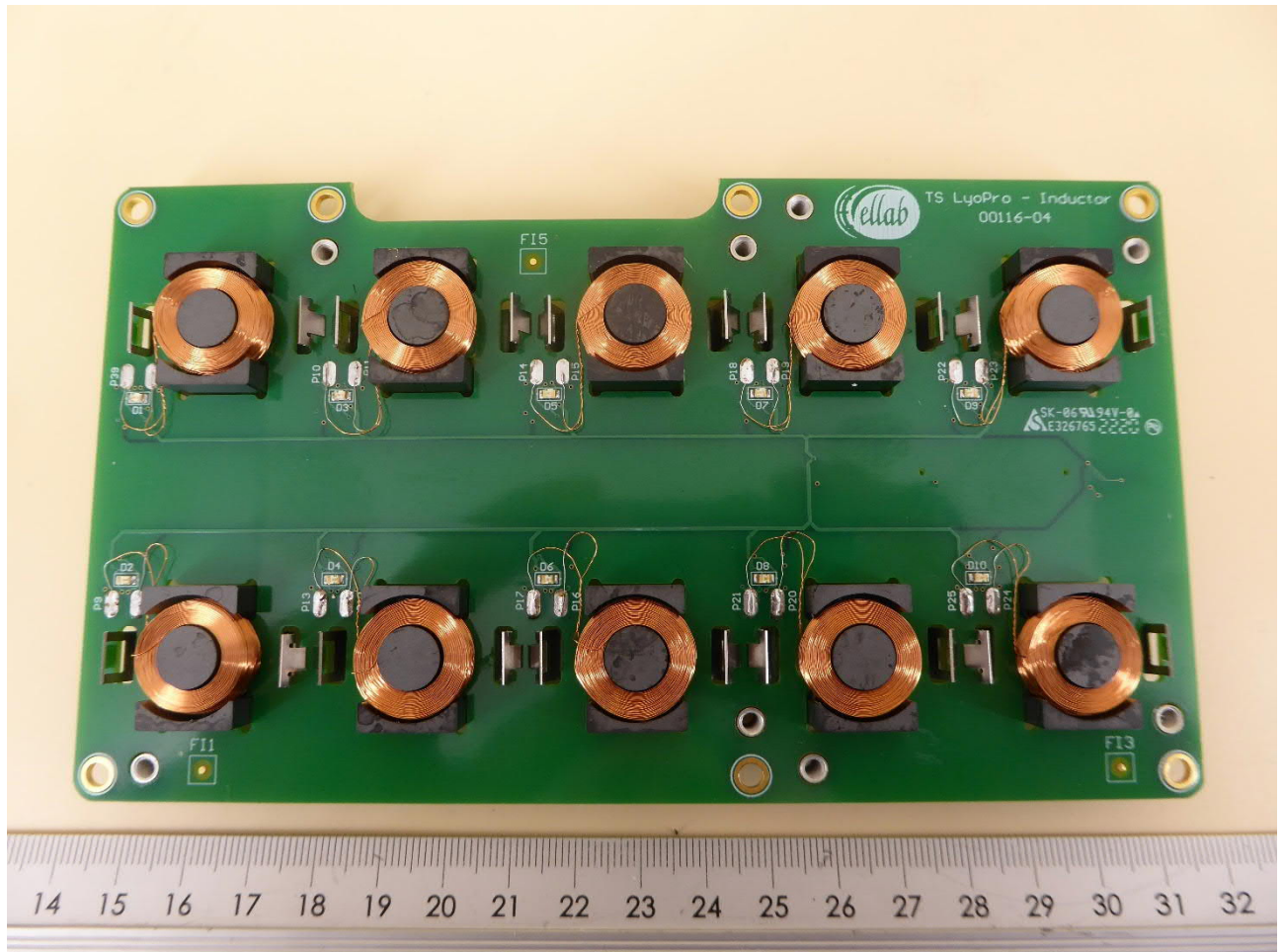
EUT – Inductor PCB (top view)
