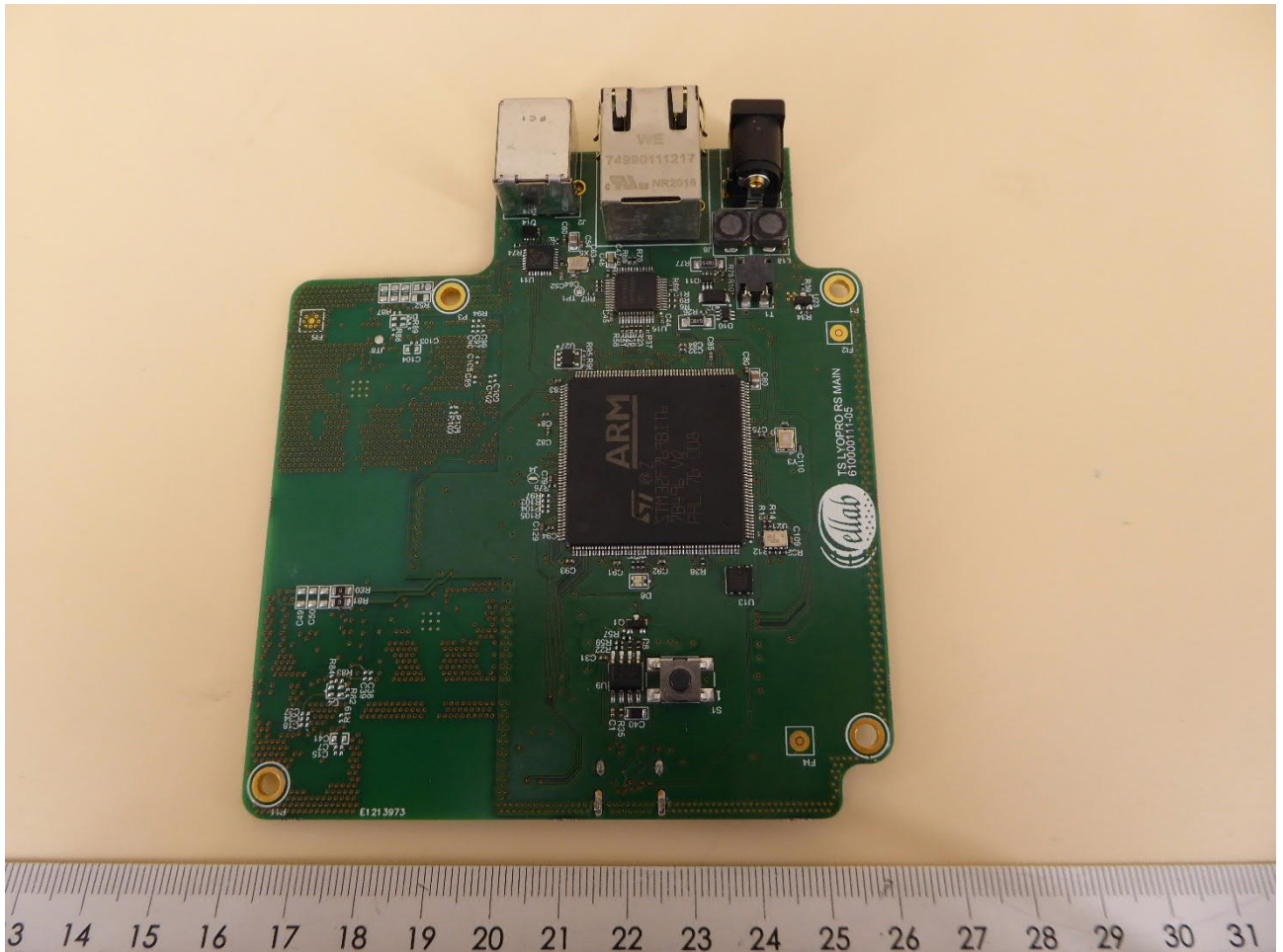
EUT – RS Main PCB (top view)
