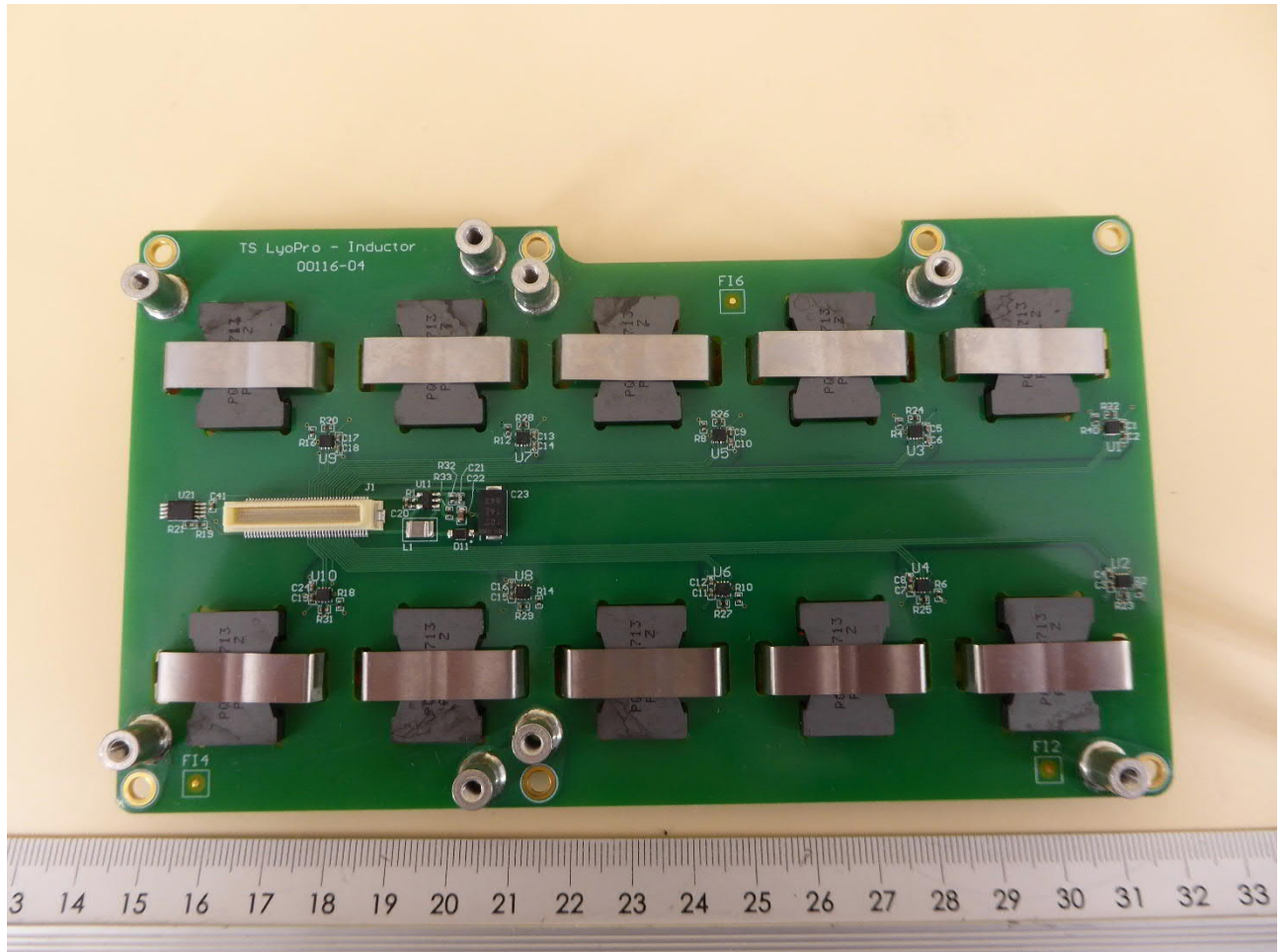
EUT – Inductor PCB (bottom view)
