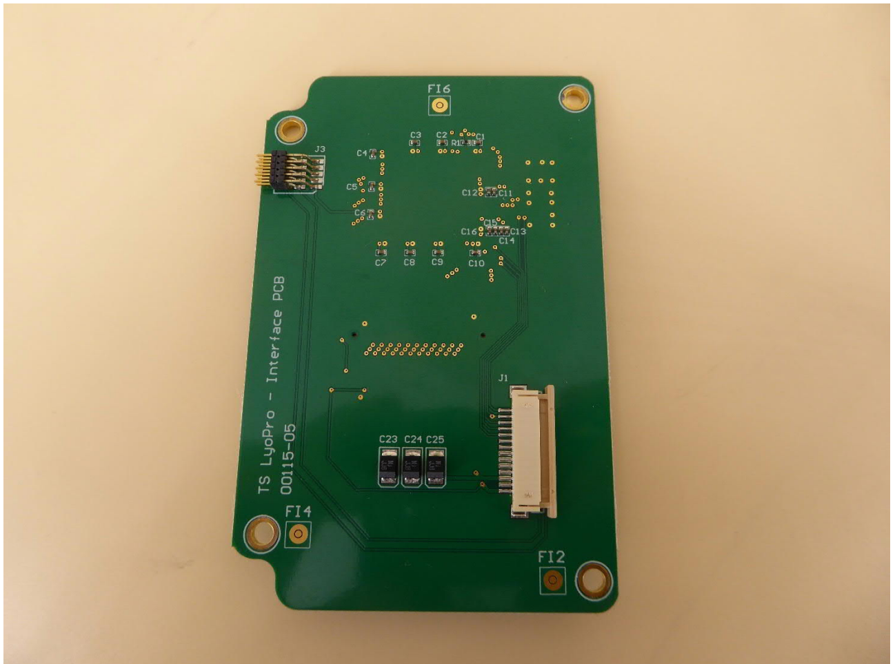
EUT – Interface PCB (bottom view)
