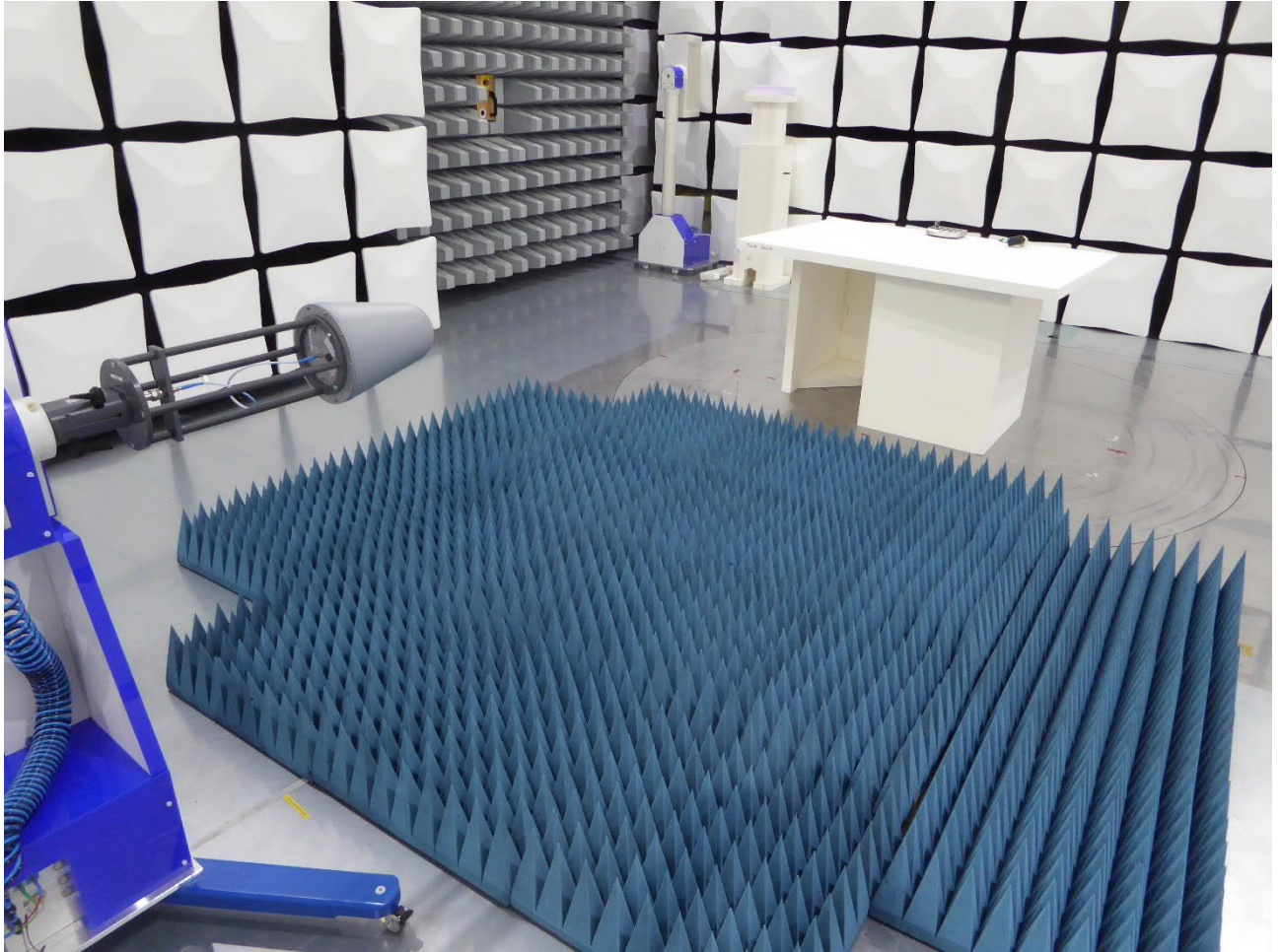
Test setup semi anechoic chamber TX spurious emissions from 1 GHz – 13GHz
