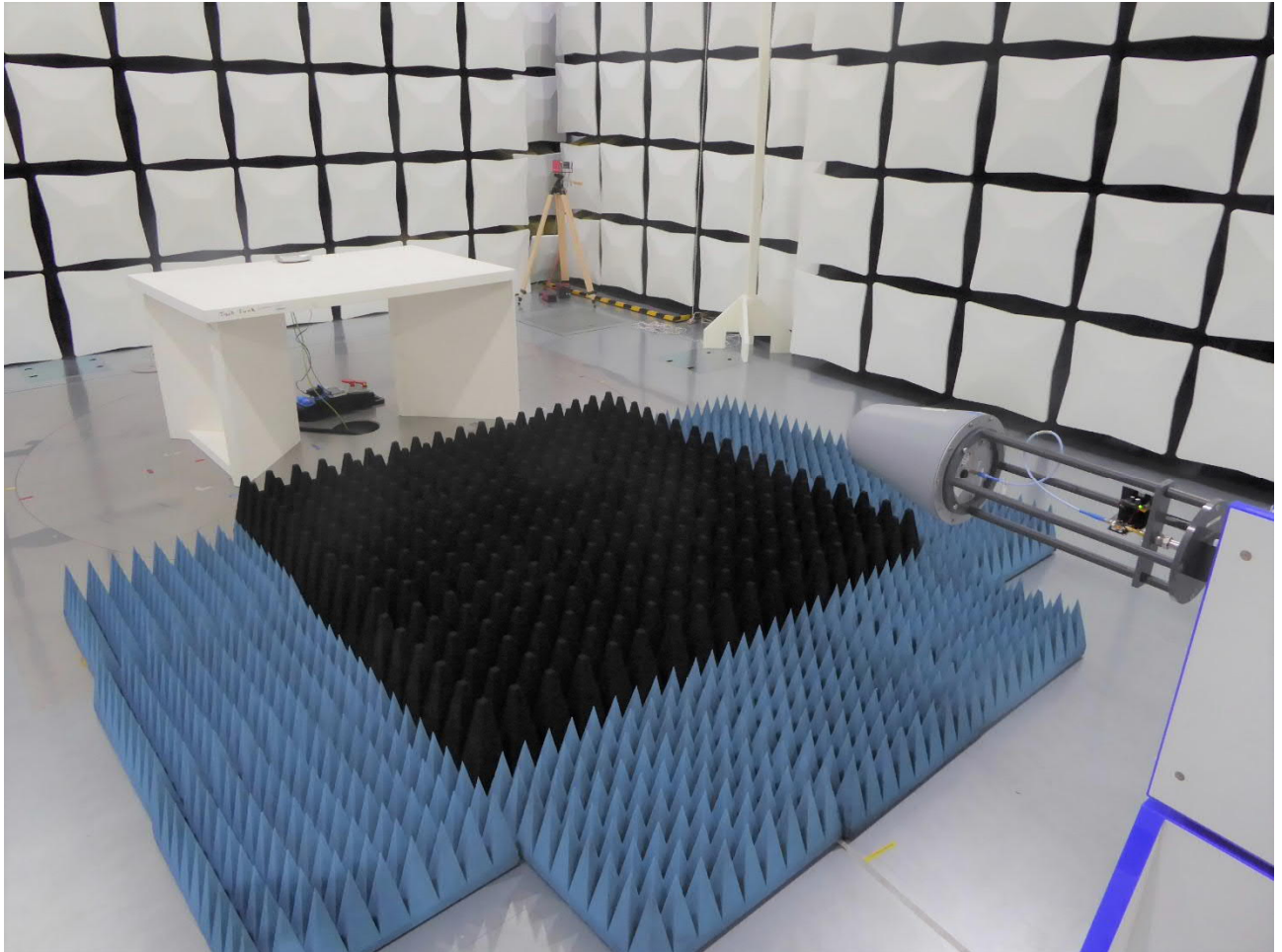
Test setup semi anechoic chamber with ground absorbers
