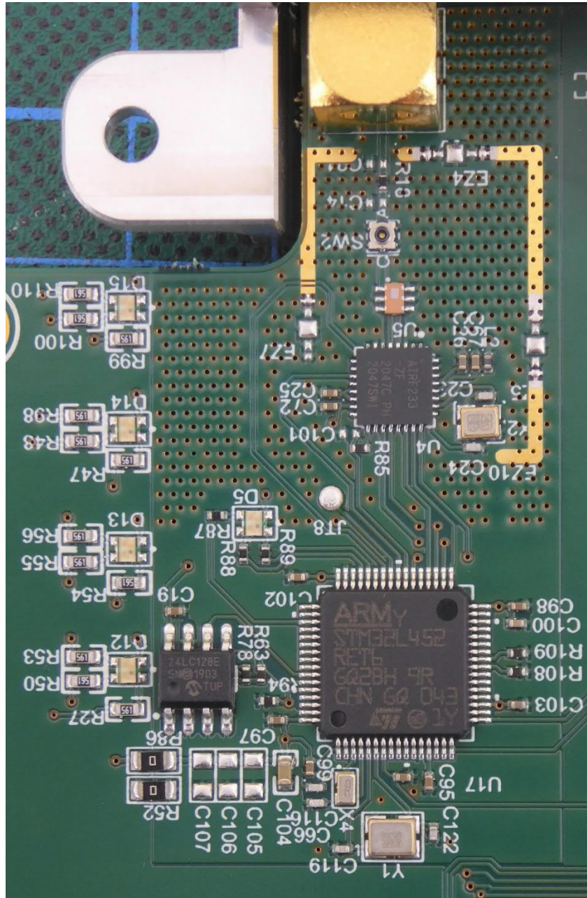
Radio part – PCB 2
