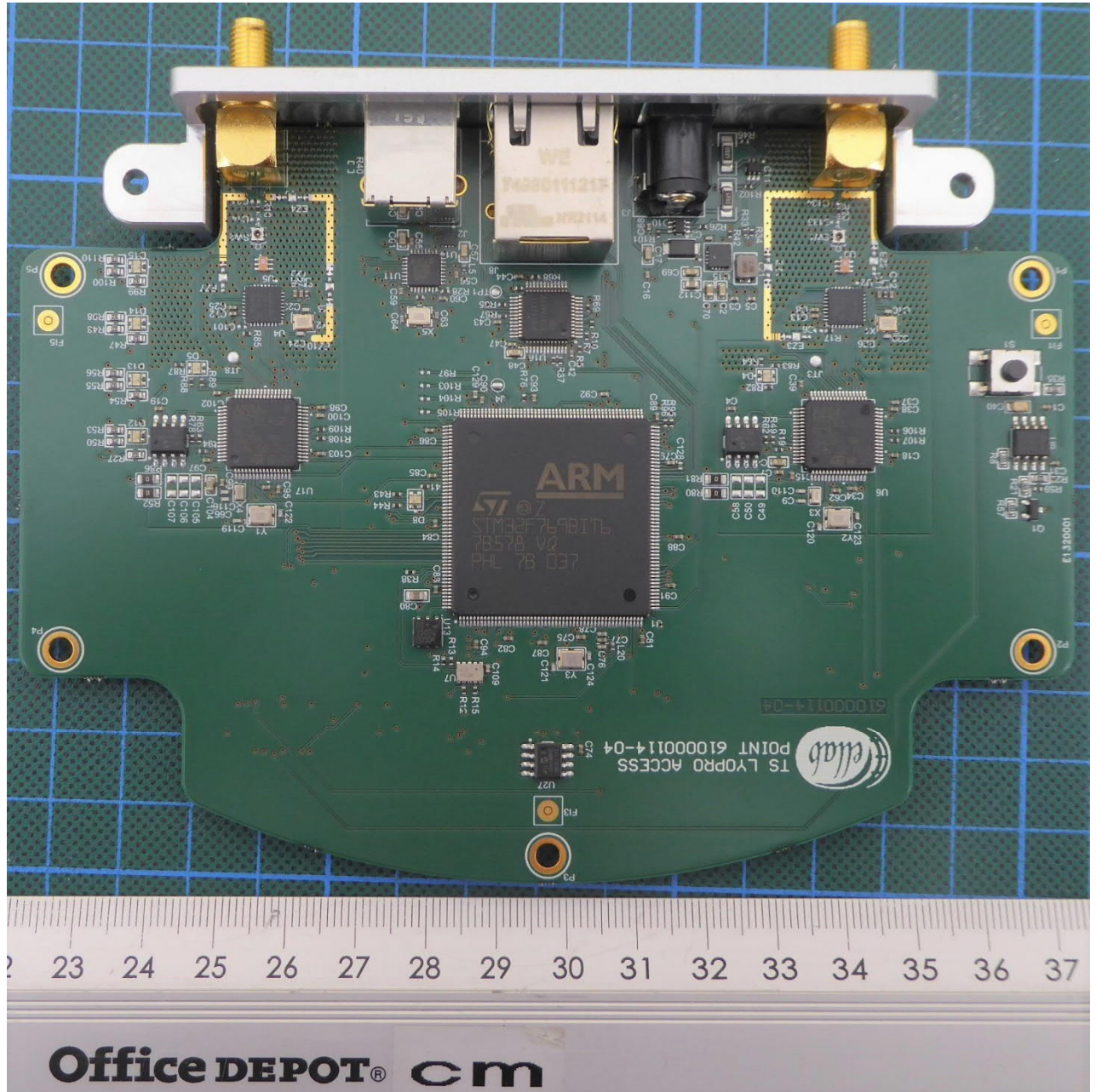
Main PCB – top view
