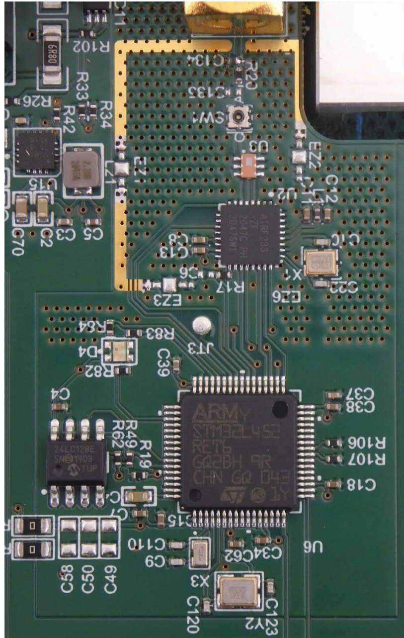
Radio part – PCB 1
