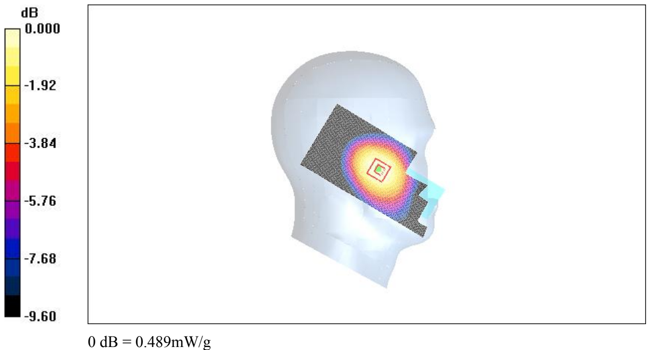
Fig.5 850 MHz CH251
