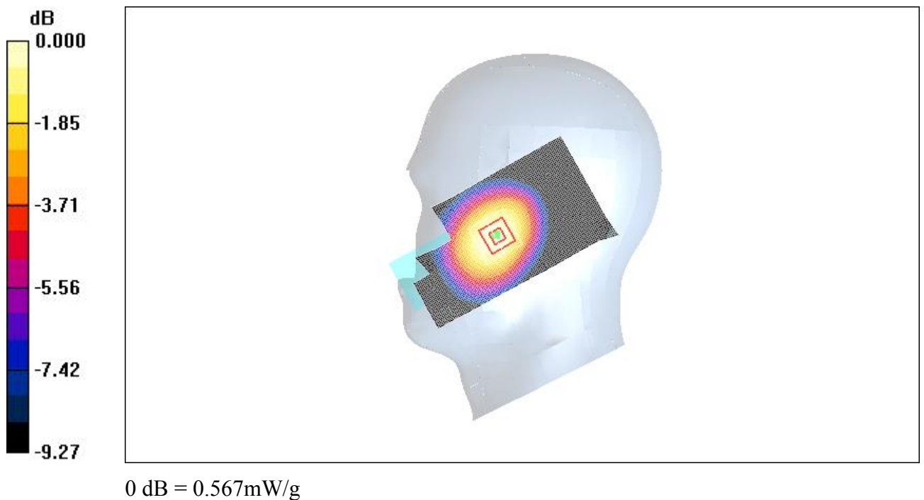
Fig.11 850 MHz CH251
