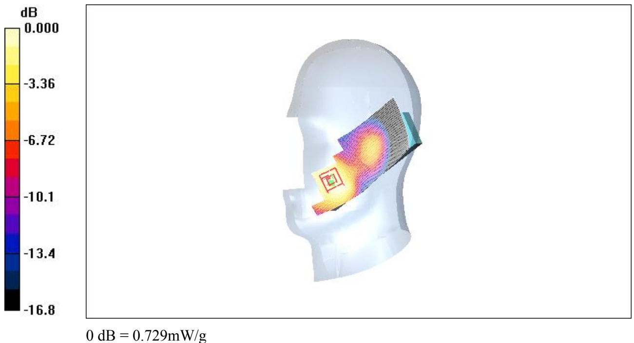
Fig. 27 1900 MHz CH661
