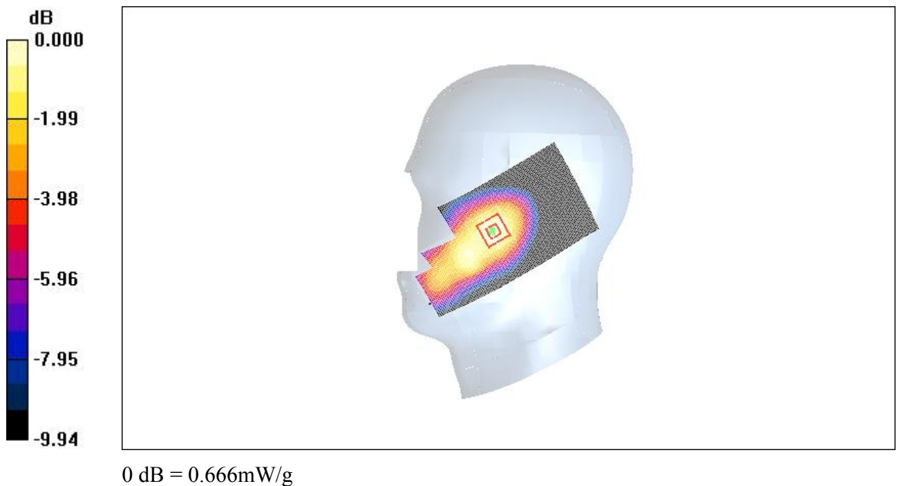
Fig. 9 850 MHz CH128
