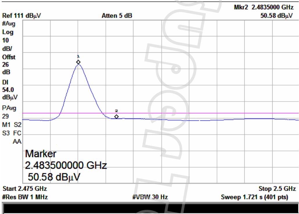
(Plot 21: Channel = 78, Detector Mode: Average, Polarity: Vertical)
