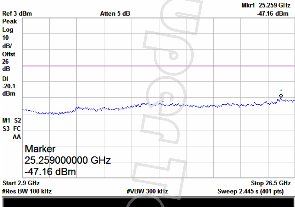
(Plot 13: Channel = 78, 3GHz to 26.5GHz)
