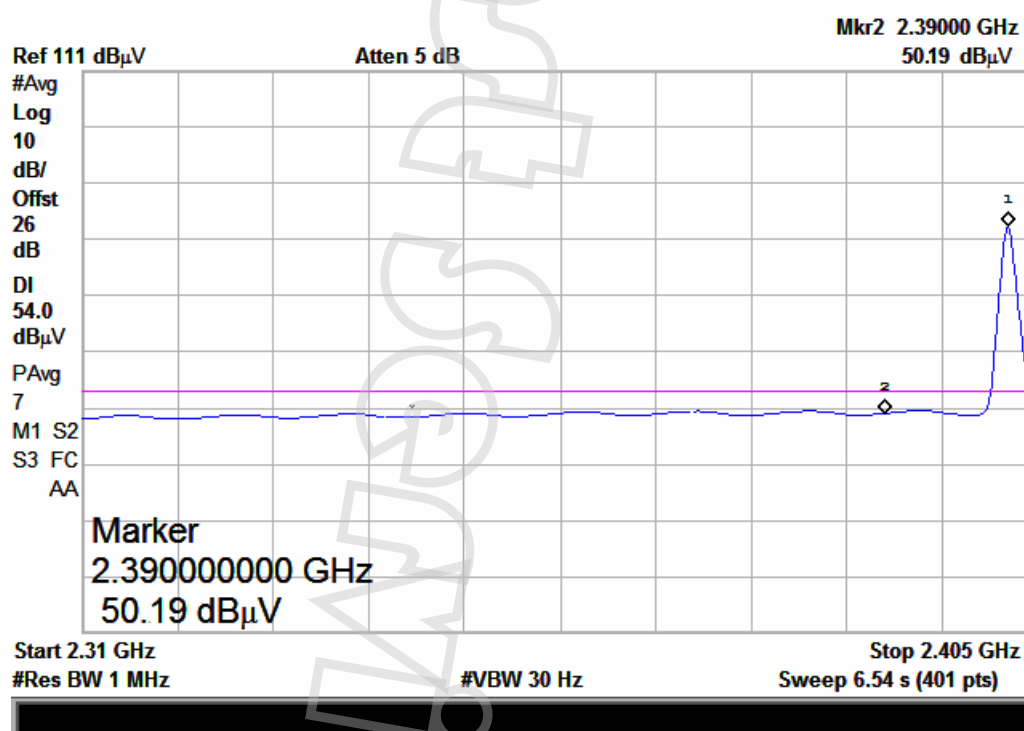
(Plot 18: Channel = 0, Detector Mode: Average, Polarity: Horizontal)
