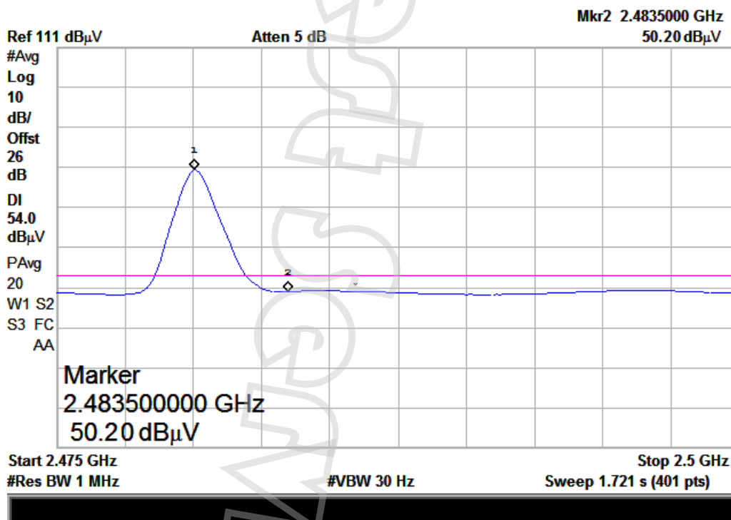
(Plot 20: Channel = 78, Detector Mode: Average, Polarity: Horizontal)
