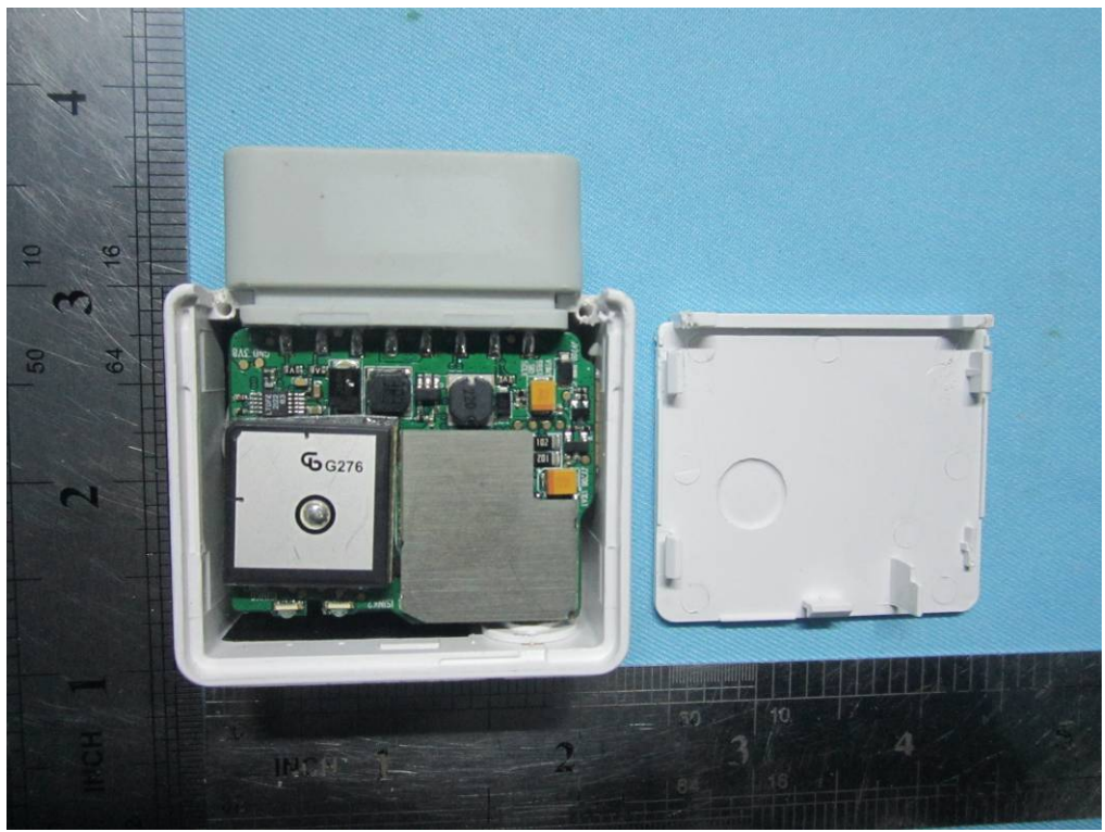
Cover Off - Front View
