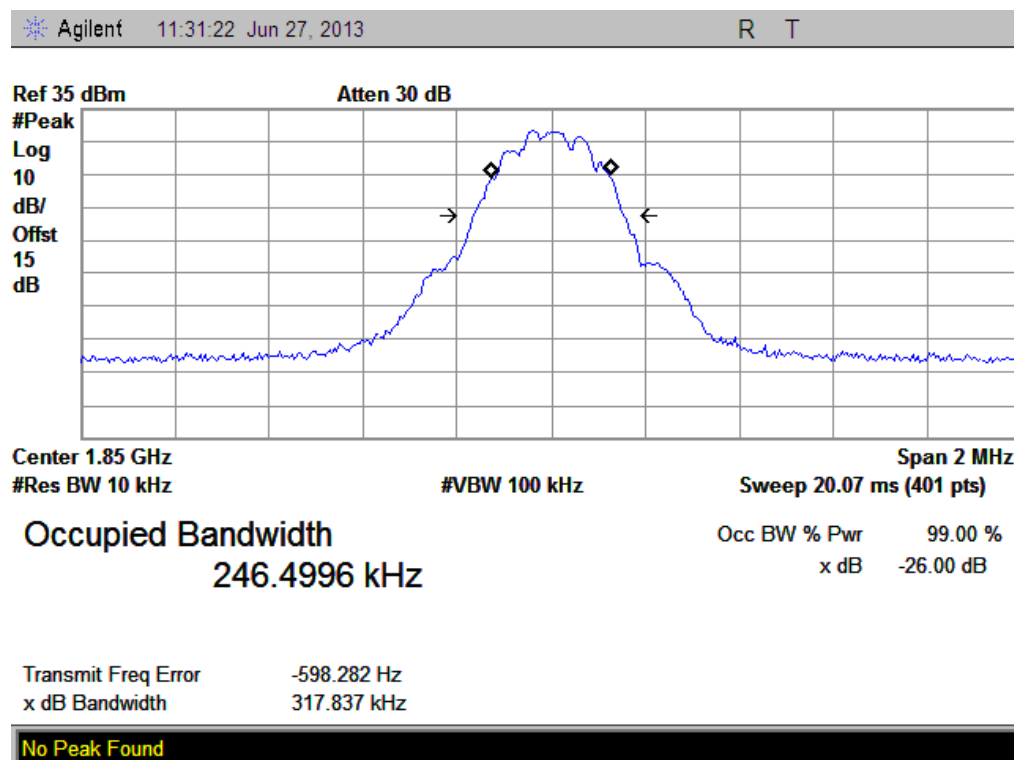
(Plot D: GPRS1900MHz Channel = 512)
