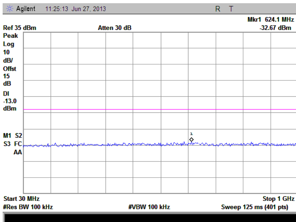
(Plot B3: GPRS1900MHz Channel = 810, 30MHz to 1GHz)
