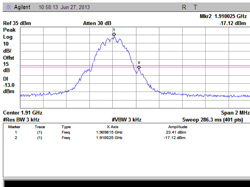
(Plot D: GPRS 1900 Channel = 810)
