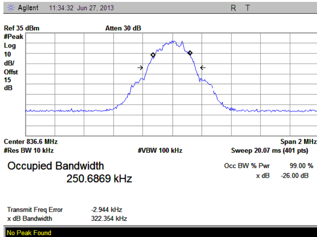
(Plot B: GPRS 850MHz Channel = 190)
