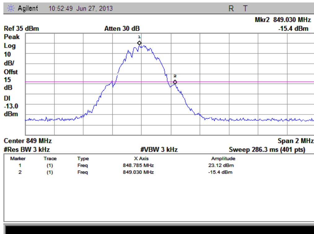
(Plot B: GPRS 850 Channel = 251)
