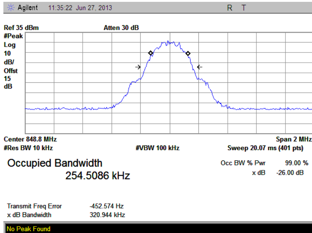
(Plot C: GPRS 850MHz Channel = 251)
