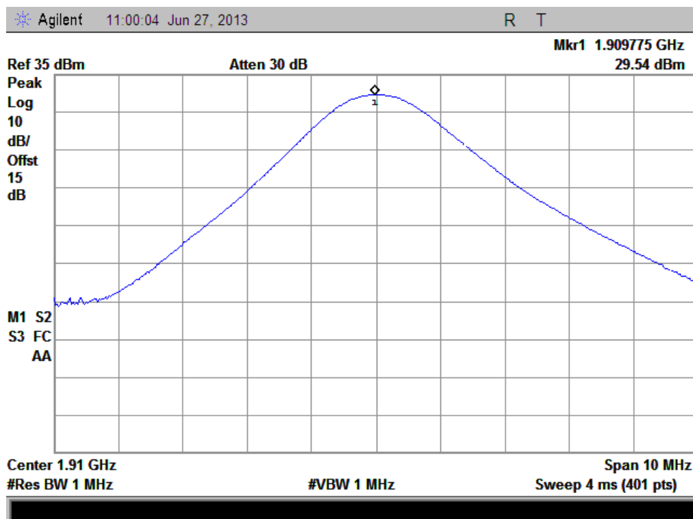
(Plot B3: GPRS 1900Hz Channel = 810)
