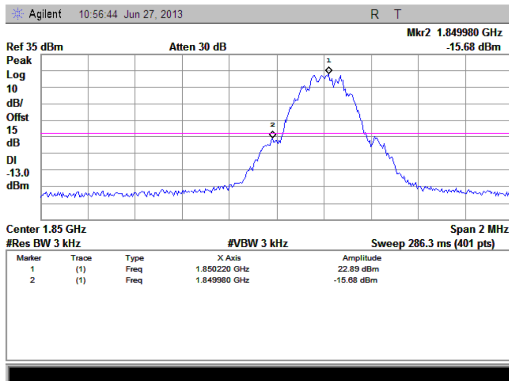
(Plot C: GPRS 1900 Channel = 512)
