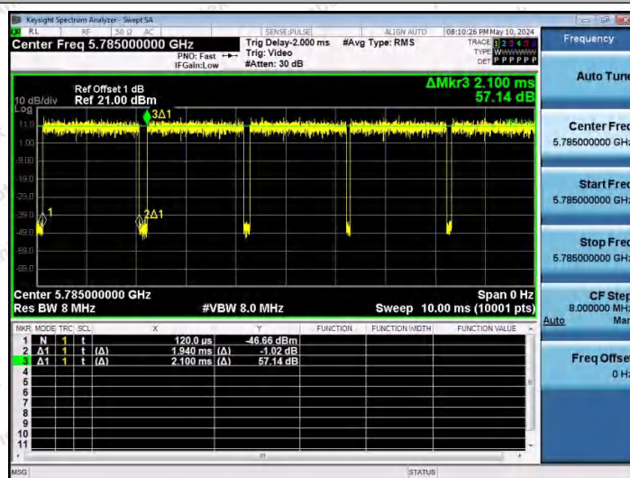
NTNV-11AC20SISO-Ant1-5785
