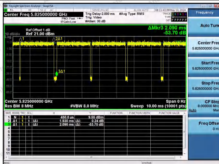
NTNV-11AC20SISO-Ant1-5825
