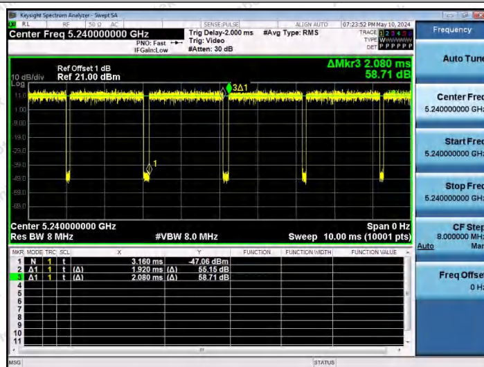
NTVN-11N20SISO-Ant1-5240
