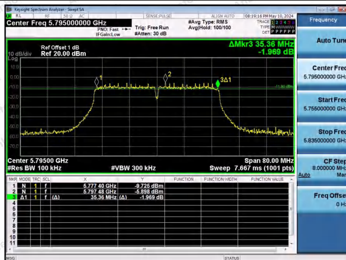
11AC40SISO-Ant1-5795-PASS
