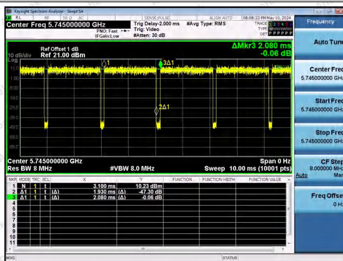
NTNV-11AC20SISO-Ant1-5745
