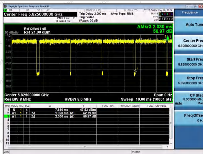
NTNV-11N20SISO-Ant1-5825
