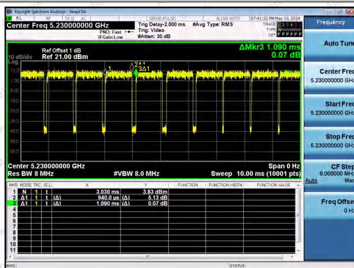
NTVN-11N40SISO-Ant1-5230
