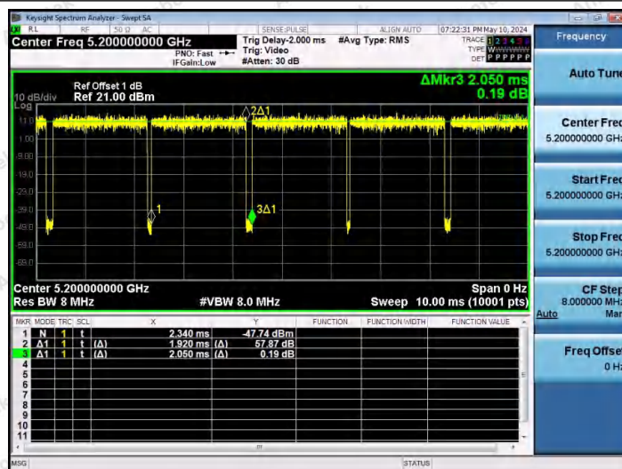
NTVN-11N20SISO-Ant1-5200
