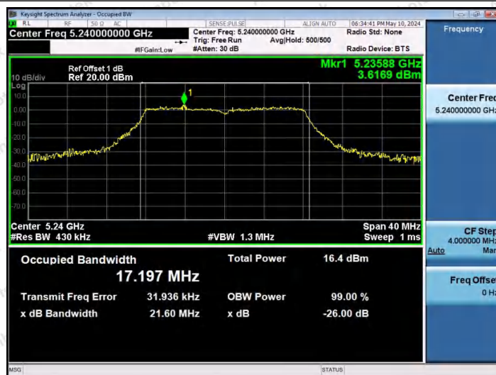
11A-Ant1-5240
