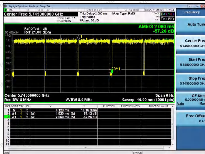
NTNV-11N20SISO-Ant1-5745
