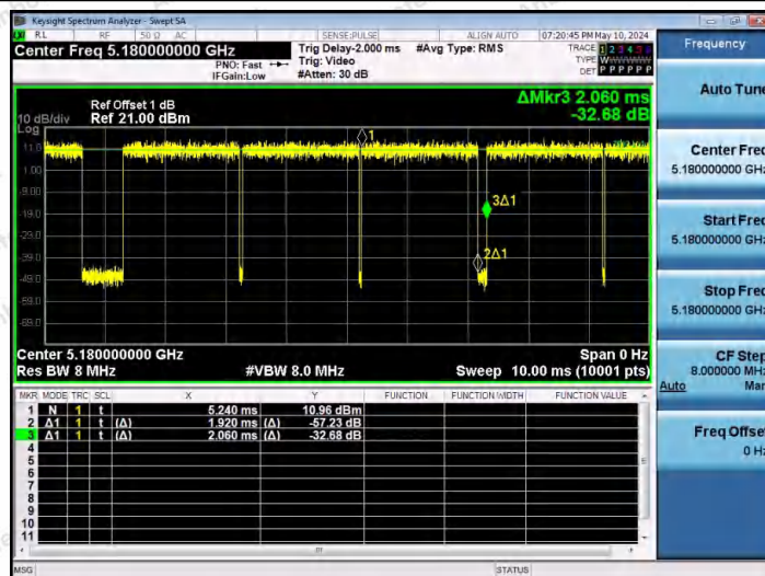
NTVN-11N20SISO-Ant1-5180
