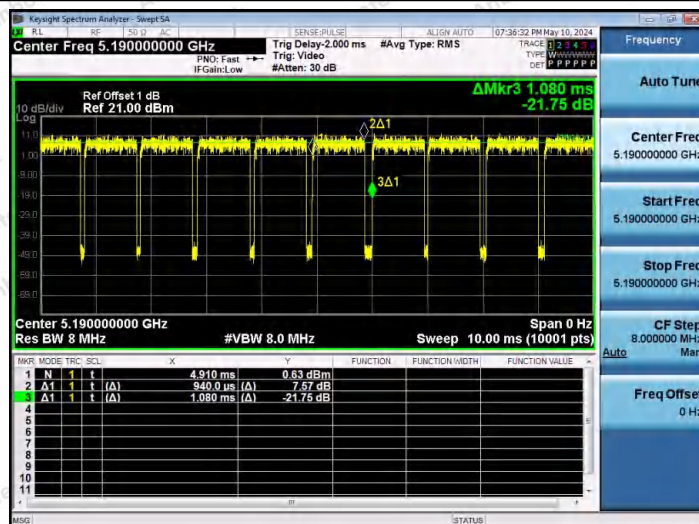
NTVN-11N40SISO-Ant1-5190
