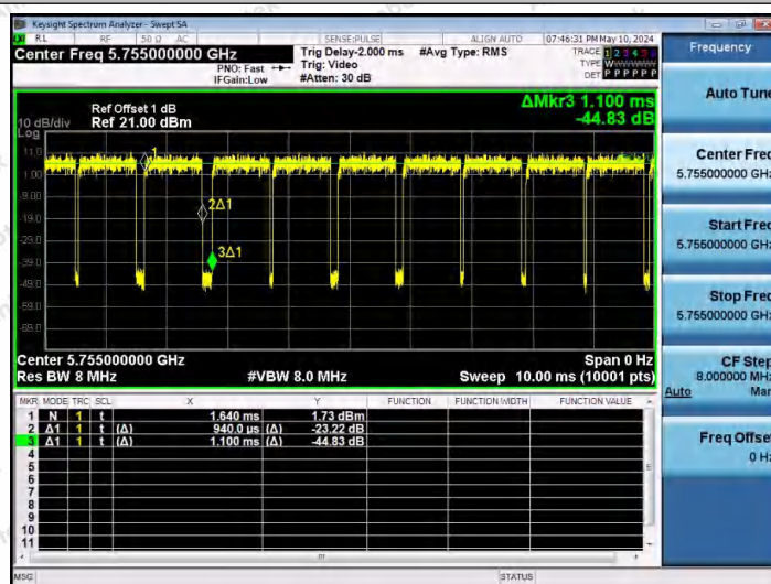
NTVN-11N40SISO-Ant1-5755
