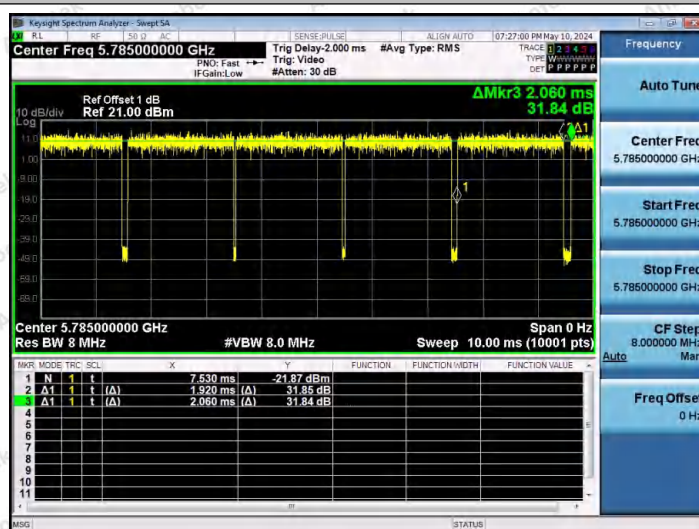
NTNV-11N20SISO-Ant1-5785
