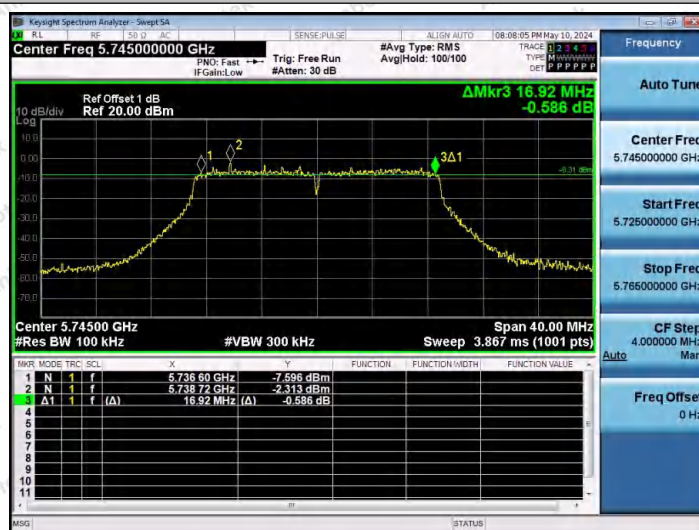
11AC20SISO-Ant1-5745-PASS
