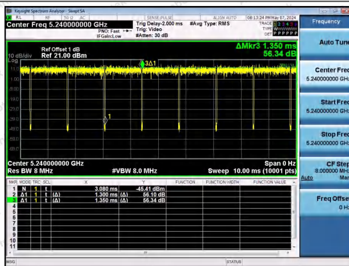
NTNV-11N20SISO-Ant1-5240
