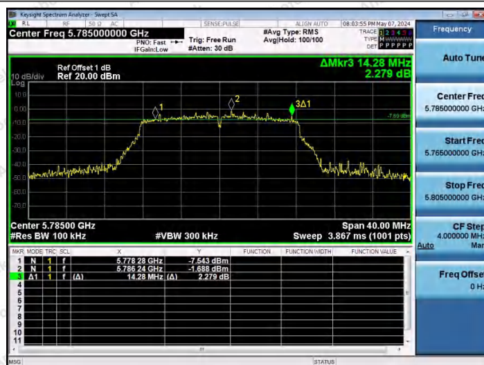
11A-Ant1-5785-PASS
