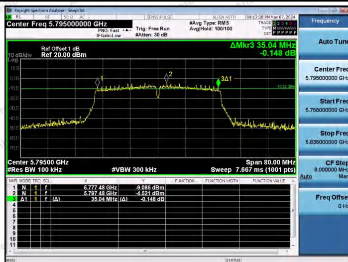
11AC40SISO-Ant1-5795-PASS
