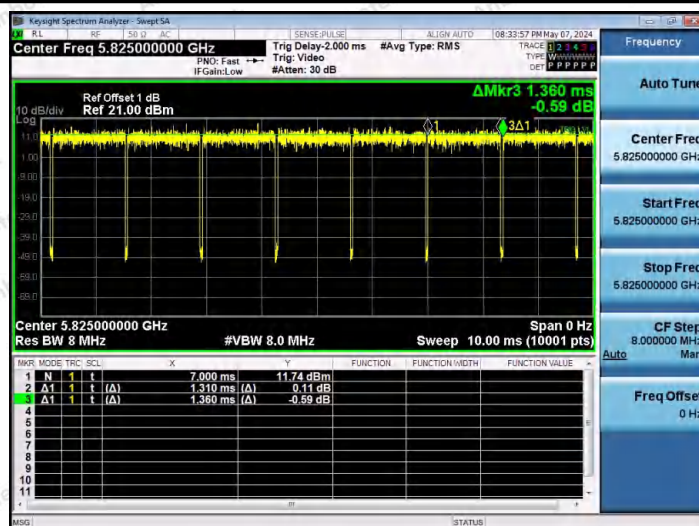
NTNV-11AC20SISO-Ant1-5825
