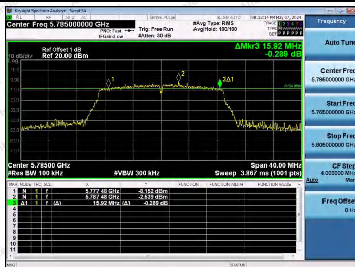
11AC20SISO-Ant1-5785-PASS
