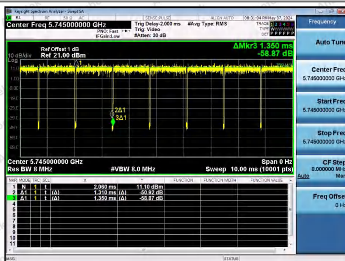
NTNV-11AC20SISO-Ant1-5745
