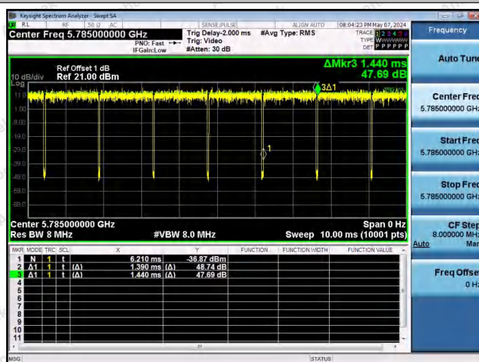
NTNV-11A-Ant1-5785
