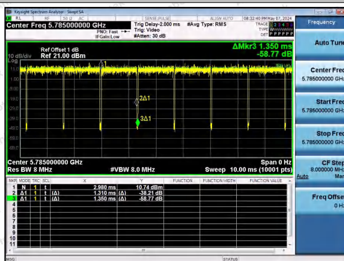
NTNV-11AC20SISO-Ant1-5785
