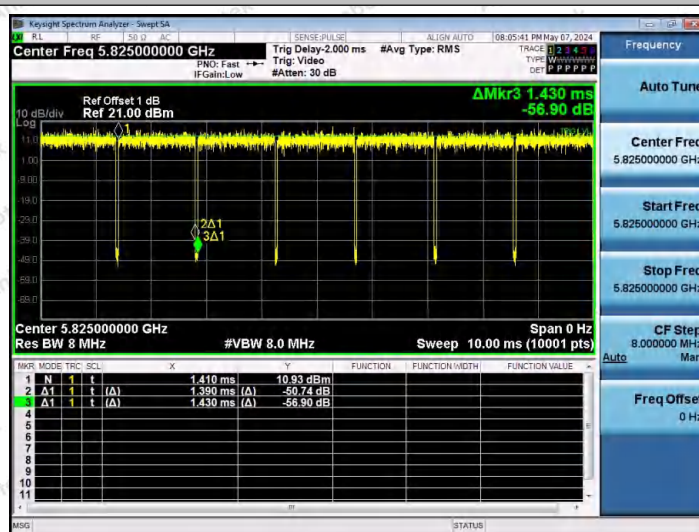
NTNV-11A-Ant1-5825
