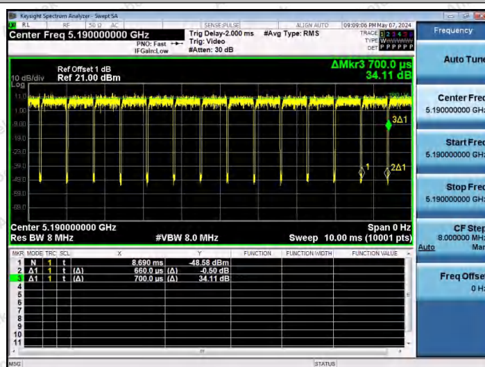
NTNV-11AC40SISO-Ant1-5190
