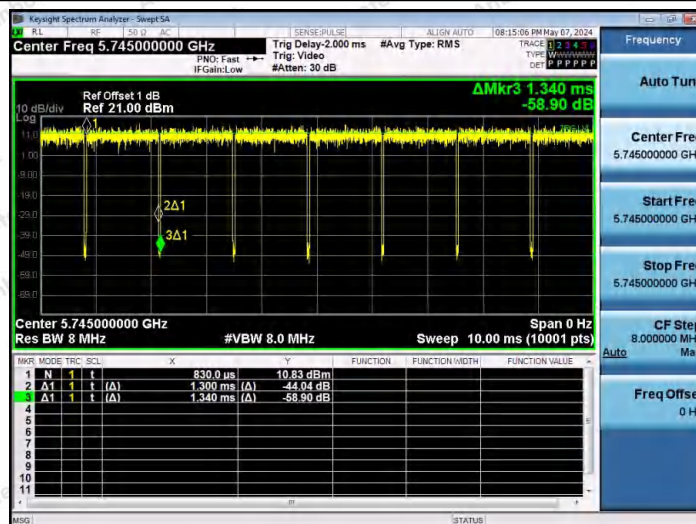
NTNV-11N20SISO-Ant1-5745
