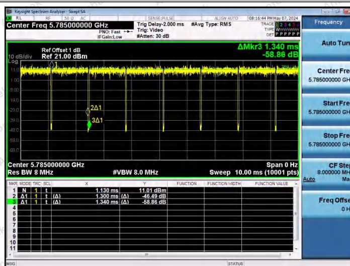
NTNV-11N20SISO-Ant1-5785
