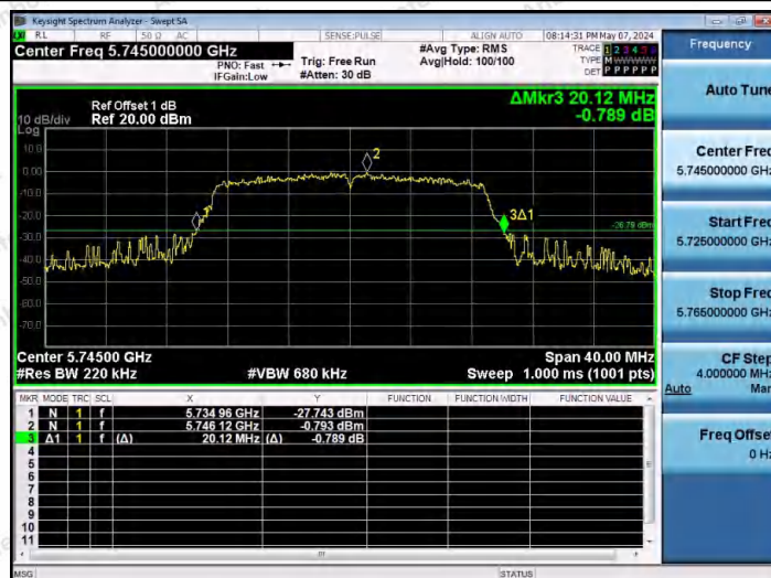
11N20SISO-Ant1-5745
