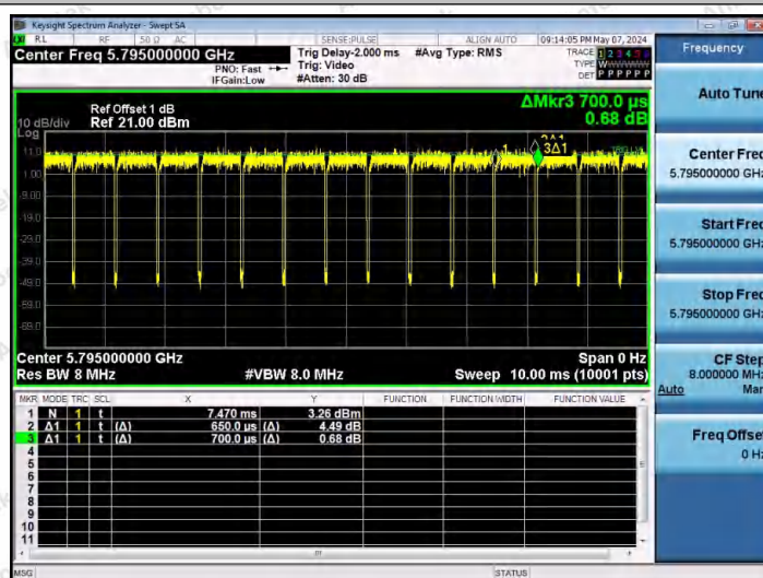
NTNV-11AC40SISO-Ant1-5795
