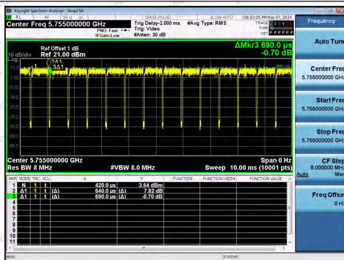
NTNV-11N40SISO-Ant1-5755
