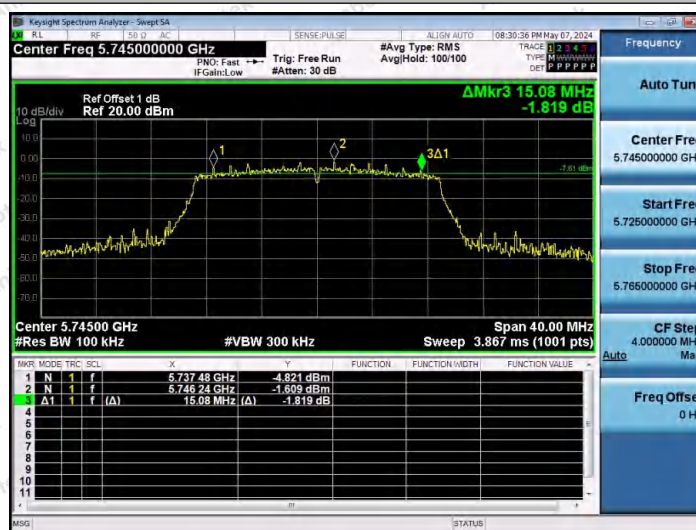
11AC20SISO-Ant1-5745-PASS
