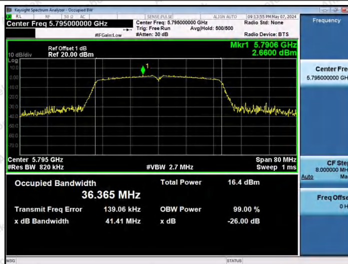
11AC40SISO-Ant1-5795
