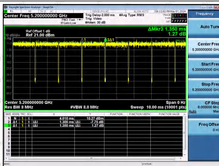
NTNV-11N20SISO-Ant1-5200
