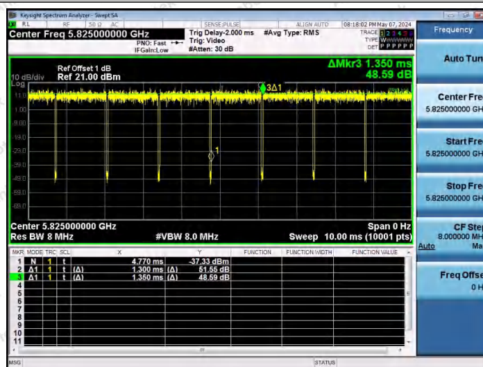
NTNV-11N20SISO-Ant1-5825
