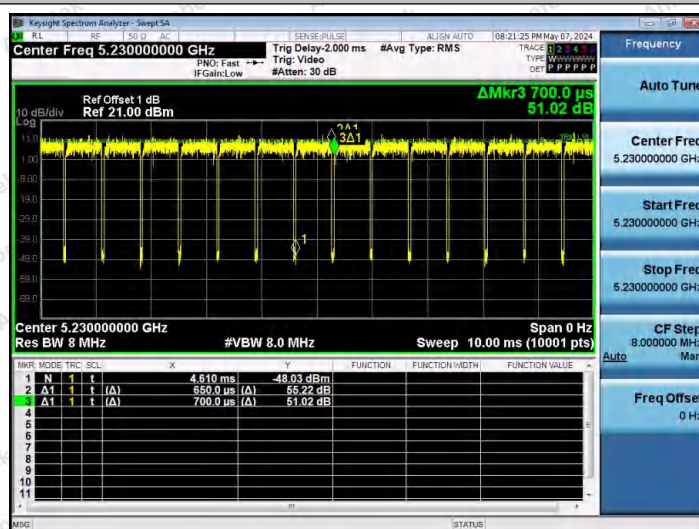
NTNV-11N40SISO-Ant1-5230
