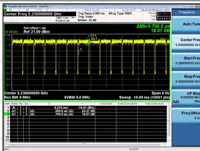
NTNV-11AC40SISO-Ant1-5230
