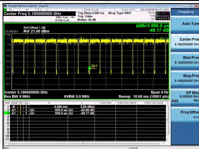
NTNV-11N40SISO-Ant1-5190
