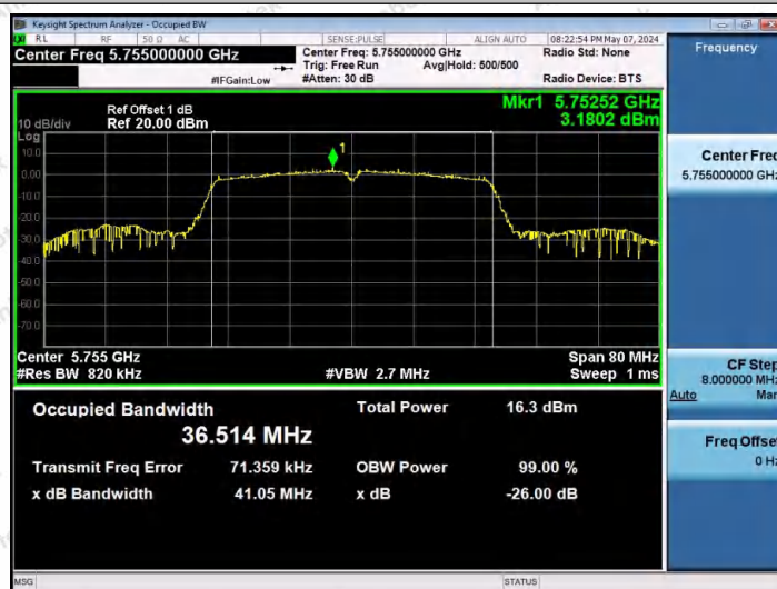
11N40SISO-Ant1-5755
