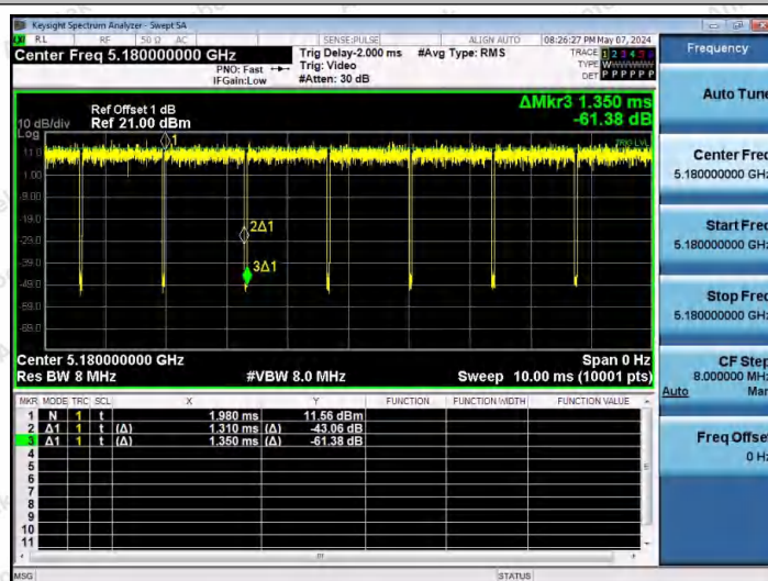
NTNV-11AC20SISO-Ant1-5180
