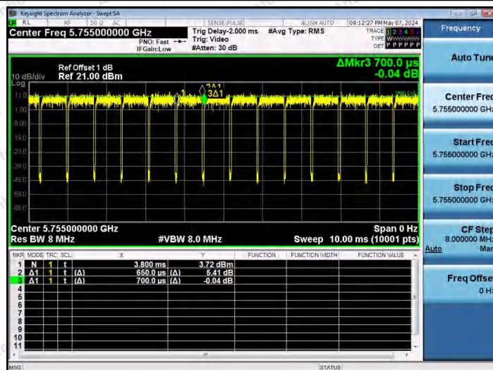
NTNV-11AC40SISO-Ant1-5755
