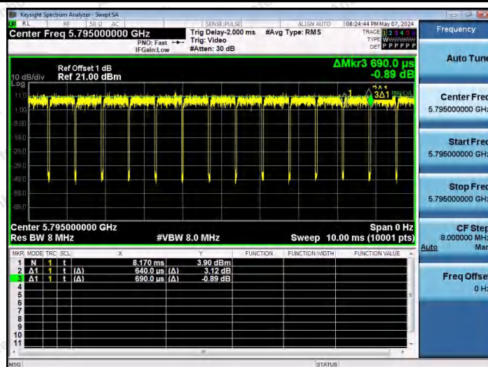
NTNV-11N40SISO-Ant1-5795
