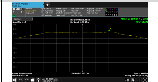
In-Band Reference Level BLE 1M_Channel 39
