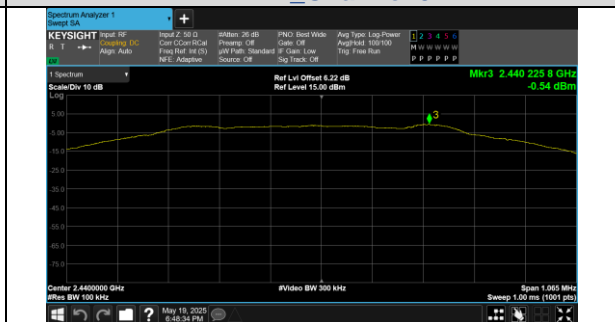
In-Band Reference Level BLE 1M_Channel 19
