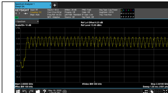
Low End Spectrum Channel Hopping Plot GFSK
