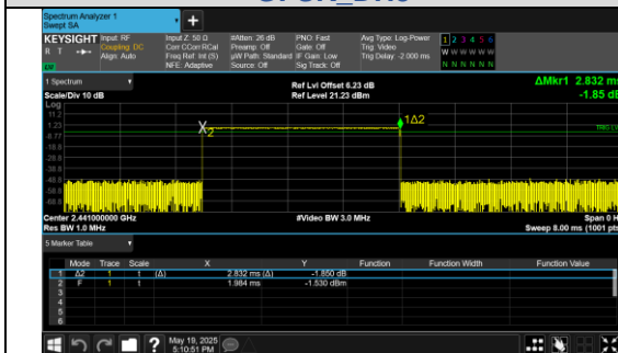
Pulse Width GFSK DH5
