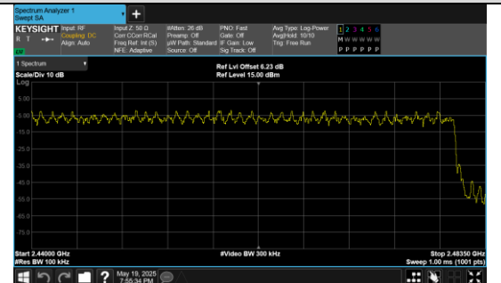
High End Spectrum Channel Hopping Plot 8DPSK
