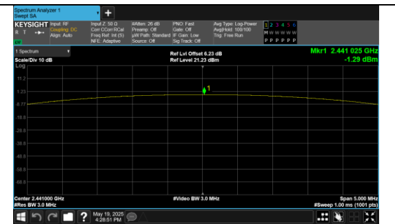
Peak Output Power GFSK_Channel 39
