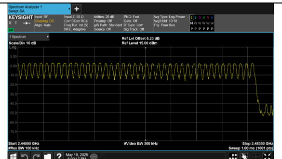
High End Spectrum Channel Hopping Plot GFSK
