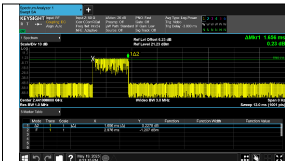
Pulse Width 8DPSK_3-DH3
