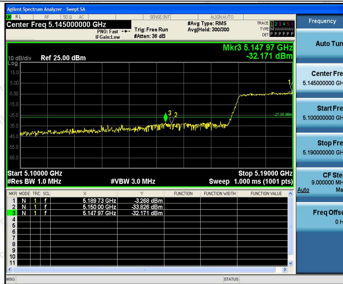
11AC80SISO_Ant1_High_5210
