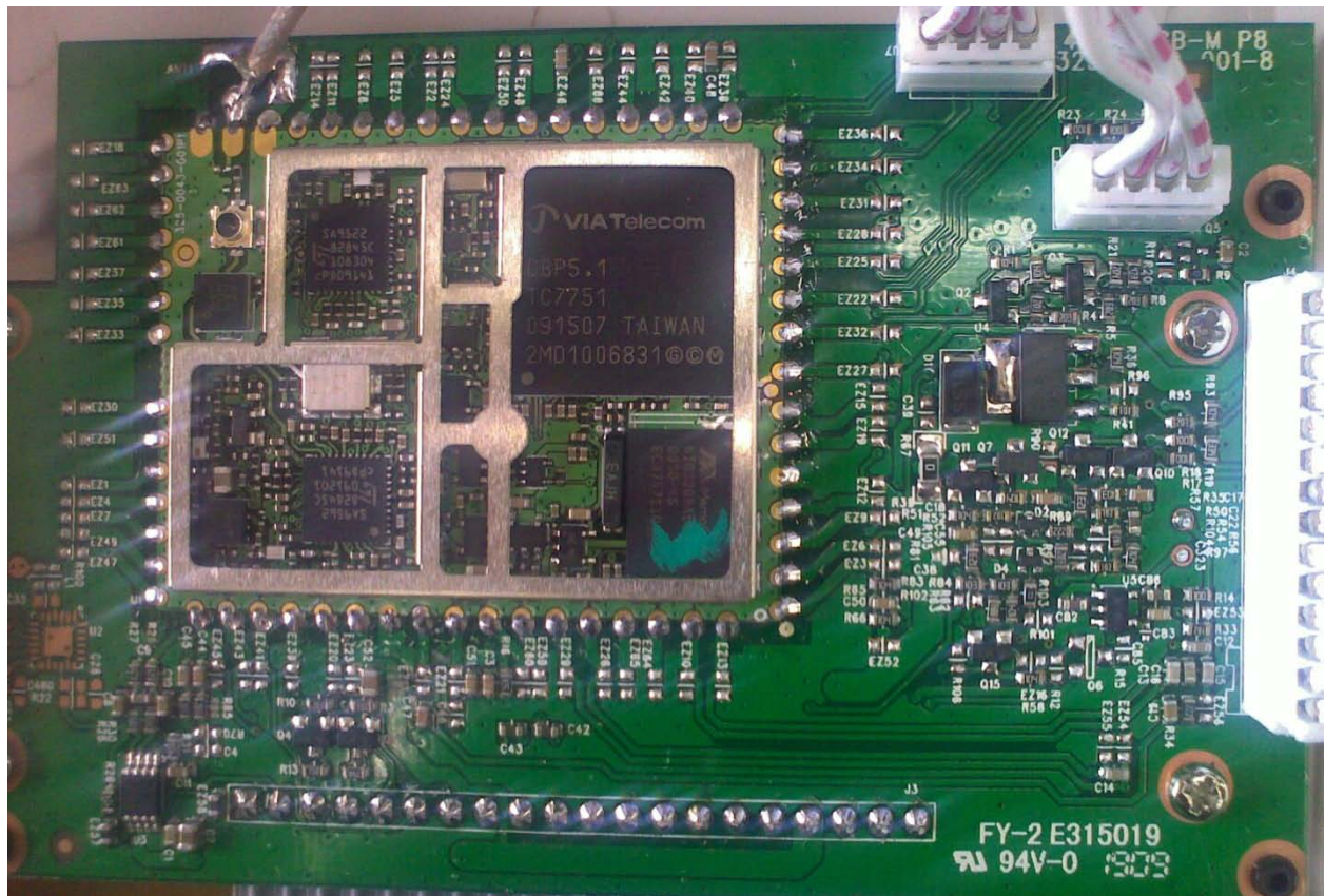
Top of RF board w/o Shield
