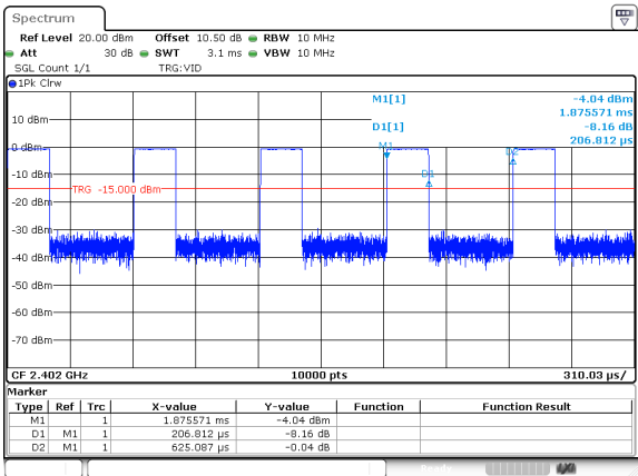
BLE_2M_Low_Channel
