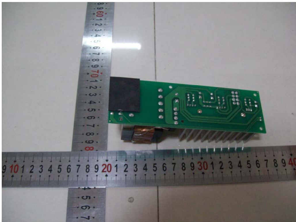
INTERNAL PHOTO OF SAMPLE-TX-4
