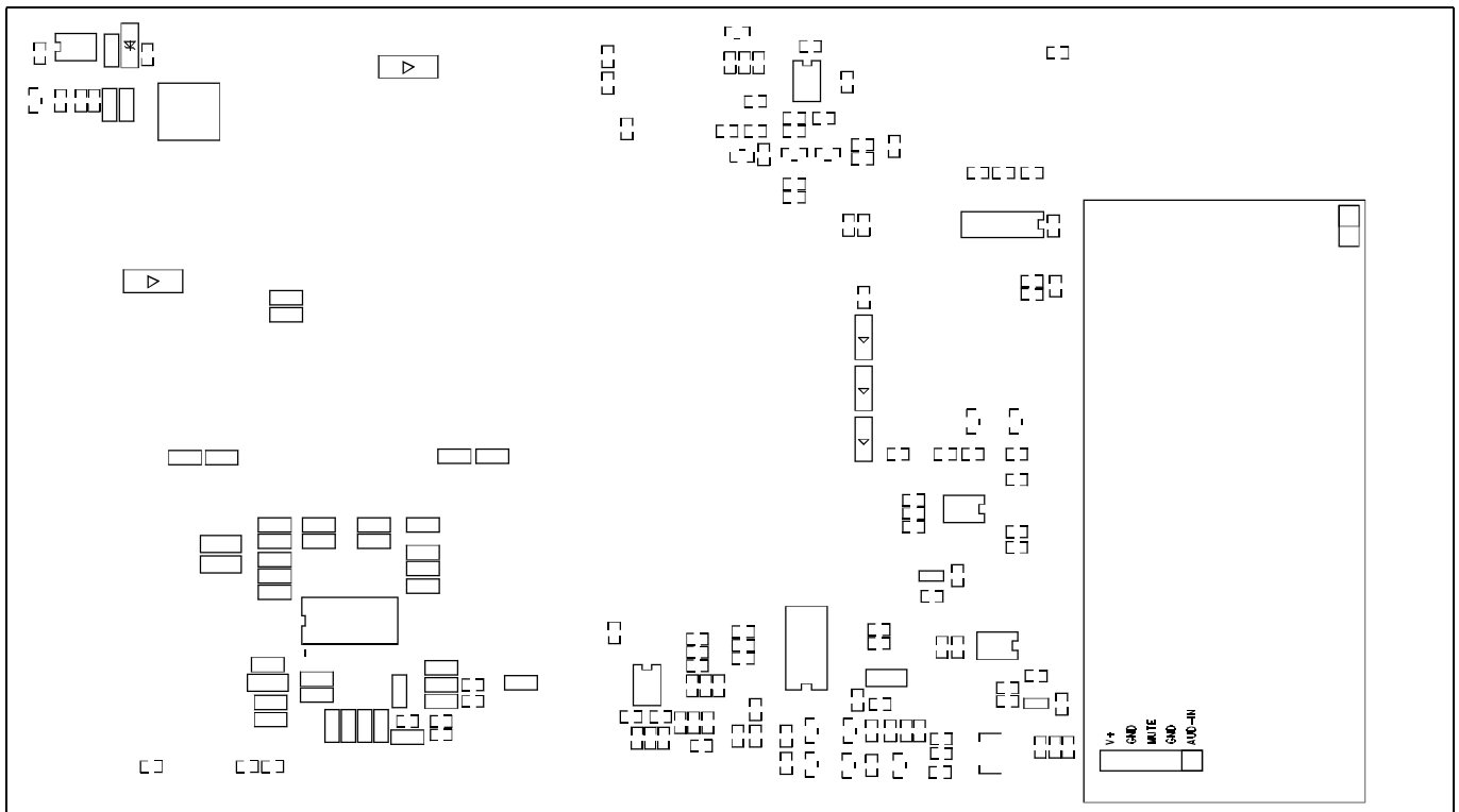
SILKSCREEN (BOTTOM)
