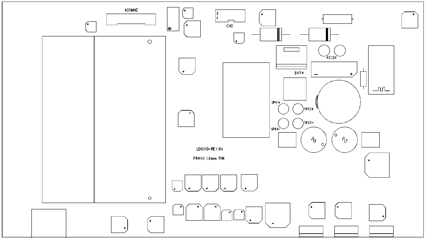
SILKSCREEN (TOP)
