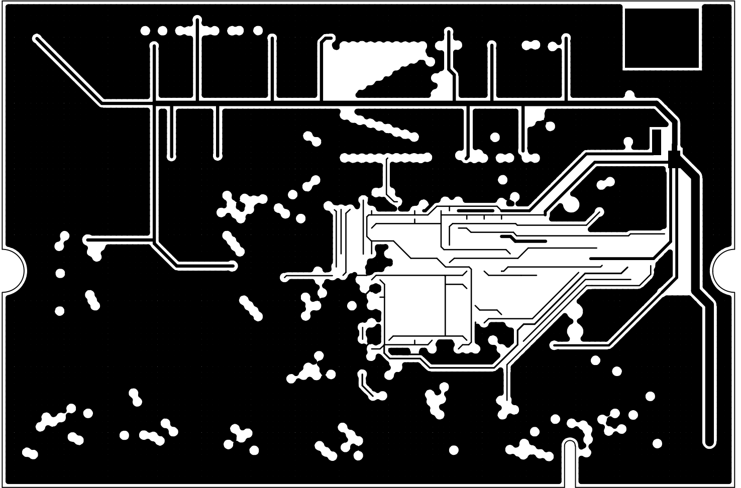
Midlayer 1
