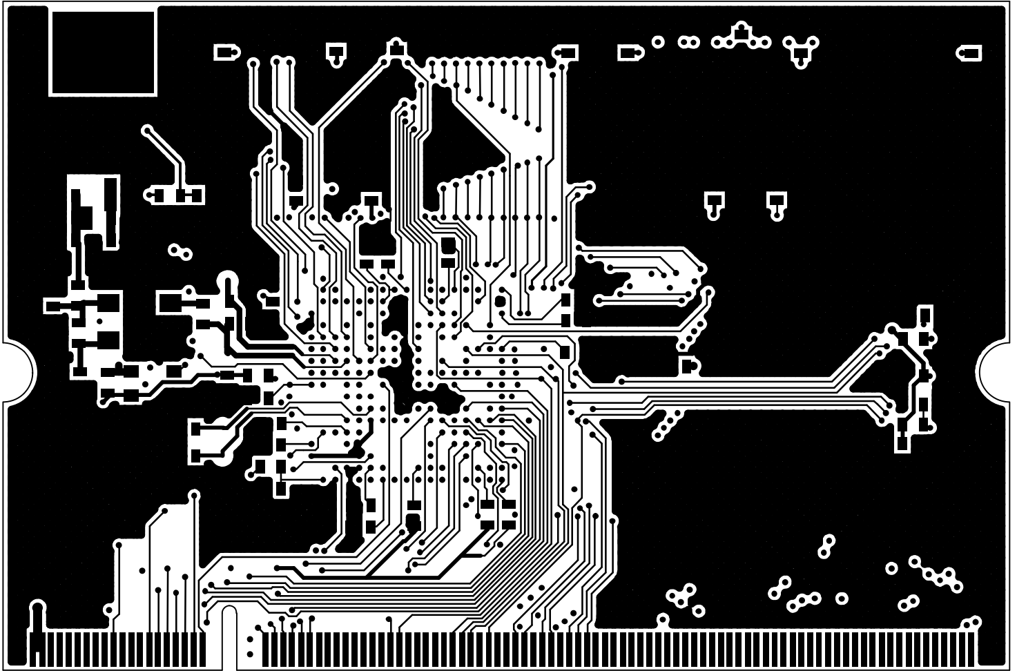
BottomLayer
