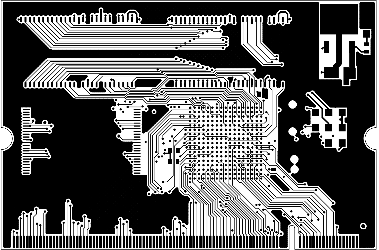
TopLayer
