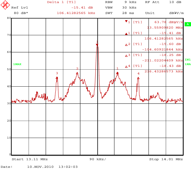
Figure 1. Plot of the Band edge (Preliminary measurement in the anechoic chamber at 3 m distance to find out the frequencies, at which the spurious emissions occur, with the peak detector function)
