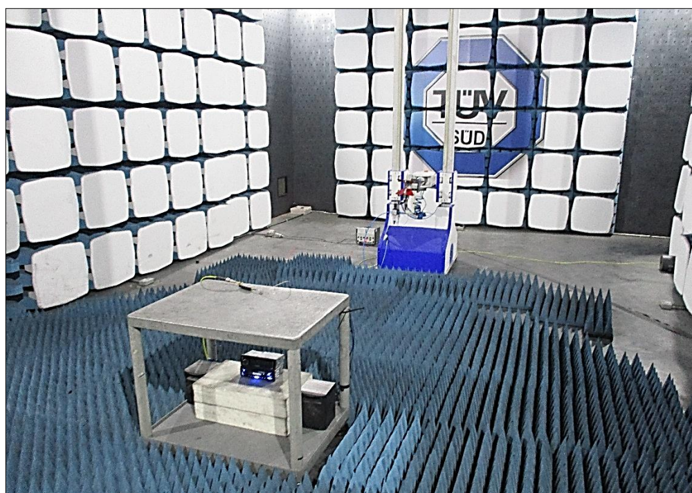
Figure 37 - Test Setup - 1 GHz to 2 GHz
