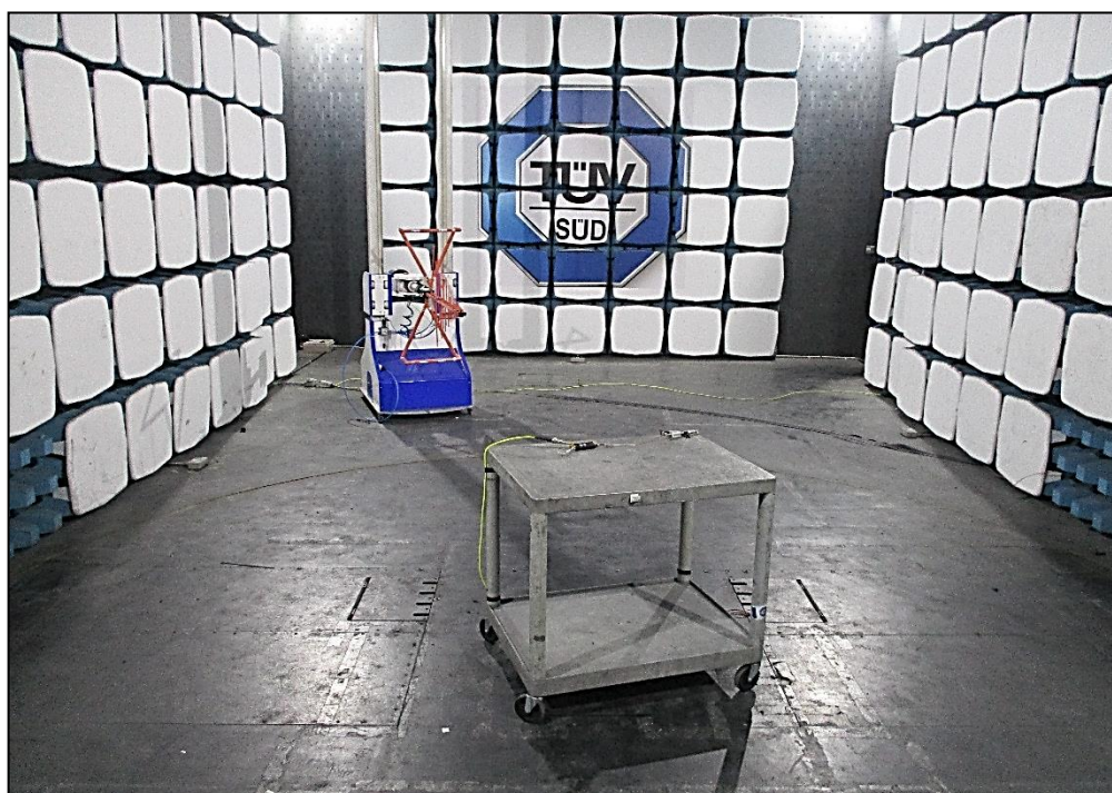
Figure 36 - Test Setup - 30 MHz to 1 GHz
