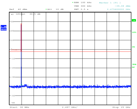
Figure 8.4-2: Conducted spurious emissions for high channel
