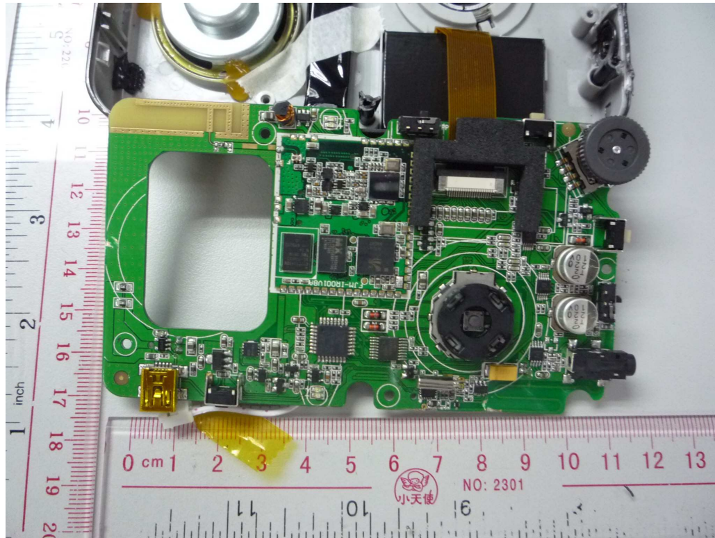
Fig. 3: Main board top view
