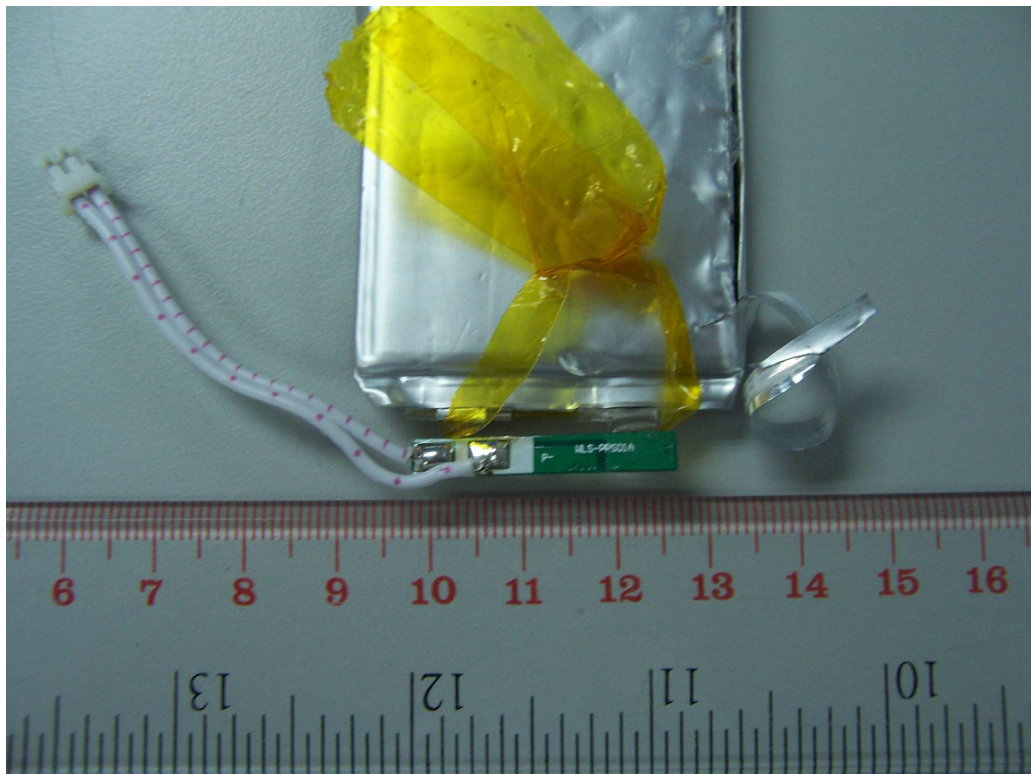
Fig. 8: Battery control board bottom view
