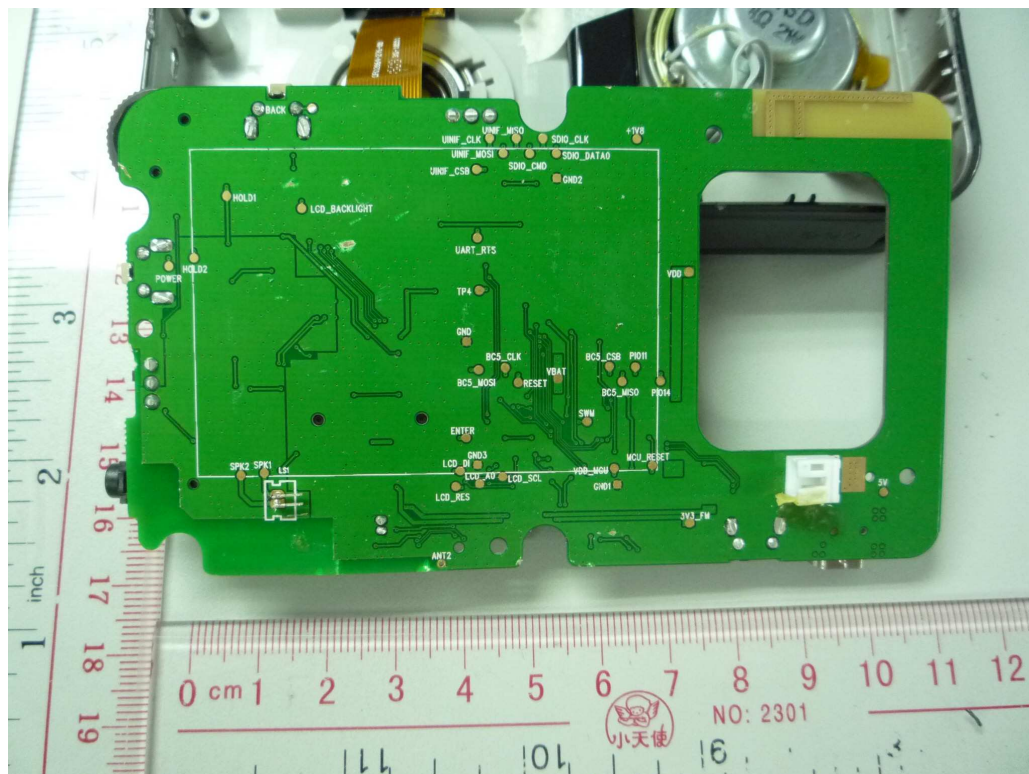
Fig. 4: Main board bottom view
