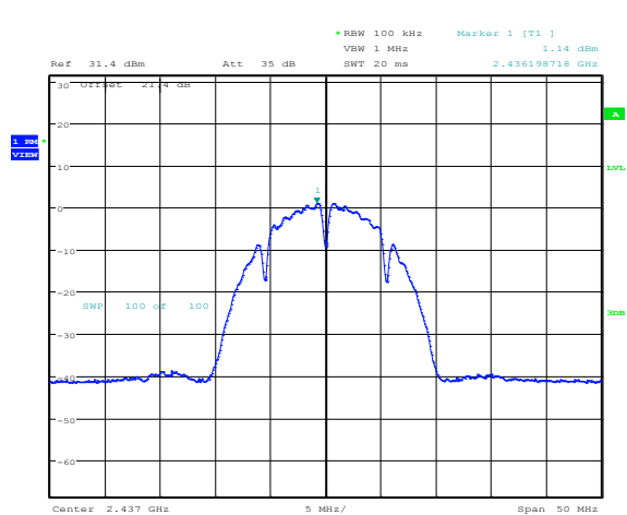
Figure 8.6-1: PSD sample plot on 802.11b
