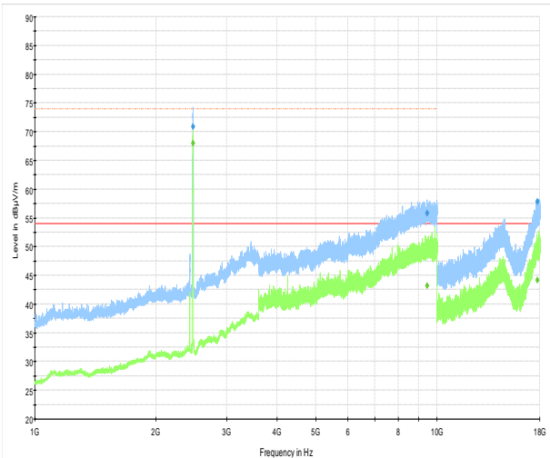
Figure 8.5-6: Radiated spurious emissions for 802.11b, Sample
