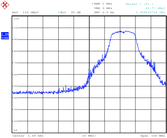
Figure 8.5-7: Radiated Spurious emissions 802.11g, Sample
