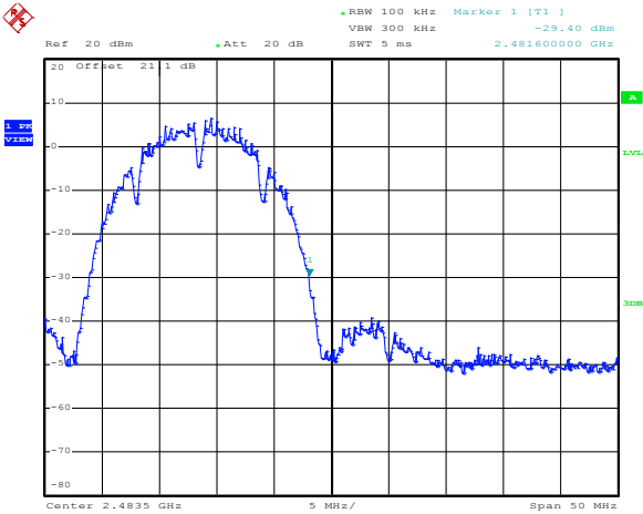
Figure 8.5-1: Conducted spurious emissions for 802.11b, Sample
