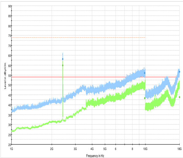
Figure 8.5-7: Radiated Spurious emissions 802.11g, Sample
