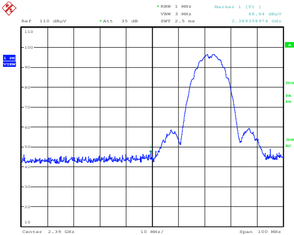
Figure 8.5-2: Conducted spurious emissions for 802.11b, Low band edge
