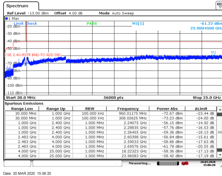
Figure 8.7-21: Conducted spurious emissions (Restricted band) for high channel
