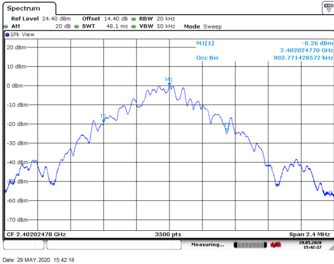
Figure 8.5-4: 99% occupied bandwidth on low channel
