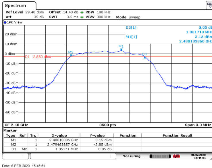
Figure 8.5-9: 6 dB bandwidth on high channel
