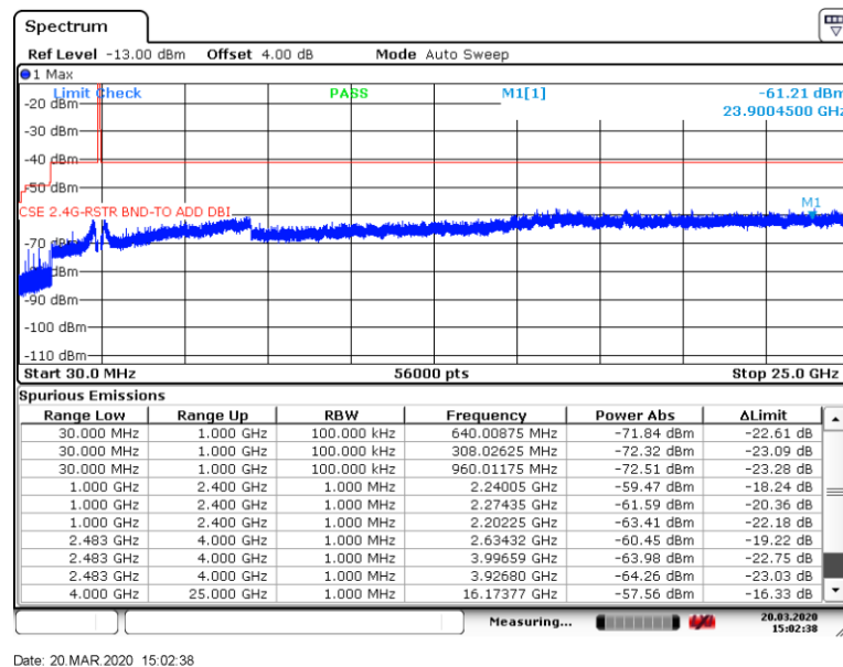
Figure 8.7-17: Conducted spurious emissions (Restricted band) for mid channel
