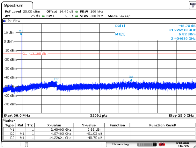
Figure 8.7-10: Conducted spurious emissions for low channel, BLE
