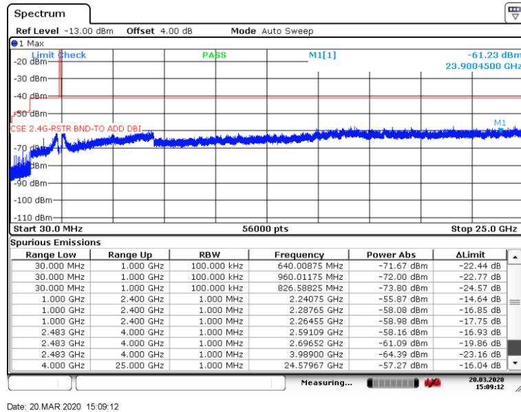
Figure 8.7-24: Conducted spurious emissions (Restricted band) for high channel
