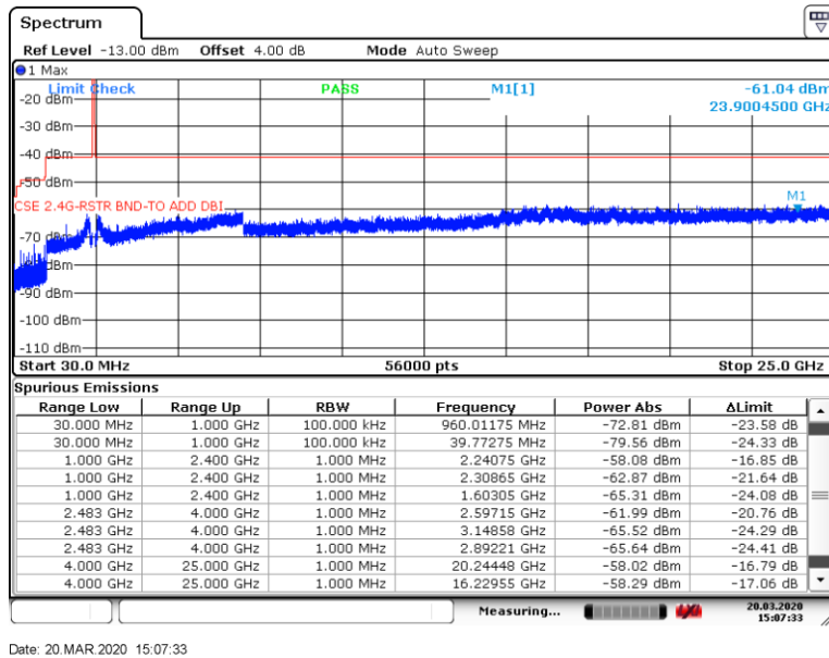
Figure 8.7-22: Conducted spurious emissions (Restricted band) for low channel
