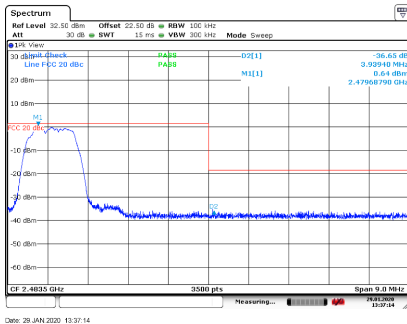
Figure 8.7-28: Band Edge emissions for high channel
