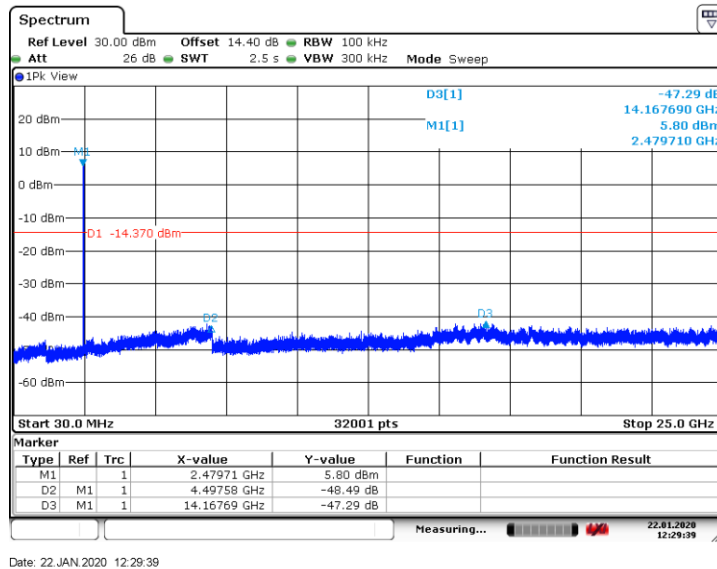
Figure 8.7-12: Conducted spurious emissions for high channel, BLE
