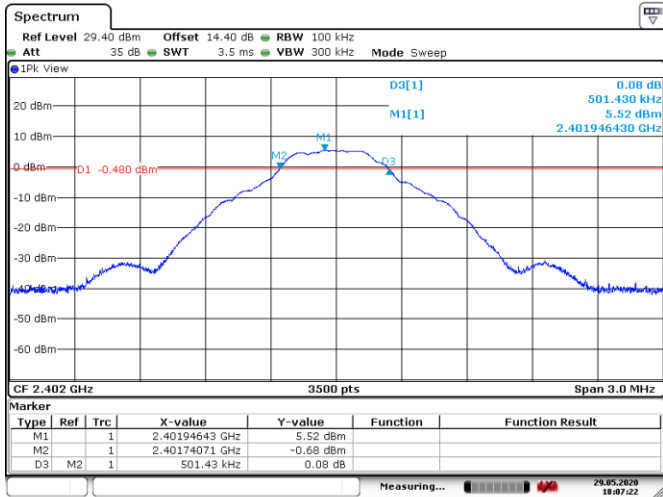
Figure 8.5-1: 6 dB bandwidth on low channel, sample plot
