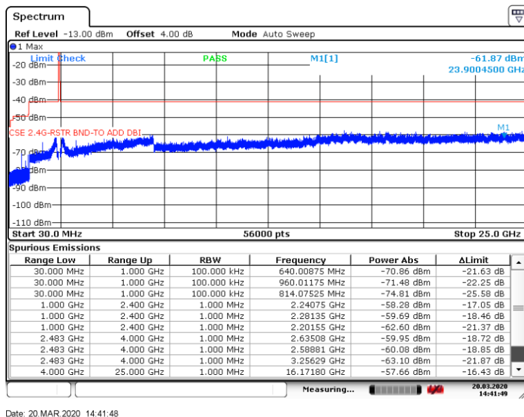
Figure 8.7-14: Conducted spurious emissions (Restricted band) for mid channel
