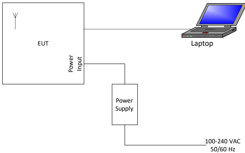
Figure 3.6-1: Setup diagram
