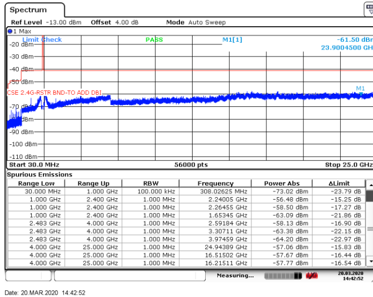
Figure 8.7-15: Conducted spurious emissions (Restricted band) for high channel
