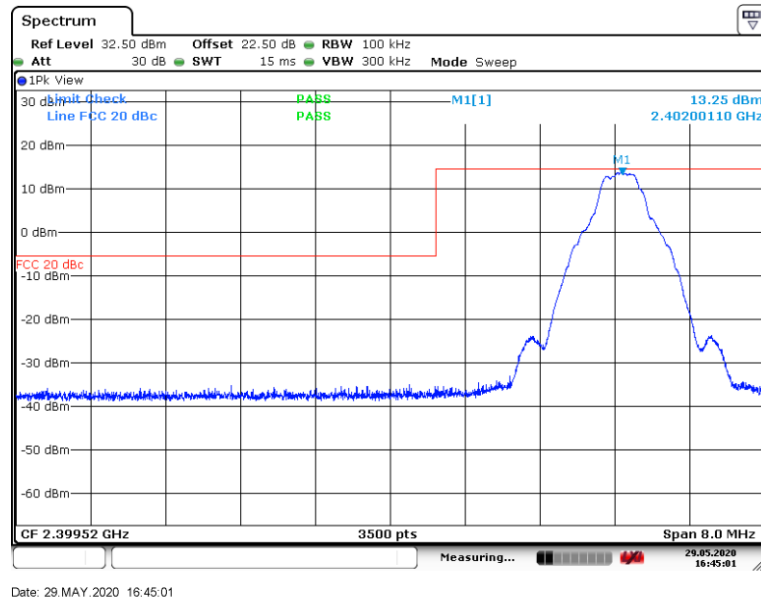
Figure 8.7-25: Band Edge emissions for low channel
