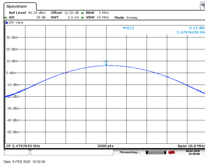
Figure 8.6-9: Output power on high channel, 8DPSK Modulation
