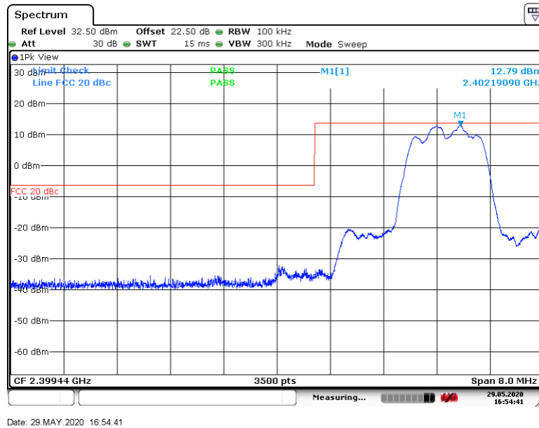
Figure 8.7-29: Band Edge emissions for low channel
