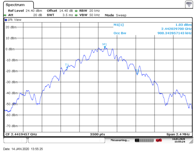
Figure 8.5-5: 99% occupied bandwidth on mid channel
