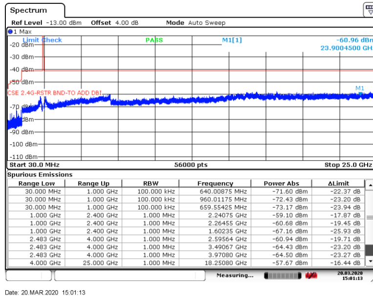
Figure 8.7-16: Conducted spurious emissions (Restricted band) for low channel
