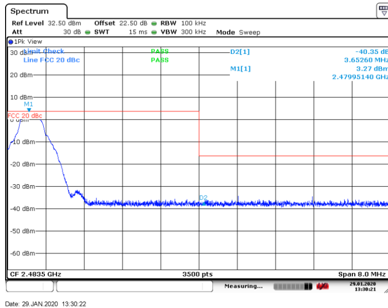
Figure 8.7-26: Band Edge emissions for high channel
