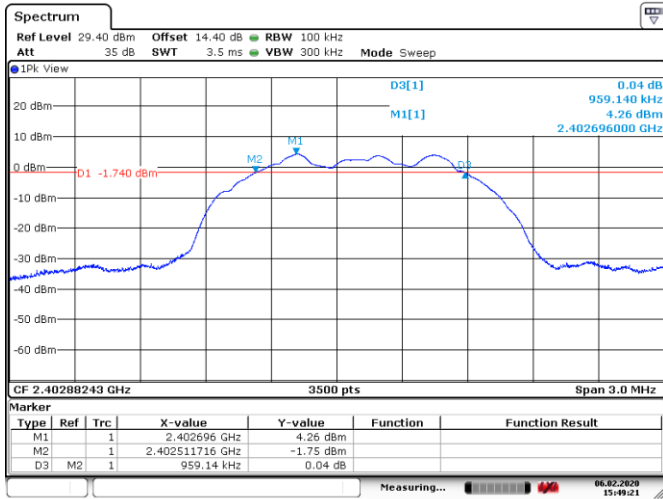
Figure 8.5-13: 6 dB bandwidth on low channel, sample plot
