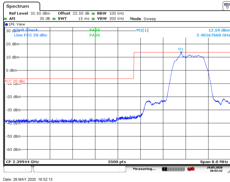
Figure 8.7-27: Band Edge emissions for low channel
