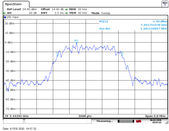
Figure 8.5-11: 99% occupied bandwidth on mid channel
