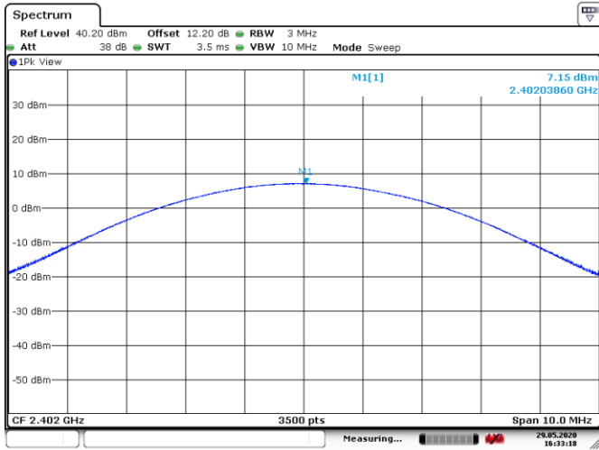
Figure 8.6-7: Output power on low channel, 8DPSK Modulation
