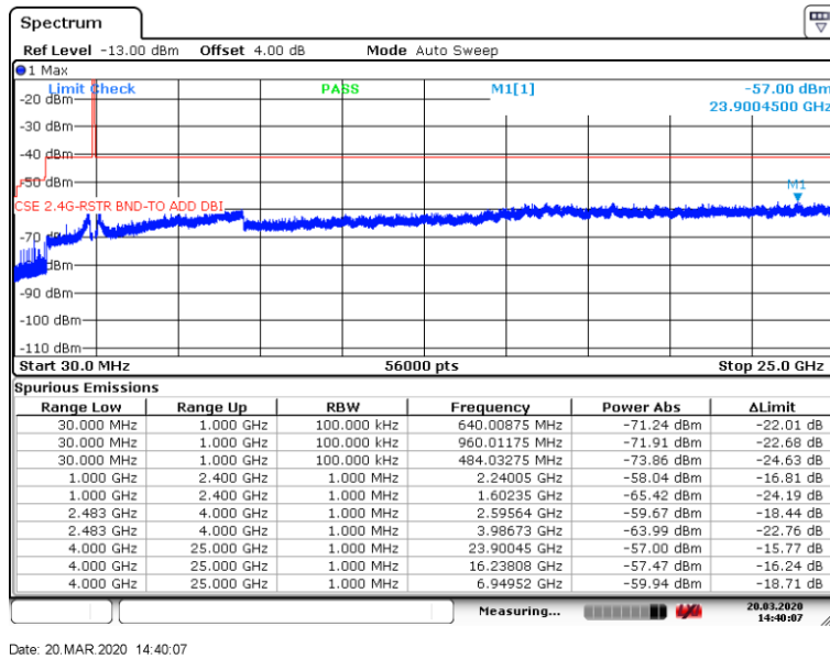
Figure 8.7-13: Conducted spurious emissions (Restricted band) for low channel
