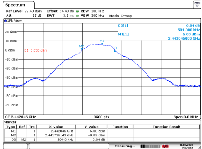
Figure 8.5-2: 6 dB bandwidth on mid channel, sample plot
