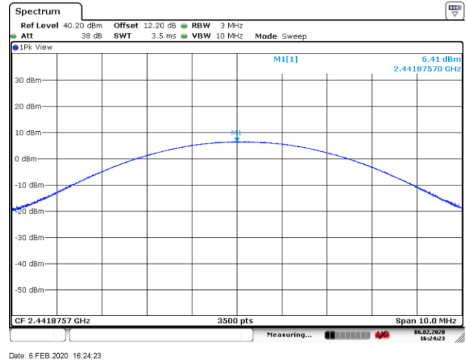
Figure 8.6-5: Output power on mid channel, pi/4-DPSK Modulation
