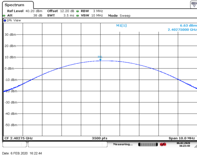
Figure 8.6-4: Output power on low channel, pi/4-DPSK Modulation
