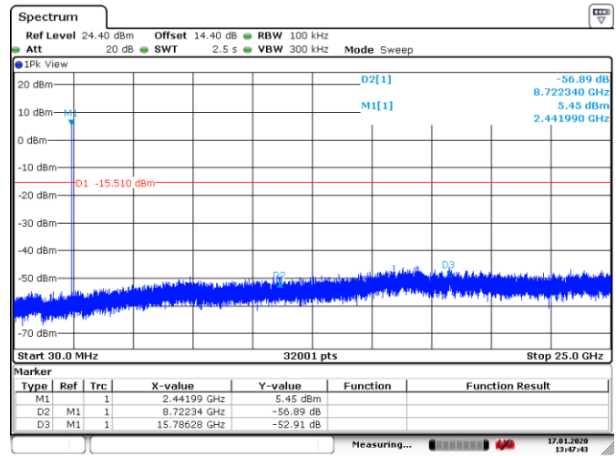
Figure 8.7-11: Conducted spurious emissions for mid channel, BLE
