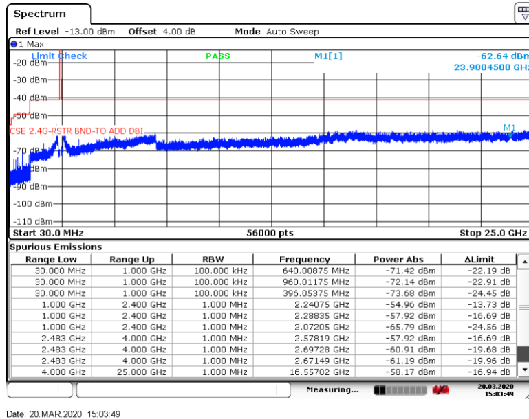
Figure 8.7-18: Conducted spurious emissions (Restricted band) for high channel
