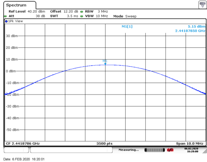
Figure 8.6-2: Output power on mid channel
