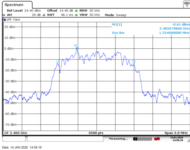
Figure 8.5-10: 99% occupied bandwidth on low channel
