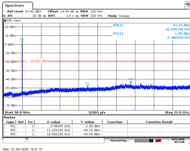
Figure 8.7-9: Conducted spurious emissions for high channel
