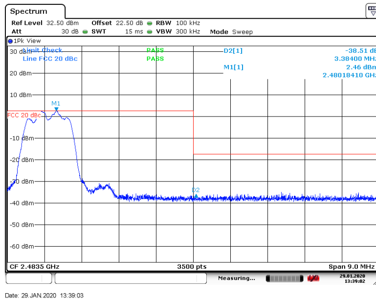
Figure 8.7-30: Band Edge emissions for high channel
