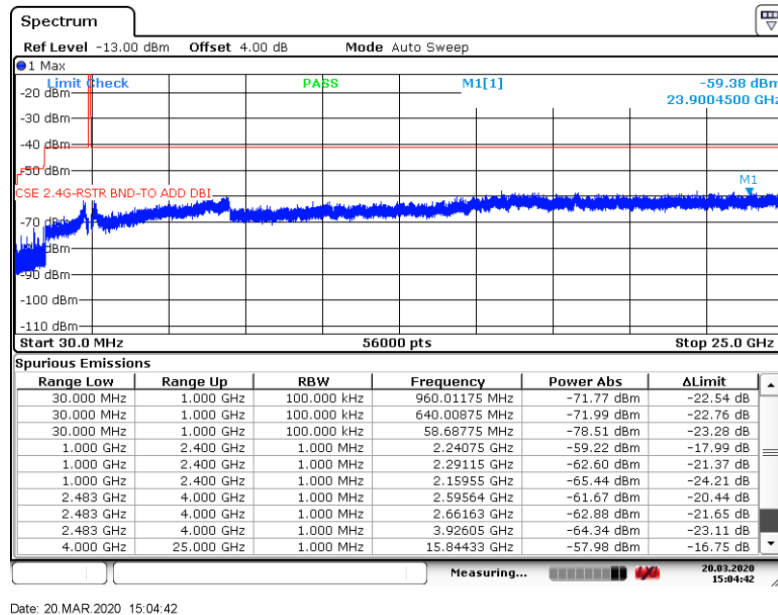
Figure 8.7-19: Conducted spurious emissions (Restricted band) for low channel
