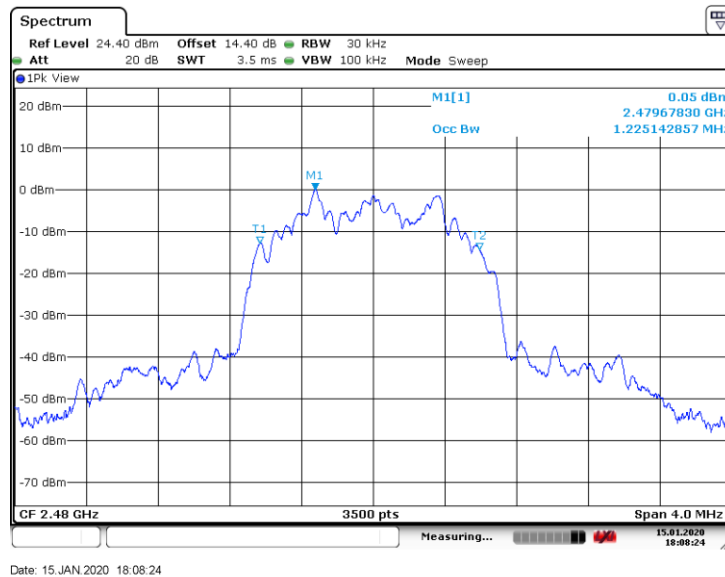
Figure 8.5-18: 99% occupied bandwidth on high channel, plot
