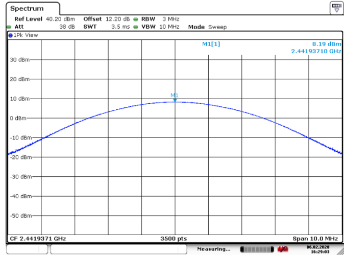
Figure 8.6-8: Output power on mid channel, 8DPSK Modulation
