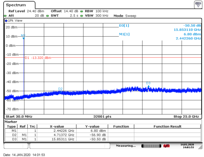
Figure 8.7-2: Conducted spurious emissions for mid channel
