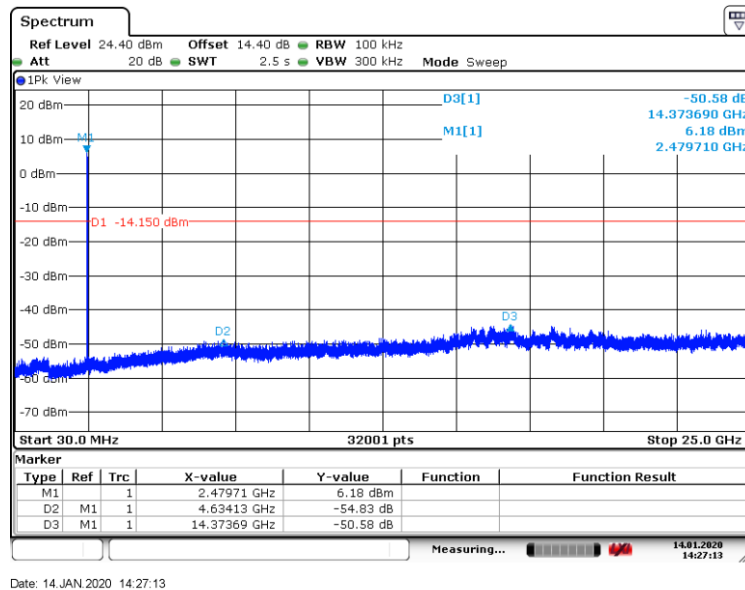
Figure 8.7-3: Conducted spurious emissions for high channel
