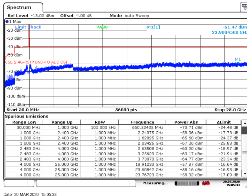
Figure 8.7-20: Conducted spurious emissions (Restricted band) for mid channel
