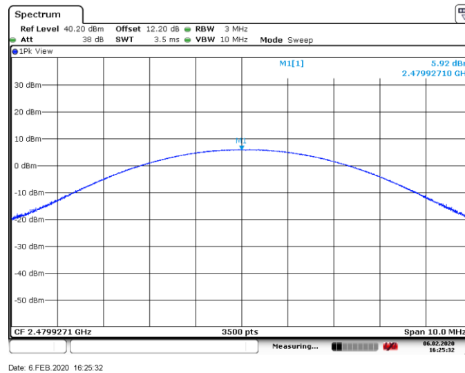
Figure 8.6-6: Output power on high channel, pi/4-DPSK Modulation
