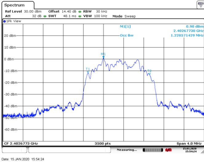
Figure 8.5-16: 99% occupied bandwidth on low channel, plot
