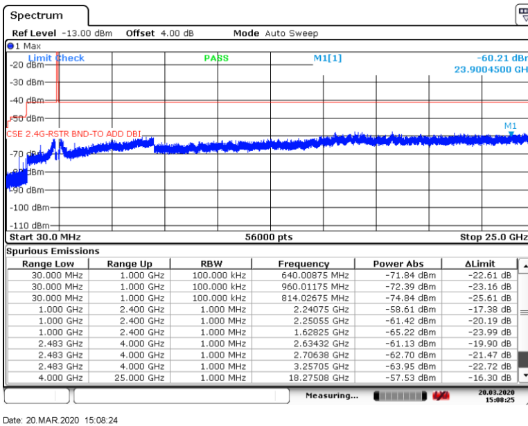
Figure 8.7-23: Conducted spurious emissions (Restricted band) for mid channel
