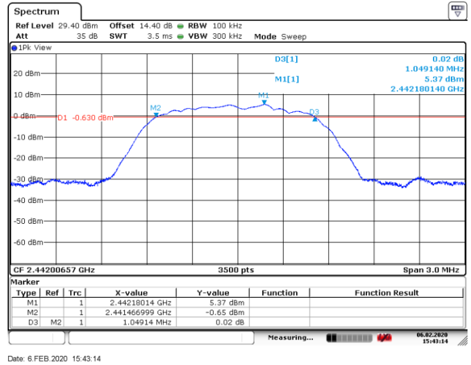
Figure 8.5-8: 6 dB bandwidth on mid channel
