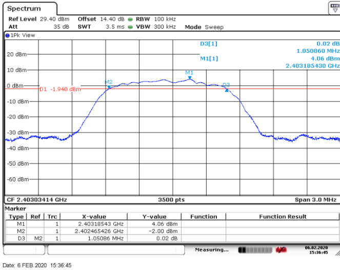
Figure 8.5-7: 6 dB bandwidth on low channel
