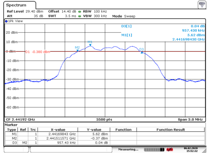
Figure 8.5-14: 6 dB bandwidth on mid channel, sample plot
