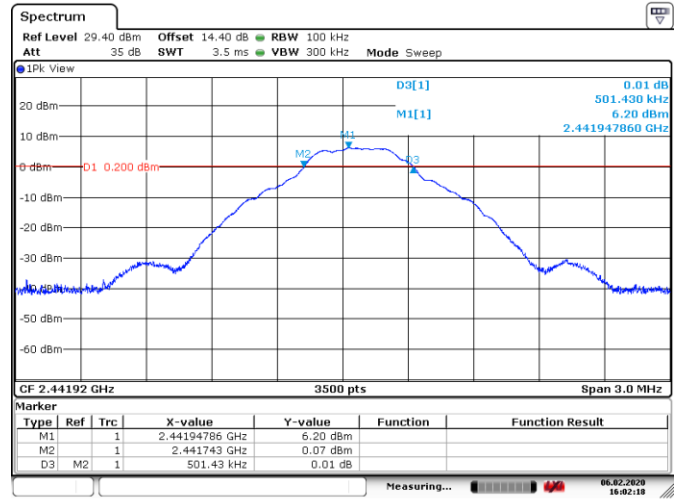
Figure 8.5-20: 6 dB bandwidth on mid channel, plot
