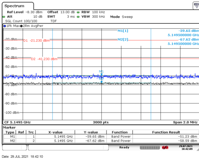
Figure 8.8-12: Lower band edge, Tx on low channel, 802.11n HT20/802.11ac VHT20
