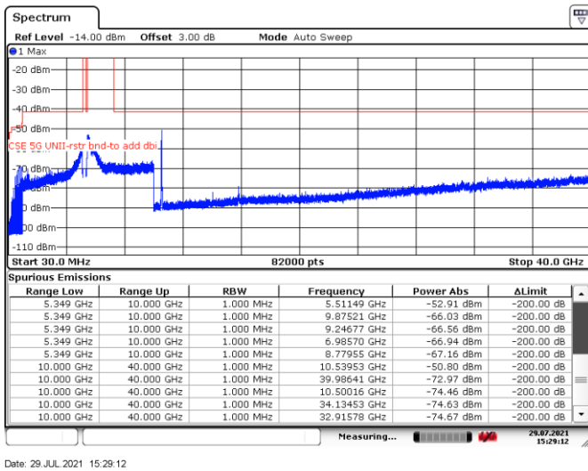
Figure 8.8-24: Spurious emissions within restricted bands, Tx on low channel, 802.11n HT40/802.11ac VHT40
