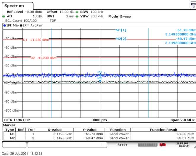
Figure 8.8-10: Lower band edge, Tx on low channel, 802.11a
